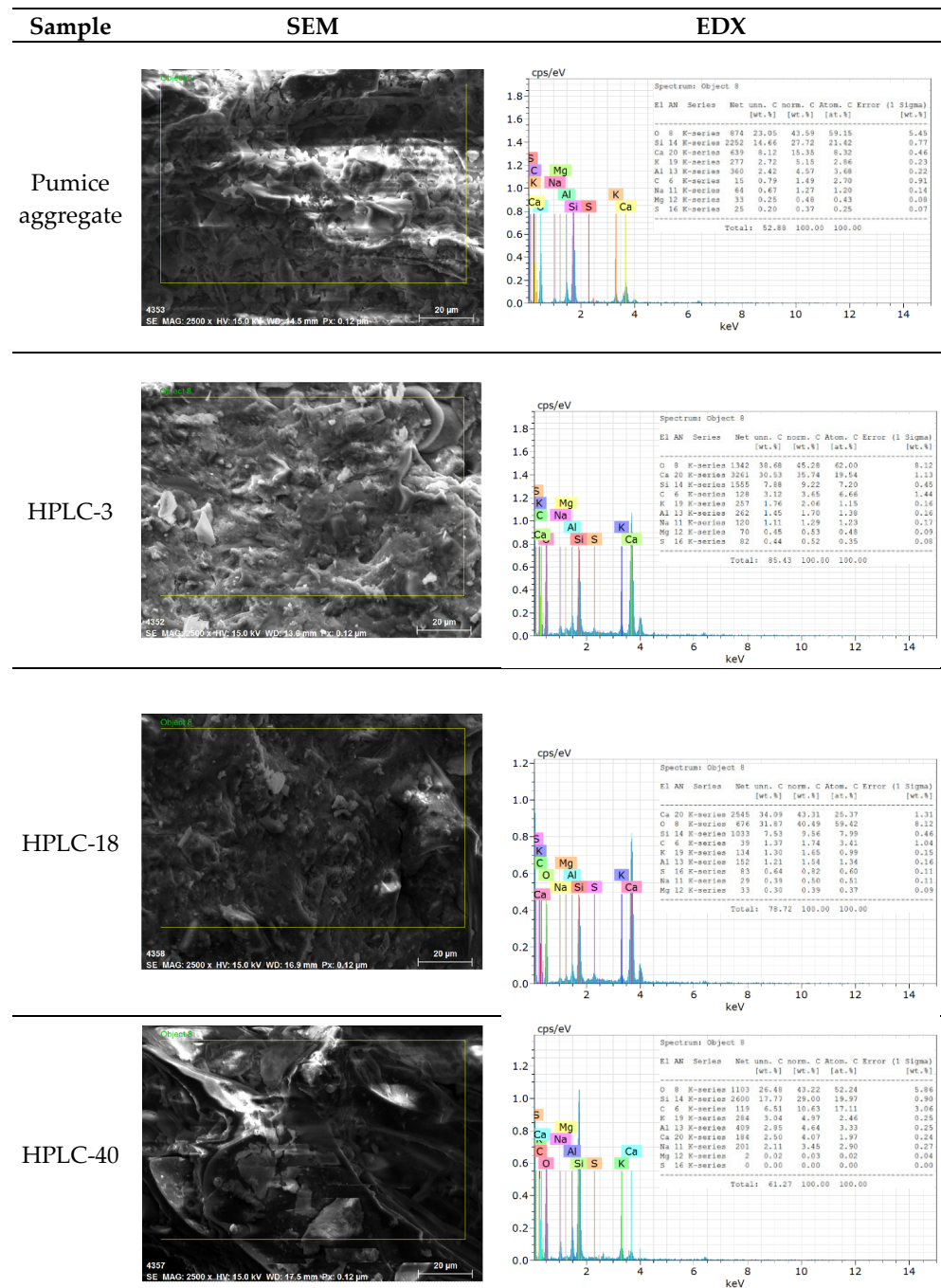
Figure 3. EDX analysis and SEM images of the pumice aggregate tested in the current study and selected HPLC samples ( the yellow frame indicates the specific region focused for microstructural/EDX analysis ).
