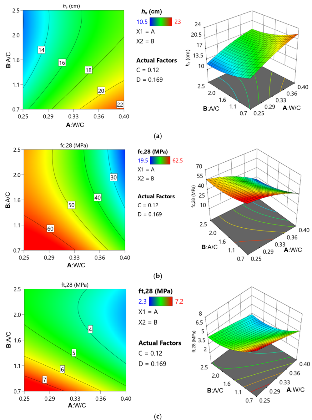
Figure 10. The effect of A/C and W/C on fresh and hardened concrete properties by Response Surface Method: (a) slump value, (b) compressive strength, (c) splitting tensile strength.
