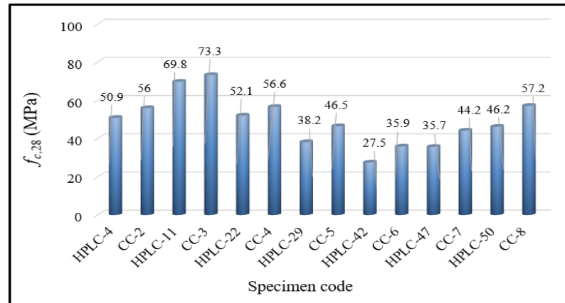
Figure 5. Comparison of 28-day compressive strengths of HPLC and CC samples.
