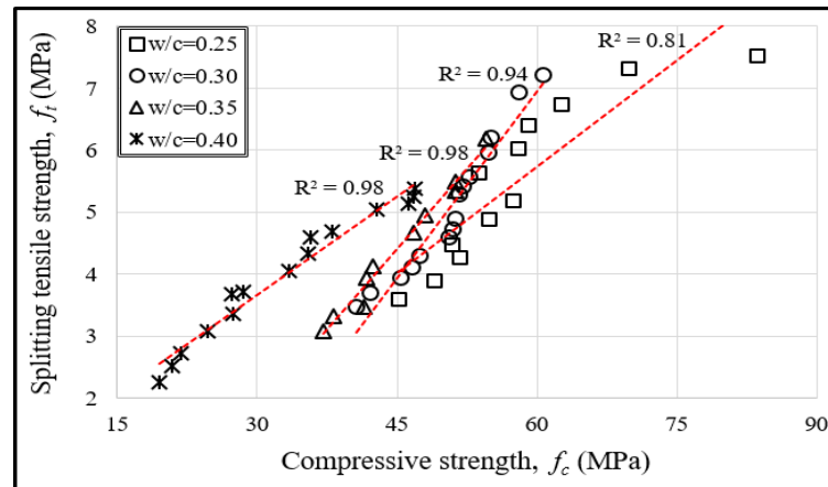
Figure 8. Comparison of 28-day splitting tensile strength with 28-day compressive strength.
