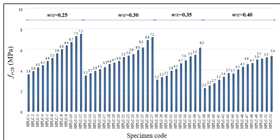
Figure 6. The 28-day average splitting tensile strength values of HPLC samples.
