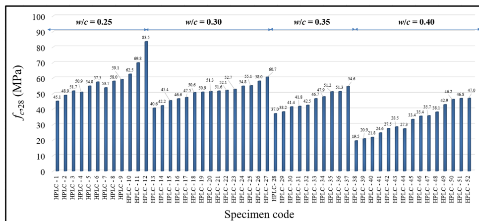
Figure 4. The 28-day average compressive strength values of HPLC samples.
