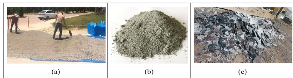
Figure 1. Materials used in HPLC production within the scope of the current study: (a) pumice aggregate, (b) silica fume, (c) waste marble aggregate.
