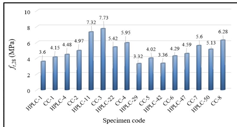
Figure 7. Comparison of HPLC and CC samples' 28-day splitting tensile strengths.
