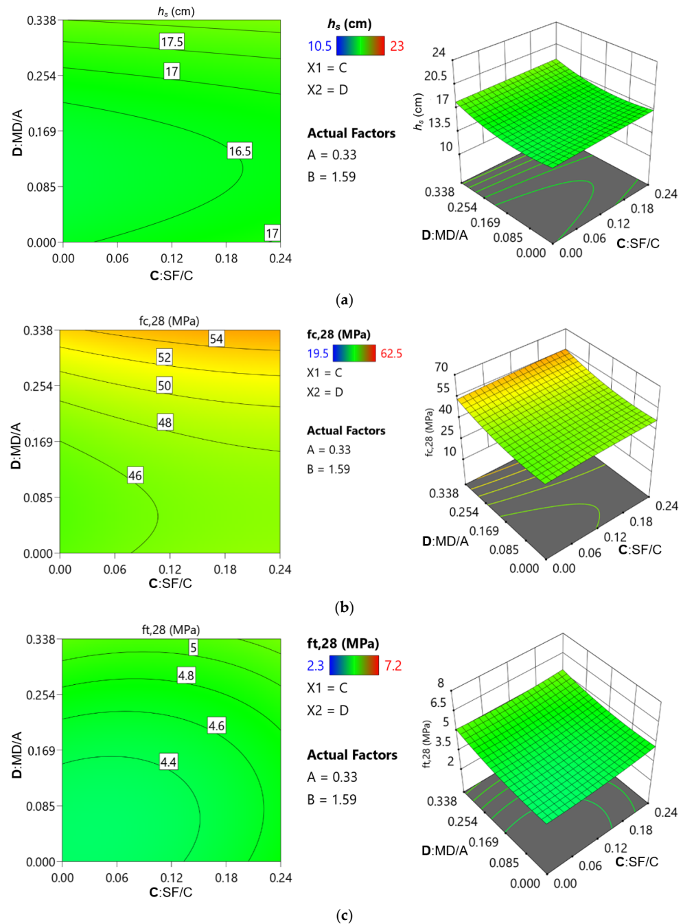
Figure 11. Effect of MD/A and SF/C on fresh and hardened concrete properties by the Response Surface Method: (a) slump value, (b) compressive strength, (c) splitting tensile strength.
