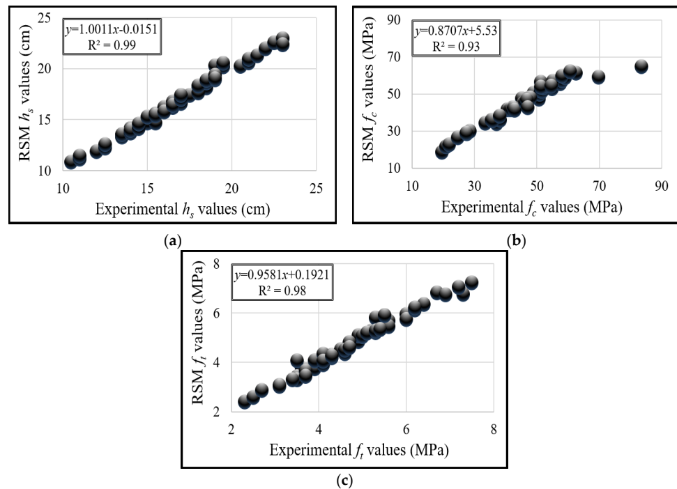
Figure 9. Comparison of the experimentally measured values with the values calculated by the RSM: (a) slump value ( h_s ), (b) compressive strength ( f_c ), (c) splitting tensile strength ( f_t ).
