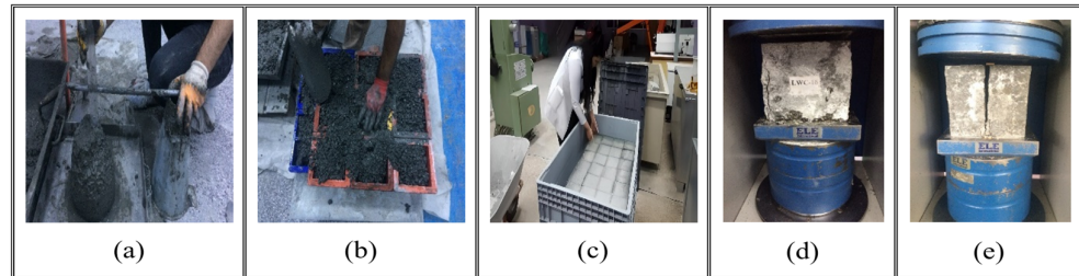
Figure 2. Performing the tests: (a) slump test, (b) fresh concrete placed in cube molds, (c) samples left in the curing pool, (d) compressive strength test for the hardened sample, (e) splitting tensile strength test for the hardened sample.
