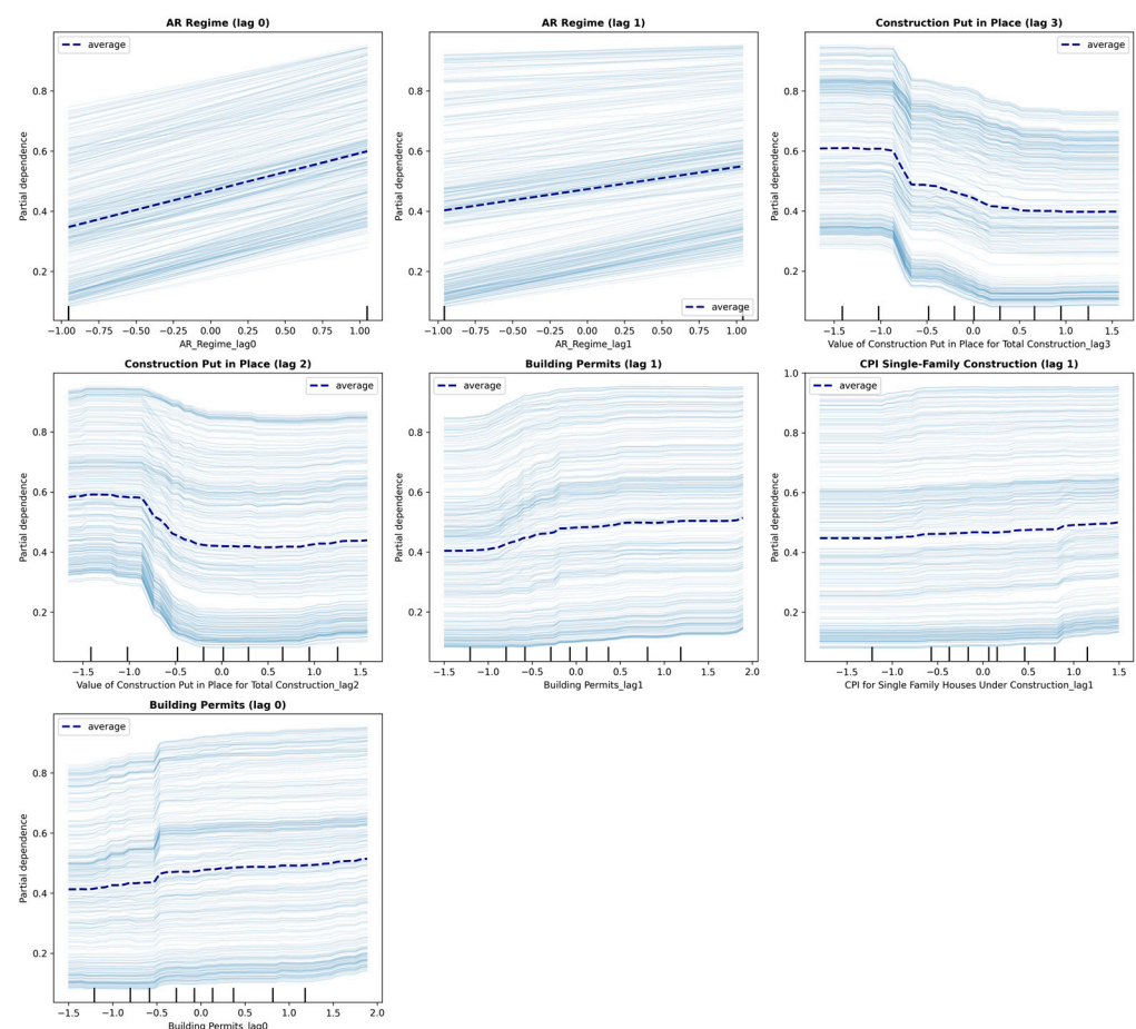
Figure 6. Partial Dependence and ICE Curves for All Seven Selected Predictors.
