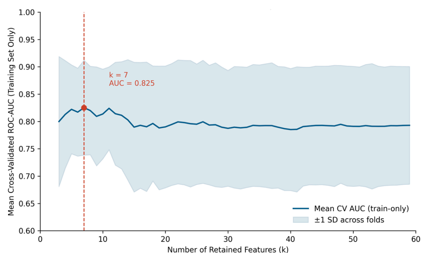
Figure 3. Cross-Validated ROC-AUC by Number of Retained Features.
