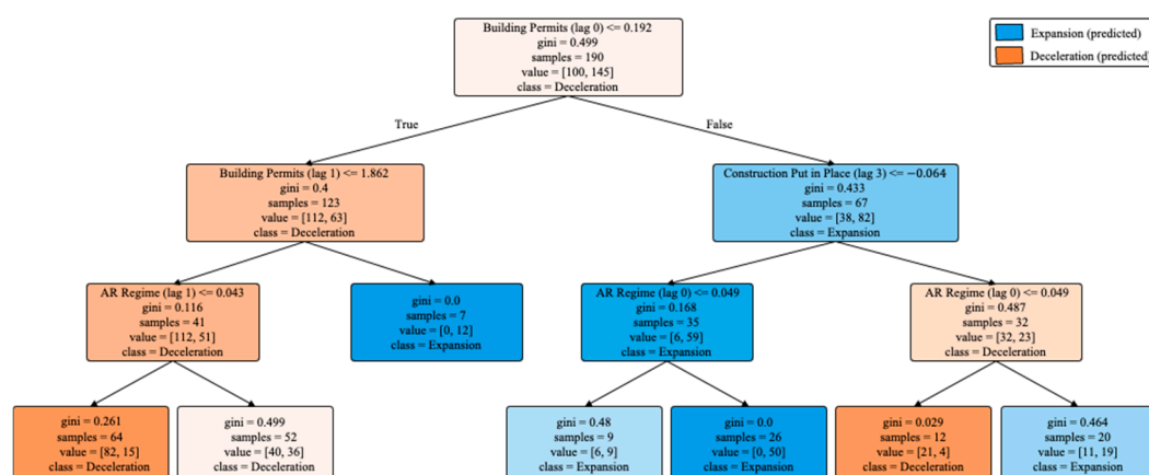
Figure 4. Example Decision Tree Classifier (Maximum Depth = 3).
