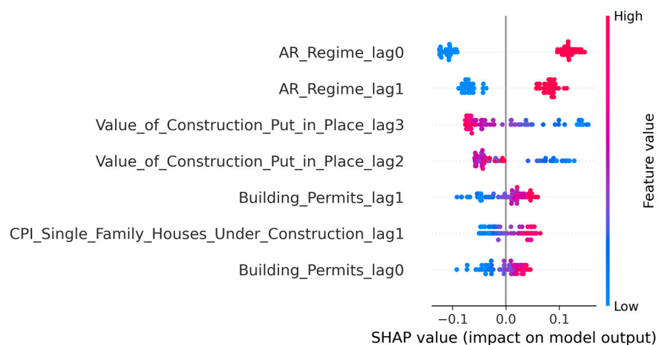
Figure 5. SHAP Beeswarm Plot for Random Forest Expansion and Deceleration Regime Classification.
