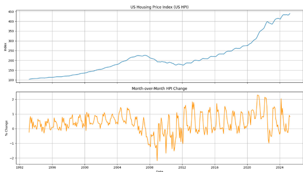
Figure 2. U.S. Housing Price Index and Month-over-Month Percentage Change (January 1993–March 2025).
