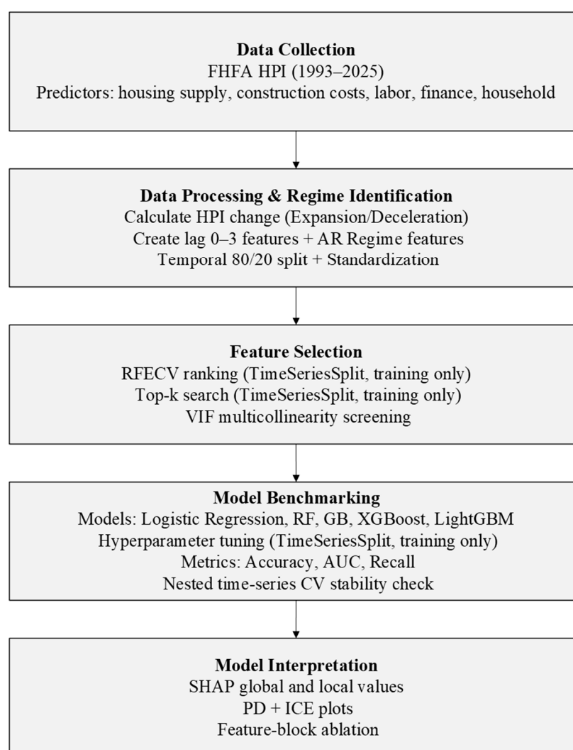
Figure 1. Flowchart of Research Methodology.
