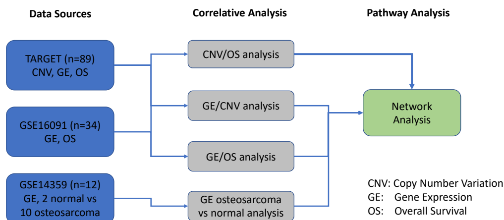
Figure 10. Schematic overview of the datasets and bioinformatics analyses conducted in the study.
