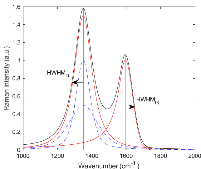
Figure 1. Typical Raman spectrum (black line) for a disordered carbon showing the principle of hand-made measurement of the half width at half maximum ( HWHM ). HWHM_D ( HWHM_D ) is for the D band (G band respectively). The G and D band contributions are plotted in red. The dotted blue reports the D band decomposition in two Voigt sub-bands (same wavenumber).
