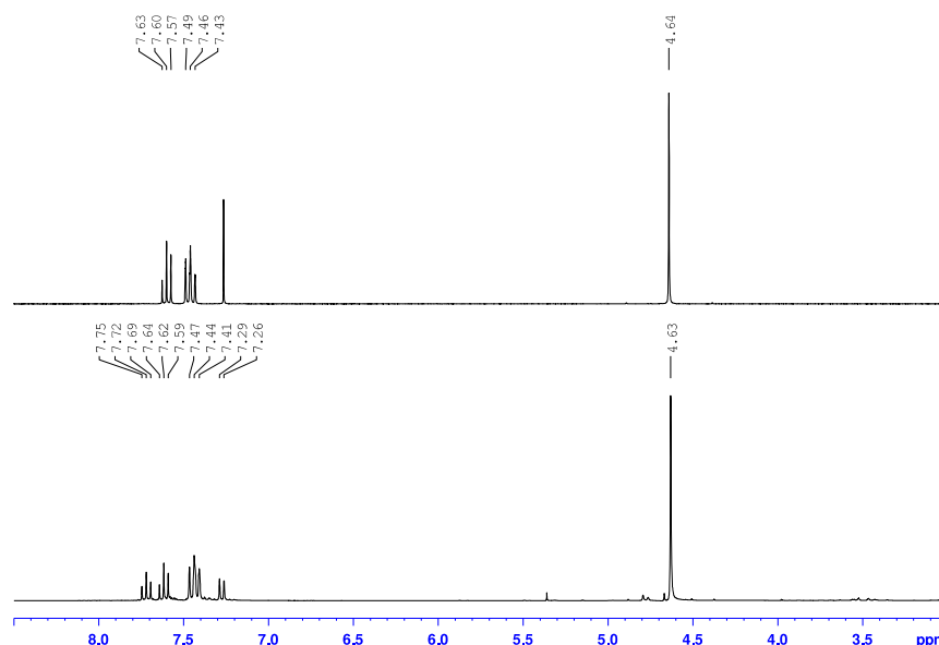
Figure 5. Overlay of the ^1\text{H} -NMR spectra for the product mixture from the reaction of 2-bromo-6-hydroxymethylpyridine with cyanuric chloride•DMF in DCM at r.t (top) and \text{SOCl}_2 at 40 °C (bottom) in \text{CDCl}_3 .
