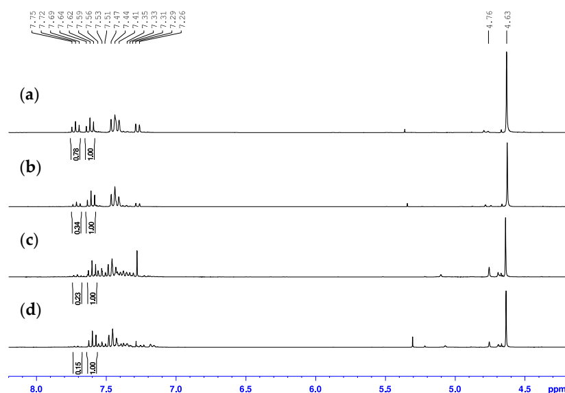
Figure 4. Overlay of the ^1\text{H-NMR} spectra for the product mixtures from the reaction of 2-bromo-6-hydroxymethylpyridine with \text{SOCl}_2 (a) neat at 40\text{ }^\circ\text{C} , (b) neat at r.t., (c) neat at 0\text{ }^\circ\text{C} , (d) in DCM at 0\text{ }^\circ\text{C} in \text{CDCl}_3 .
