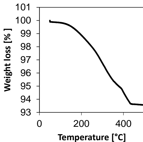
Figure S1. TG curve for centrifuged and dried PdNPs/4MePy (obtained in water).
