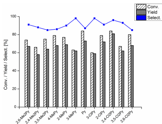
Figure S2. Effect of derivatives of pyridine on the conversion (Conv.), yield and selectivity (Select.) of the catalyst. Reaction conditions: 54 mmol AN, PdCl 2 (X n Py) 2 /Fe/I 2 = 0.056/2.68/0.118 mmol, 15 atm CO, 19 atm CO 2 , 6 atm O 2 , 20 ml EtOH, 100°C, 60 min.
