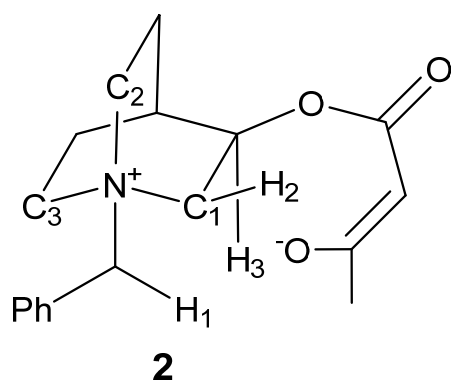
Figure 6. Selected ^1\text{H} and ^{13}\text{C} NMR signals for 2 assigned via HMBC and HSQC.
