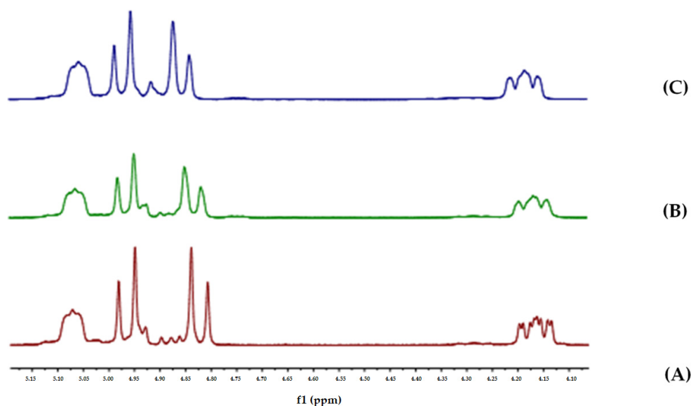
Figure 5. Selected ^1\text{H} -NMR spectral region of compound 16 before and following the addition of base. (A) Compound 16 ; (B) compound 16 and 2 equiv. of proton sponge after 10 min; (C) compound 16 and 2 equiv. of proton sponge after 24 h.
