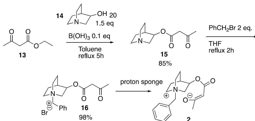
Scheme 2. Preparation of 2 .
