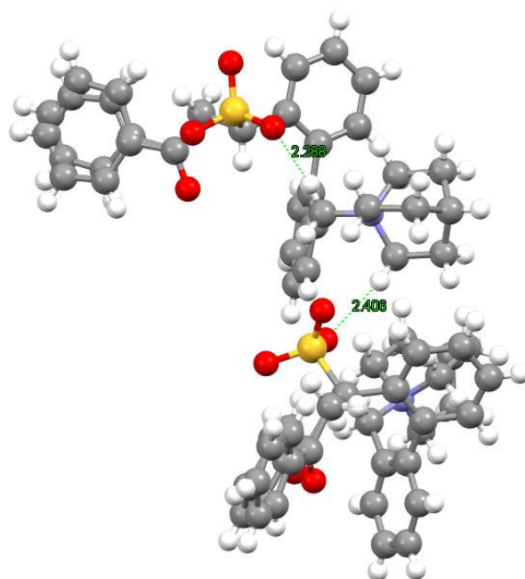
Figure 4. X-ray crystal structure of compound 1a .
