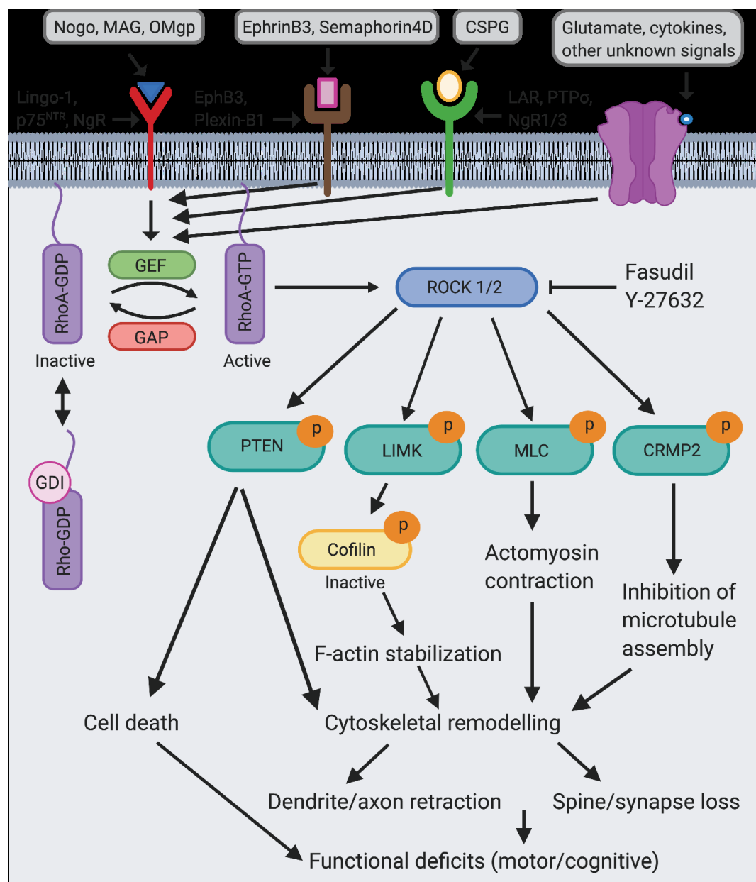
Figure 1. Model for the role of the RhoA-ROCK pathway in the pathogenesis of TBI. The small GTPase RhoA is activated by RhoA-GEFs in response to various extracellular signals triggered by injury. Active GTP-bound RhoA binds to and stimulates the activity of the serine/threonine kinase ROCK1/2. Through phosphorylation of downstream effectors such as PTEN, LIMK, MLC, and CRMP-2, ROCK initiates signaling cascades that induce cytoskeletal remodeling underlying dendrite/axon retraction and synapse/spine loss as well as cell death, which together contribute to functional deficits. Inhibition of ROCK (e.g., Fasudil, Y-27632) or RhoA rescues these TBI-induced deficits. ROCK: Rho Kinase, GEF: guanine nucleotide exchange factor, GAP: GTPase-activating protein, GDI: Guanine nucleotide dissociation inhibitor, PTEN: phosphatase and tensin homolog, LIMK: LIM kinase, MLC: myosin light chain, CRMP2: collapsin response mediator protein 2, MAG: myelin-associated glycoprotein, OMgp: oligodendrocyte-myelin glycoprotein, NgR: nogo receptor, PTP \sigma : protein tyrosine phosphate \sigma , NgR1/3: nogo receptor 1 and 3, LAR: leukocyte common antigen-related phosphatase, CSPG: chondroitin sulfate proteoglycans.
