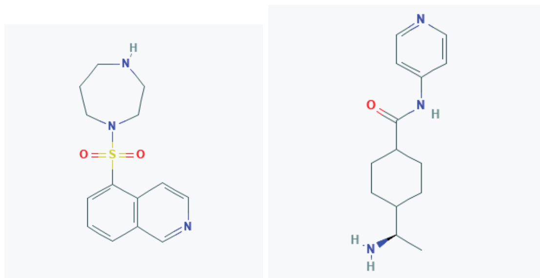
Figure 2. Pharmacological ROCK inhibitors Fasudil and Y-27632. Chemical structures of two widely used ROCK inhibitors, Fasudil and Y-27632. Both ROCK inhibitors have been demonstrated to alleviate functional deficits in mouse models of TBI. Images were taken from the National Center for Biotechnology Information, PubChem Database; Fasudil: https://pubchem.ncbi.nlm.nih.gov/compound/Fasudil ; Y-27632: https://pubchem.ncbi.nlm.nih.gov/compound/448042 .
