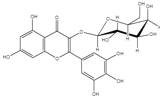
Figure 1. Chemical structure of M3G.
