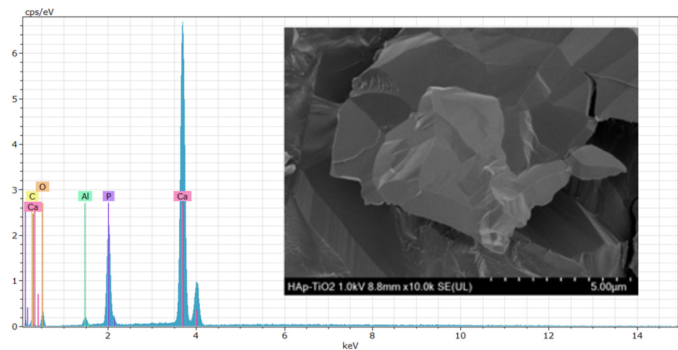
Figure 5. EDS spectra of HAp flakes.
