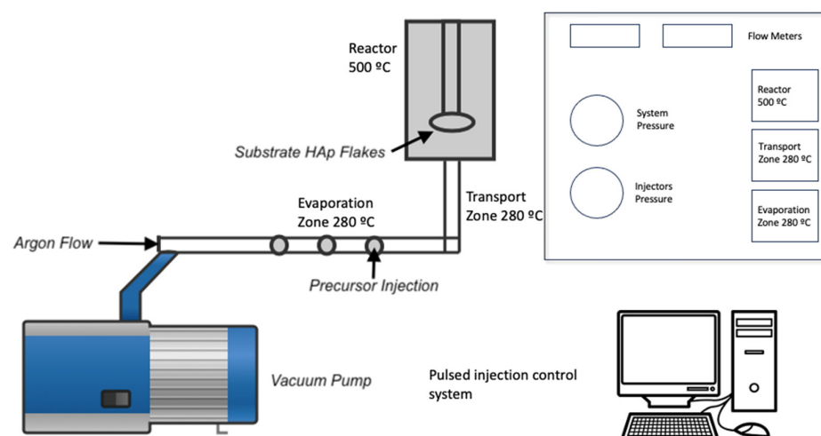
Figure 1. Schematic diagram to obtain \text{TiO}_2 coatings on hydroxyapatite flakes.
