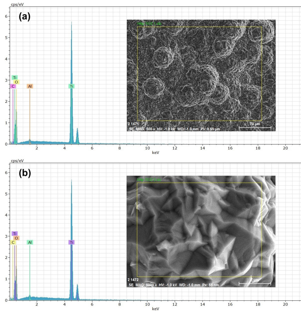
Figure 4. EDS spectra of \text{TiO}_2 coating: (a) micrograph at \times 500 ; (b) micrograph at \times 5000 .
