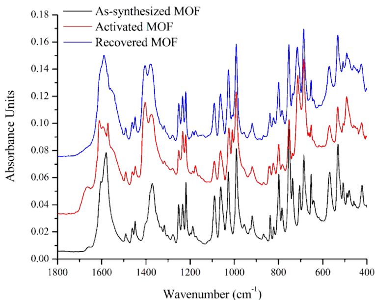
Figure 4. ATR-FTIR spectra of the as-synthesized MOF (black), the activated MOF (red), and the recovered MOF (blue).
