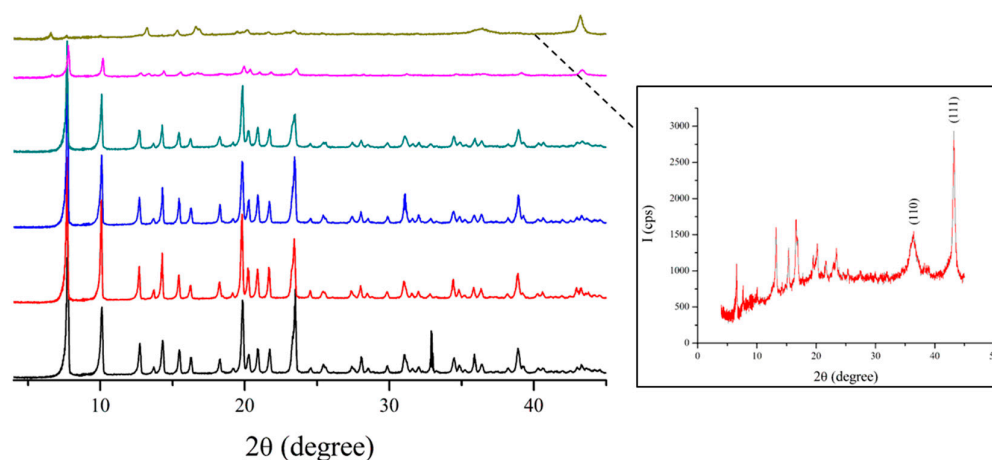
Figure 3. The in-situ PXRD analysis for the metal–organic framework (MOF). The sample has been treated at 100 °C for 2 h (red line), 120 °C for 2 h (blue line), 140 °C for 2 h (green line), 160 °C for 2 h (pink line), and 180 °C for 2 h (yellow line). The black line corresponds to the simulated pattern.
