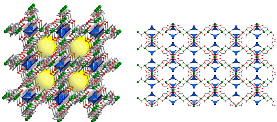
Figure 1. Perspective views of \infty^3[\text{Cu}_2(\text{mand})_2(\text{hmt})] (the hmt molecules are drawn in blue): the channels (yellow) hosting the water molecules, which are not shown ( left ); view along the crystallographic b axis emphasizing the hmt molecules (blue) each one with two uncoordinated nitrogen atoms ( right ).
