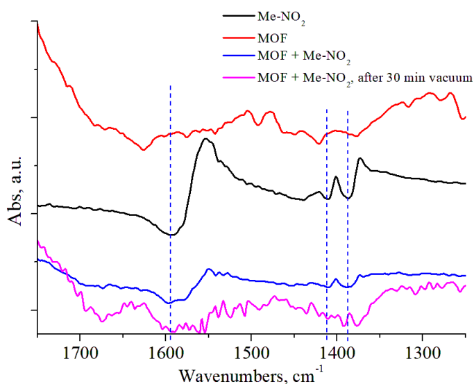
Figure 7. The diffuse reflectance infrared Fourier transform (DRIFT) spectra recorded for the nitromethane reference (black), the activated MOF (red), MOF washed by the substrate (blue), and MOF after 30 min evacuation (violet).
