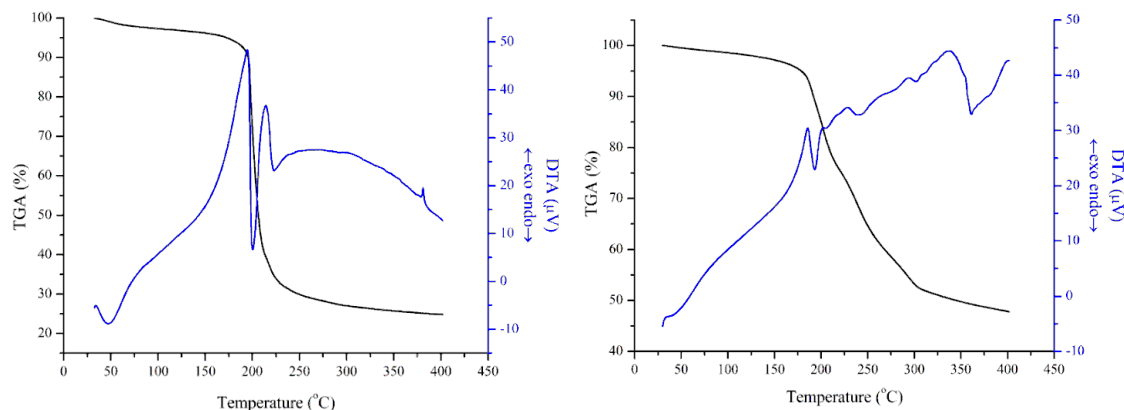
Figure 5. The TG–DTA profiles for the as-synthesized MOF ( left ) and the activated MOF ( right ).
