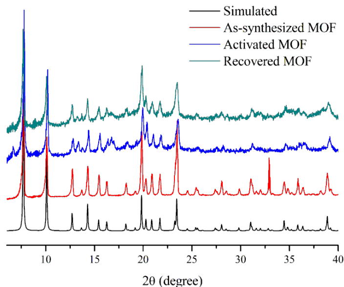
Figure 2. The XRD powder patterns for the simulated, as synthesized, activated, and recovered MOF.
