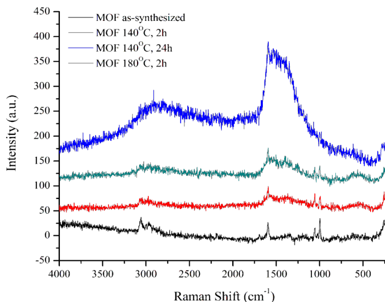
Figure 6. The Raman spectra recorded for MOF samples exposed to different thermal treatments.
