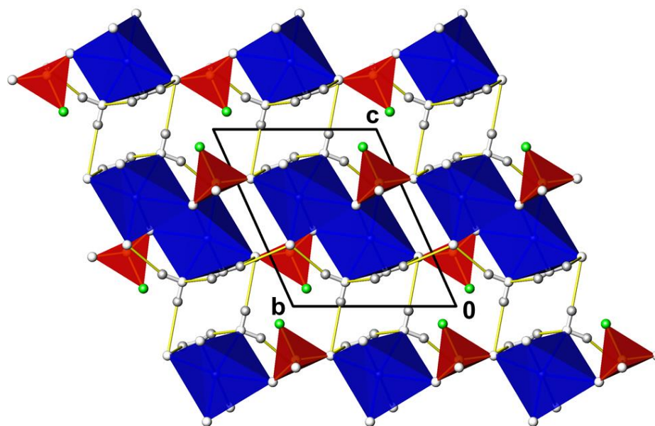
Figure 1. The crystal structure of \text{CdPO}_3\text{F}(\text{H}_2\text{O})_2 in a projection along [-100] . \text{PO}_3\text{F} tetrahedra are given in red (O atoms as colourless, F atoms as green spheres), [\text{CdO}_6] octahedra are given in blue, and H atoms are given as grey spheres. O–H...O hydrogen bonding is indicated by yellow lines.
