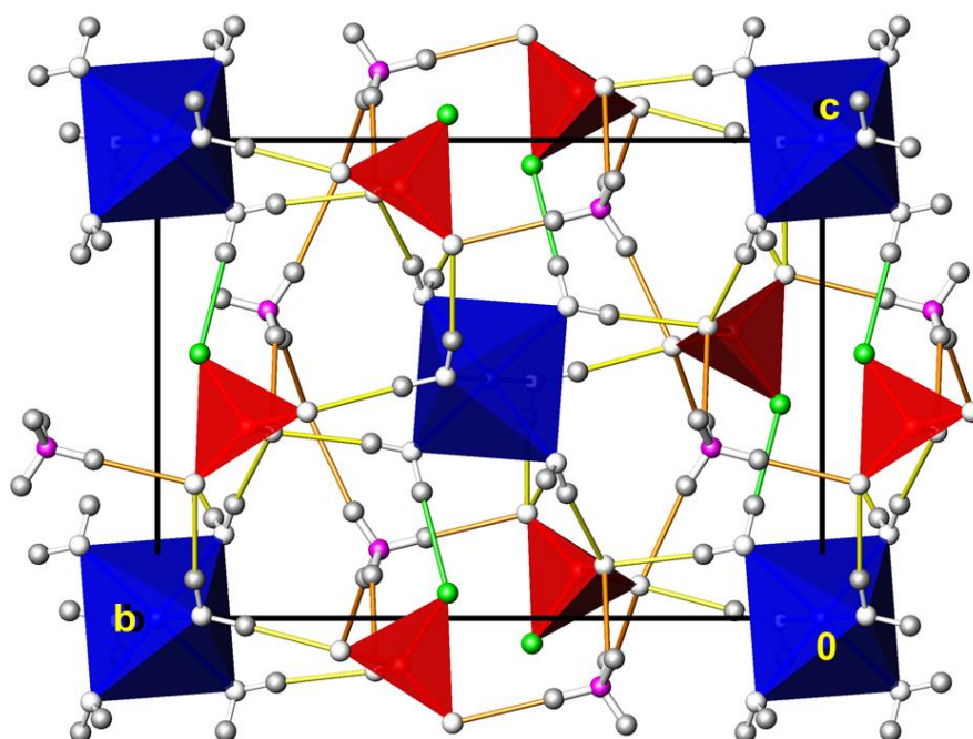
Figure 8. The crystal structure of (\text{NH}_4)_2\text{Ni}(\text{PO}_3\text{F})_2(\text{H}_2\text{O})_6 in a projection along [-100] . Colour code as in Figure 6; O–H...F hydrogen bonding is indicated by green lines.
