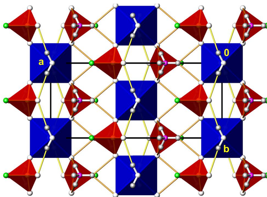
Figure 6. The crystal structure of (\text{NH}_4)_2\text{M}(\text{PO}_3\text{F})_2(\text{H}_2\text{O})_2 ( M = \text{Mg}, \text{Co} ; data used from the Mg-compound) in a projection along [001] . Colour code of \text{PO}_3\text{F} tetrahedra, H atoms and \text{O}-\text{H}\cdots\text{O} hydrogen bonding as in Figure 1; [\text{MO}_6] octahedra are given in blue, N atoms of the ammonium groups as magenta spheres. \text{N}-\text{H}\cdots\text{O} hydrogen bonding is indicated by orange lines.
