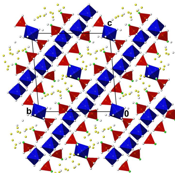
Figure 3. The crystal structure of \text{Cr}_2(\text{PO}_3\text{F})_3(\text{H}_2\text{O})_{18.8} in a projection along [-100] . Colour code of \text{PO}_3\text{F} tetrahedra as in Figure 1; [\text{CrO}_6] octahedra are given in blue, O atoms of crystal water molecules with full occupation are given as colourless spheres and those of disordered crystal water molecules as yellow spheres. For clarity, disorder of one of the \text{PO}_3\text{F} groups is not shown.
