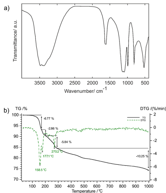
Figure 2. \text{CdPO}_3\text{F}(\text{H}_2\text{O})_2 . (a) IR spectrum; (b) TG curve (black) with its first derivative (DTG curve, green).
