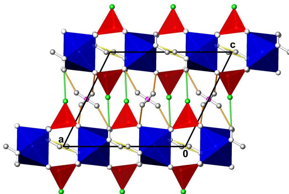
Figure 10. The crystal structure of \text{NH}_4\text{Cu}_2(\text{H}_3\text{O}_2)(\text{PO}_3\text{F})_2 in a projection along [010] . Colour code as in Figure 6.
