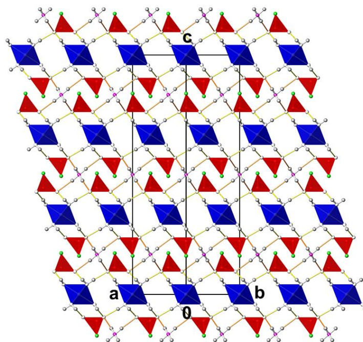
Figure 9. The crystal structure of \text{NH}_4\text{Cr}(\text{PO}_3\text{F})_2(\text{H}_2\text{O})_6 in a projection along [110] . Colour code as in Figure 6.
