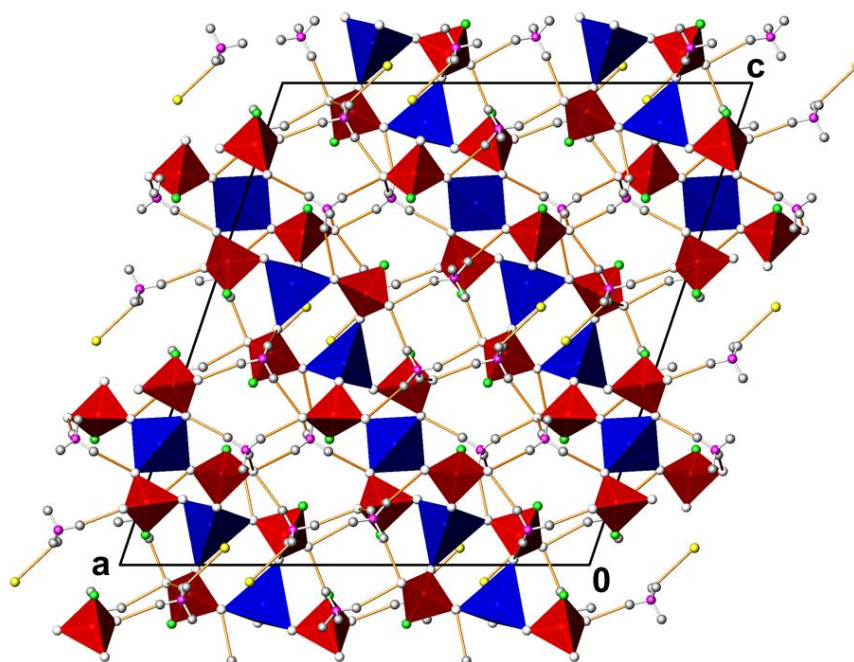
Figure 11. The crystal structure of (\text{NH}_4)_2\text{Zn}(\text{PO}_3\text{F})_2(\text{H}_2\text{O})_{0.2} in a projection along [010] . Colour code of \text{PO}_3\text{F} tetrahedra and H atoms as in Figure 1; O atoms of disordered crystal water molecules are given as yellow spheres. For clarity, disorder involving parts of the [\text{ZnO}_4] and \text{PO}_3\text{F} tetrahedra is not shown.
