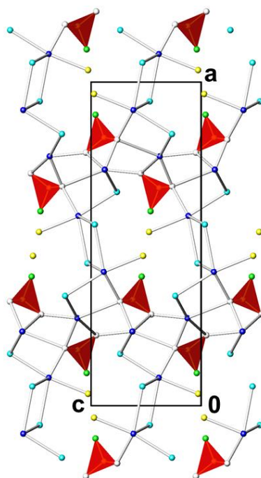
Figure 4. The crystal structure of \text{Pb}_2(\text{PO}_3\text{F})\text{Cl}_2(\text{H}_2\text{O}) in a projection along [0-10] . Colour code of \text{PO}_3\text{F} tetrahedra as in Figure 1; Pb atoms are represented by dark-blue spheres, Cl atoms as turquoise spheres and O atoms of the water molecules as yellow spheres.
