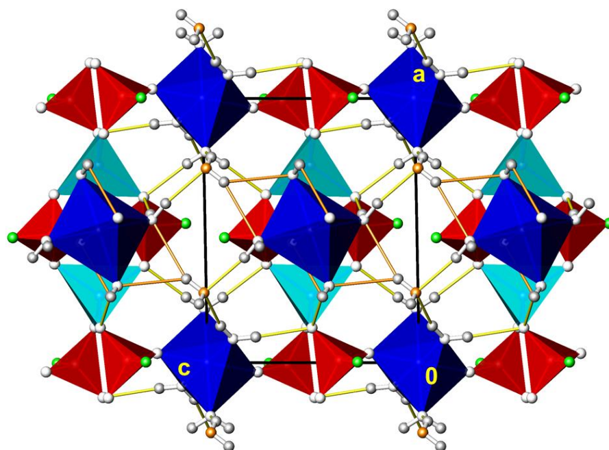
Figure 5. The crystal structure of \text{ZnPO}_3\text{F}(\text{H}_2\text{O})_{2.5} in a projection along [010] . Colour code of \text{PO}_3\text{F} tetrahedra and H atoms as in Figure 1; [\text{ZnO}_6] octahedra are given in dark-blue, [\text{ZnO}_4] tetrahedra in turquoise and the O atom of the crystal water molecule as an orange sphere. O–H...O hydrogen bonding with the aqua ligands as donor groups is given as yellow lines, and involving the crystal water molecules as donor groups as orange lines.
