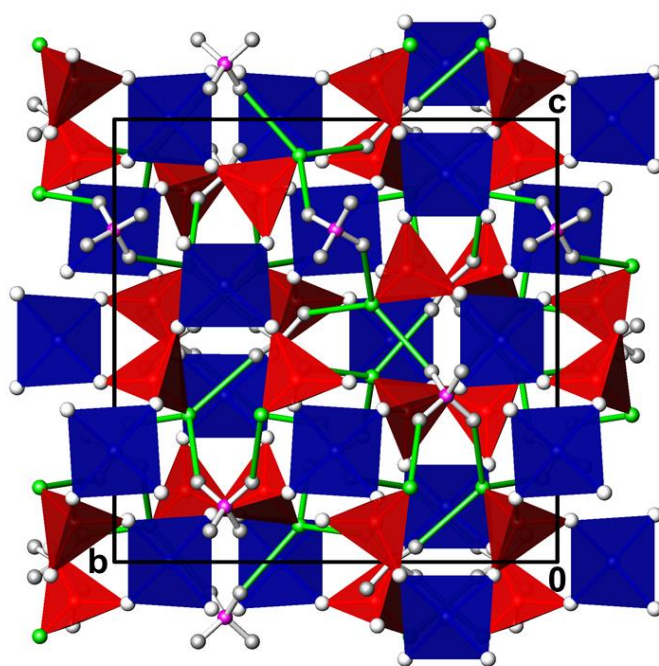
Figure 13. The crystal structure of (\text{NH}_4)_2\text{Zn}_3(\text{PO}_3\text{F})_4(\text{H}_2\text{O}) in a projection along [-100] giving only the major part of the disordered Zn site. Colour code of \text{PO}_3\text{F} tetrahedra as in Figure 1; [\text{ZnO}_4] tetrahedra are given in blue and (\text{N},\text{O})\text{--H}\cdots\text{F} hydrogen bonding is indicated by green lines. For clarity, (\text{N},\text{O})\text{--H}\cdots\text{O} hydrogen bonding is not shown.
