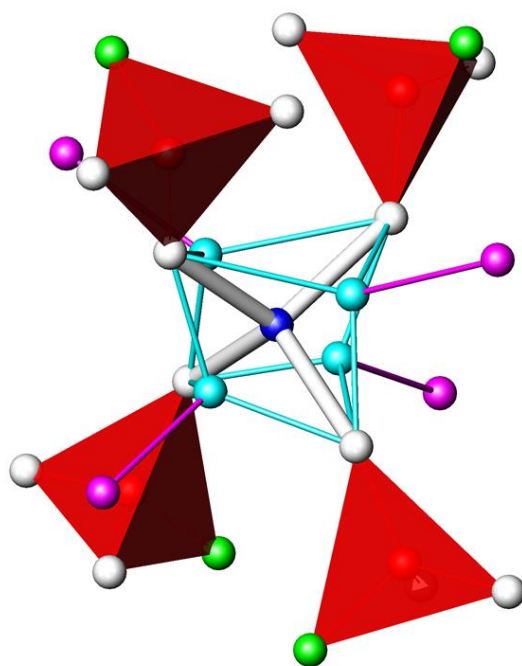
Figure 12. Disorder in the crystal structure of (\text{NH}_4)_2\text{Zn}_3(\text{PO}_3\text{F})_4(\text{H}_2\text{O}) . Colour code of the \text{PO}_3\text{F} tetrahedra as in Figure 1. The major part of the disordered Zn site (ZnA) is given as a blue sphere, the minor part (ZnB) as a turquoise sphere. The statistically occupied (\text{NH}_4/\text{H}_2\text{O}) site is given in magenta. For clarity, H atoms are not shown.
