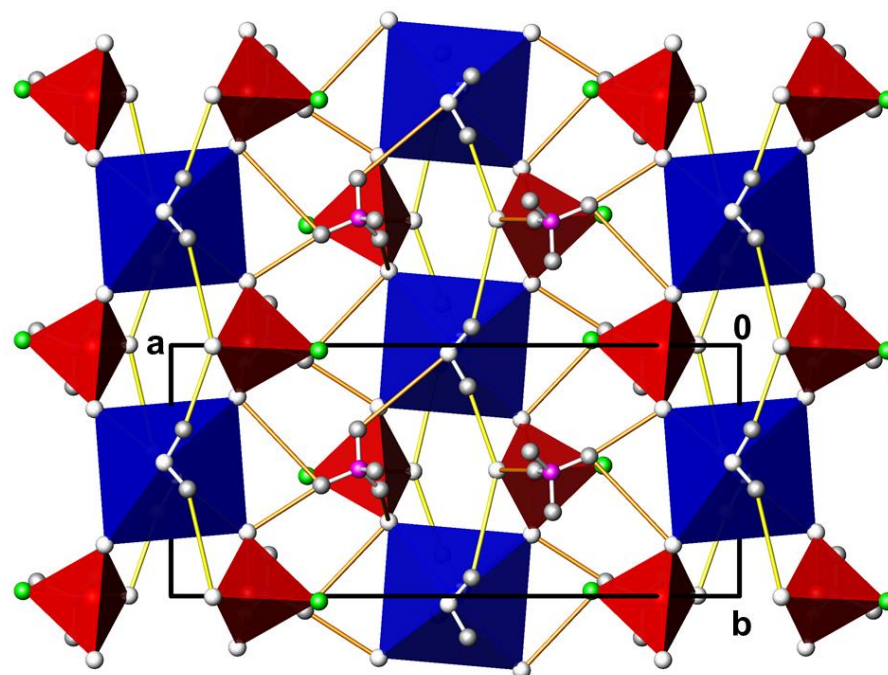
Figure 7. The crystal structure of (\text{NH}_4)_2\text{Mn}(\text{PO}_3\text{F})_2(\text{H}_2\text{O})_2 in a projection along [001] . Colour code as in Figure 6.
