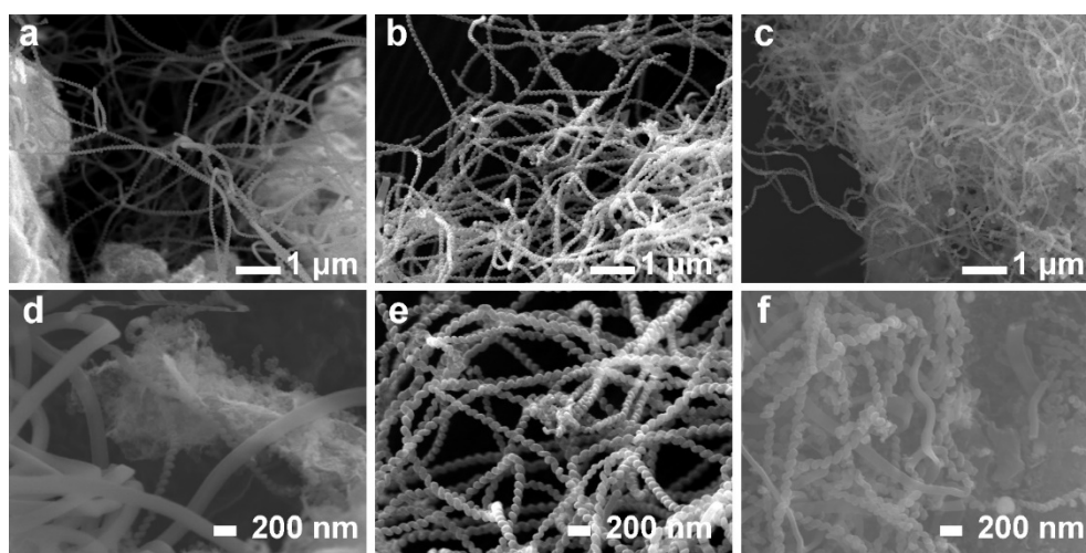
Figure 4. SEM images for CNCs. (a,d) CNCs synthesized by Cu100, (b,e) CNCs synthesized by Cu200, (c,f) CNCs synthesized by Cu 400.
