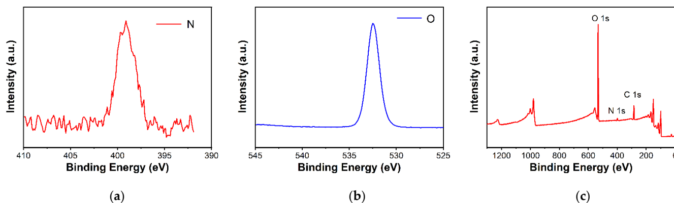
Figure 7. XPS spectra for 3-PANI-CNCs. (a) N 1s spectrum, (b) O 1s spectrum and (c) surface elements analysis spectrum.
