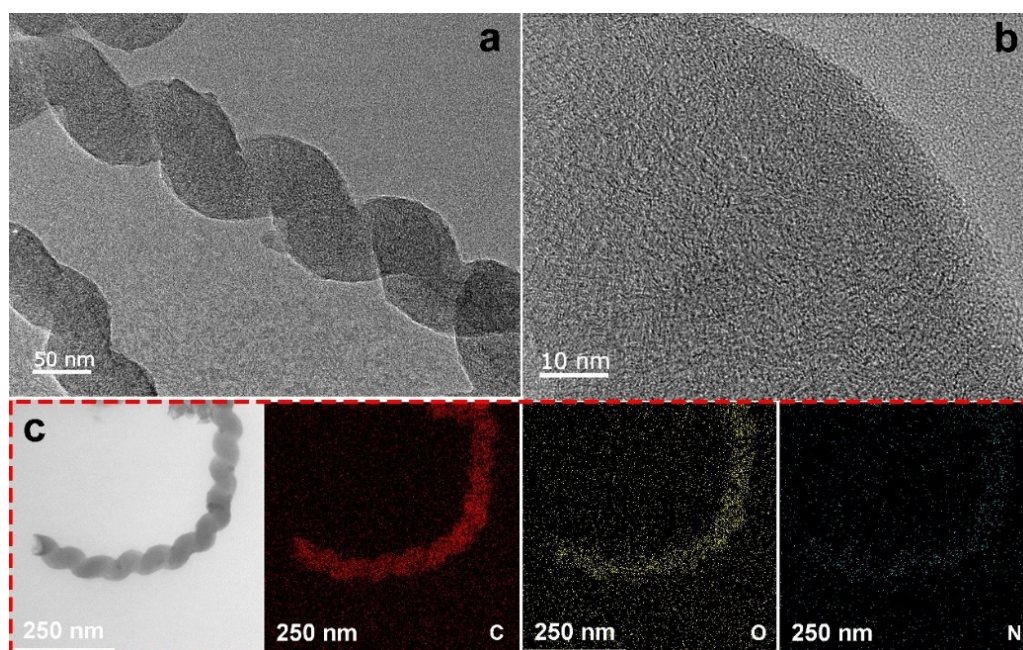
Figure 6. (a) TEM for PANI-CNCs, (b) HRTEM images for PANI-CNCs, (c) HAADF-STEM and EDS mapping for the PANI-CNCs.
