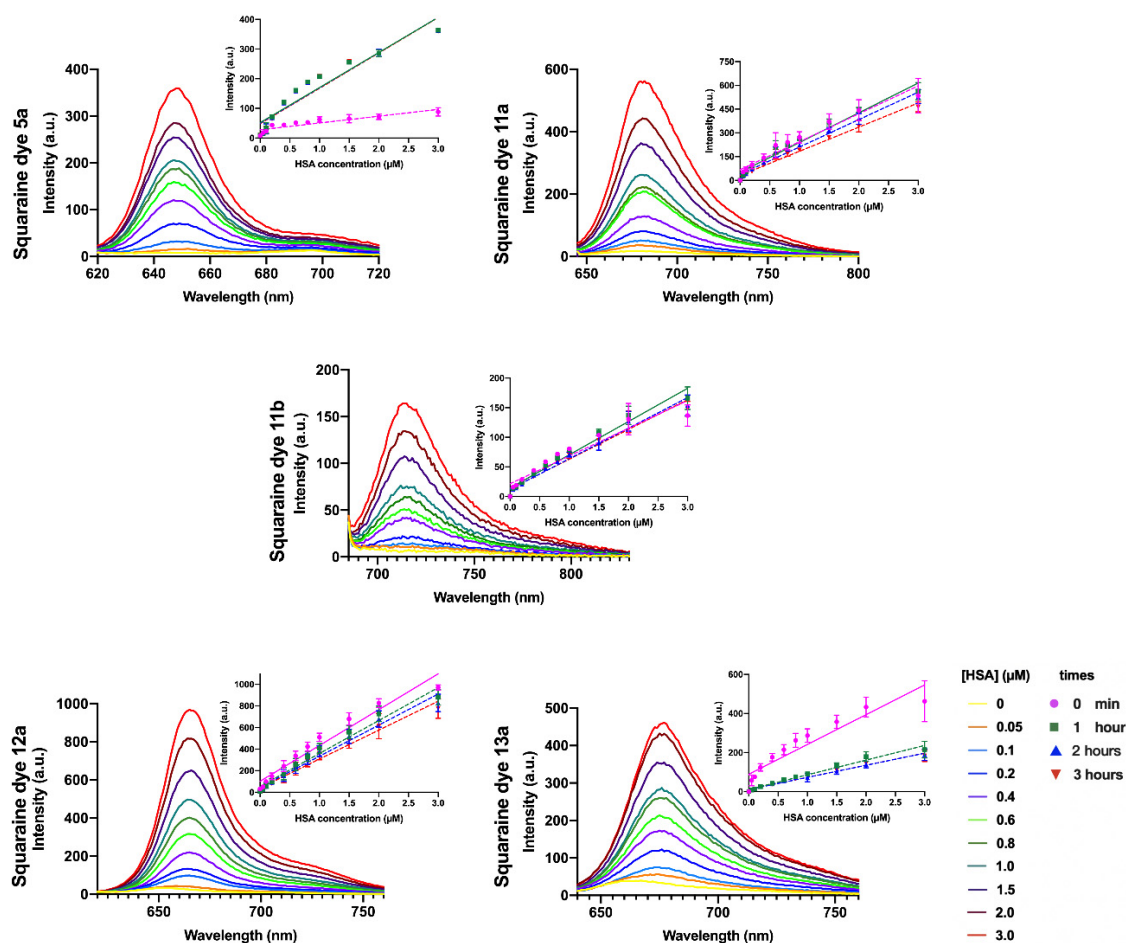
Figure 2. Fluorescence spectra of the squaraine dyes ( 5a , 11a,b , 12a , and 13a ) on phosphate buffer pH 7.4, with increasing concentrations of human serum albumin (0.00, 0.05, 0.10, 0.20, 0.40, 0.60, 0.80, 1.00, 1.50, 2.00 and 3.00 μM) and regression plots of the emitted fluorescence intensity as a function of protein concentration at various incubation times ( t = 0, 1, 2 and 3 h). Data on the plots are the mean \pm standard deviation of three independent assays. Spectra presented correspond to the time in which the dye exhibited more expressive fluorescence intensity in the shortest required time (full line). Fluorescence intensity is presented as arbitrary units (a.u.).
