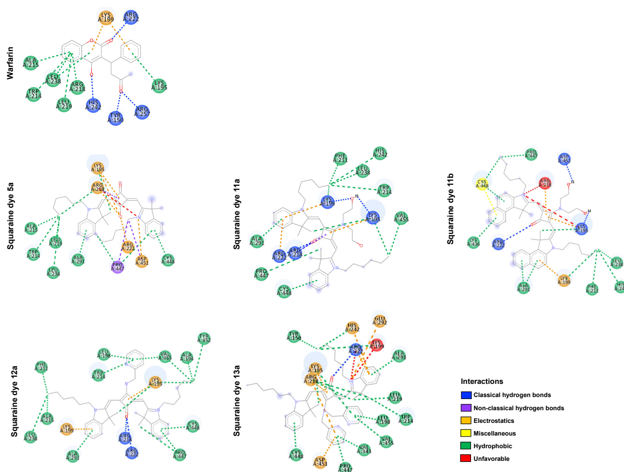
Figure 4. Binding modes and interactions of warfarin and squaraine dyes 5a , 11a , 11b , 12a , and 13a with amino acid residues of human serum albumin protein at Sudlow site I.
