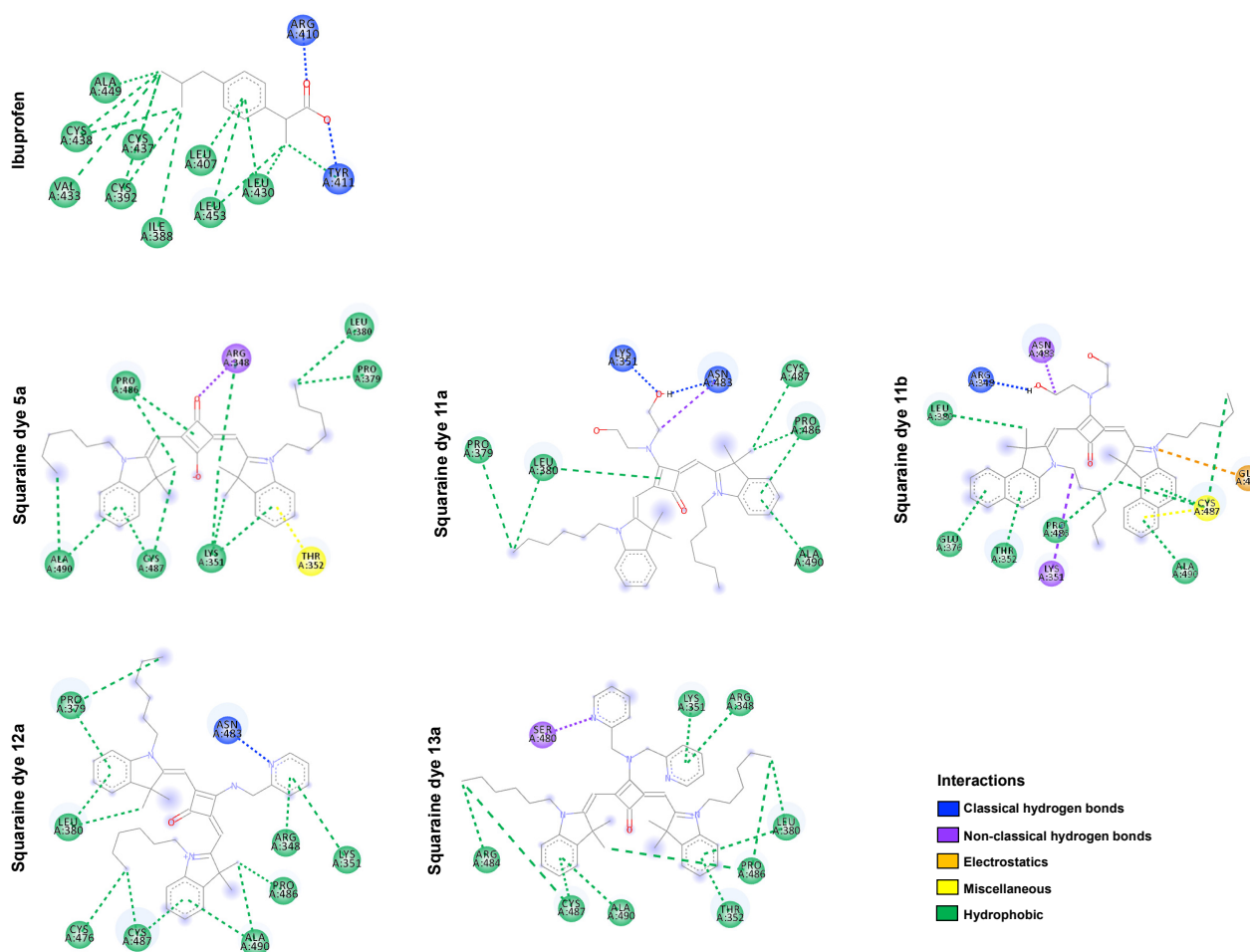
Figure 5. Binding modes and interactions of ibuprofen and squaraine dyes 5a , 11a,b , 12a , and 13a with amino acid residues of human serum albumin protein at Sudlow site II.
