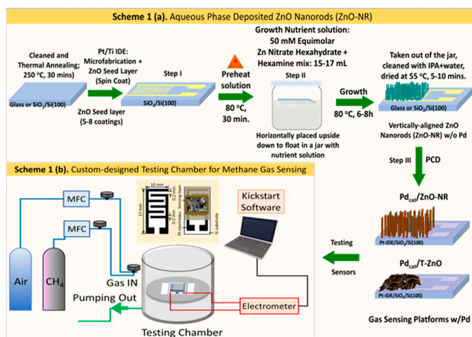
Scheme 1. (a) ZnO-NR synthesis (b) Custom-built testing system.
