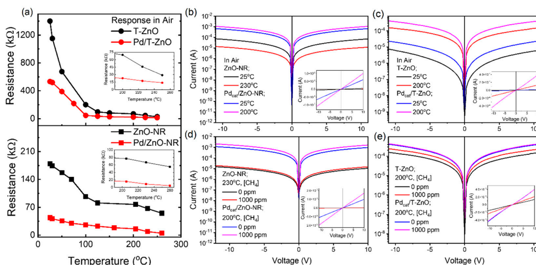
Figure 5. (a) Resistance response measured in air for ZnO-NR, Pd cat /ZnO-NR, T-ZnO, and Pd cat /T-ZnO, films; (b,c) I–V curves with temperature measured in air; (d,e) I–V curves at ~200 °C in air and 1000 ppm CH 4 .
