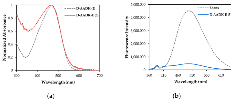
Figure 1. UV/Vis absorption and fluorescence spectroscopy: (a) normalized UV/Vis spectra of peptides 2–3 ( 1.0 \times 10^{-5} M) at pH 7.5 in phosphate buffer; (b) fluorescence spectra of free Edans and peptide probe 3 ( 1.0 \times 10^{-5} M) at pH 7.5 in phosphate buffer, upon excitation at 342 nm.
