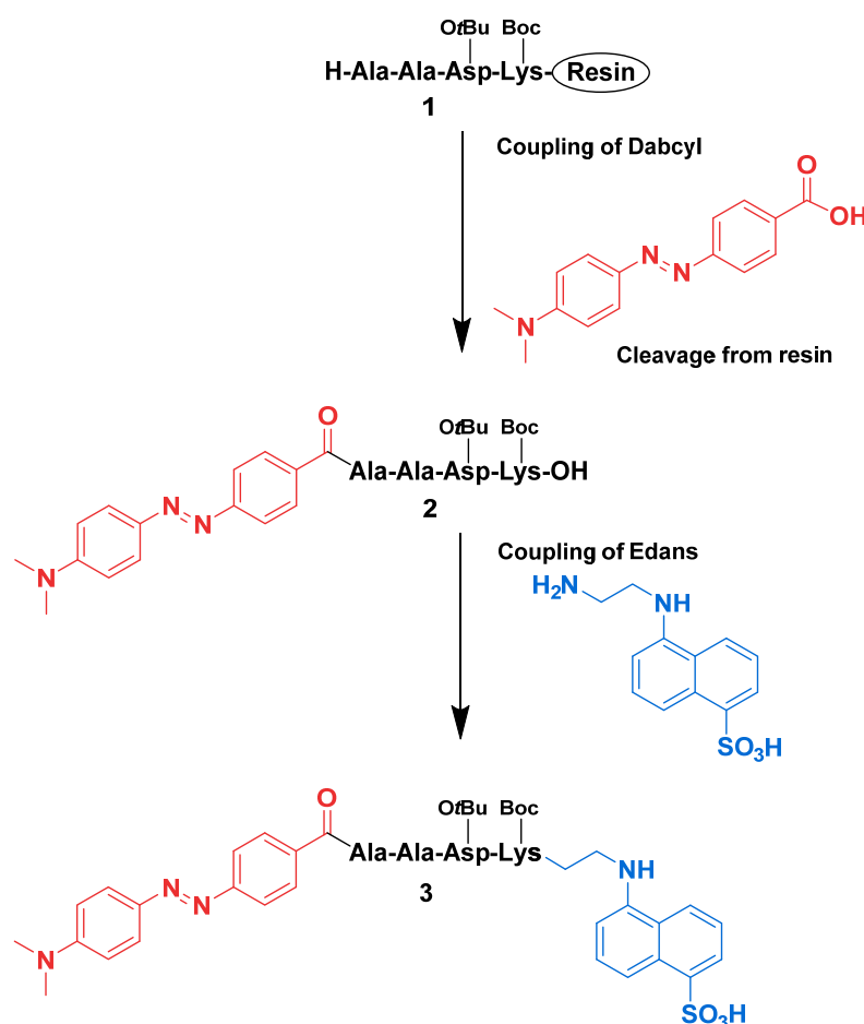
Scheme 1. Synthesis of Dabcyl-Ala-Ala-Asp(OtBu)-Lys(Boc)-Edans ( 3 ).
