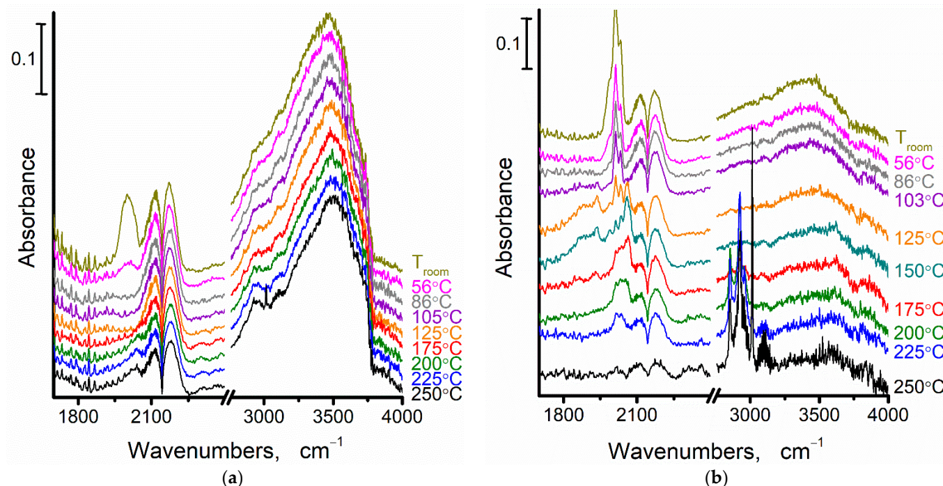
Figure 1. In situ DRIFTS spectra recorded at different temperatures during CO hydrogenation at 1 atm in the presence of: (a) CoPdA sample; (b) CoPdT sample.
