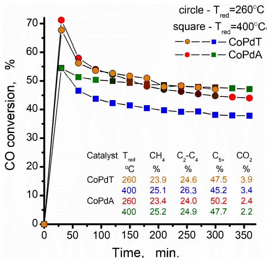
Figure 2. CO conversion at P = 10 atm over the studied samples after reduction at different temperatures. Inset: Product distribution.
