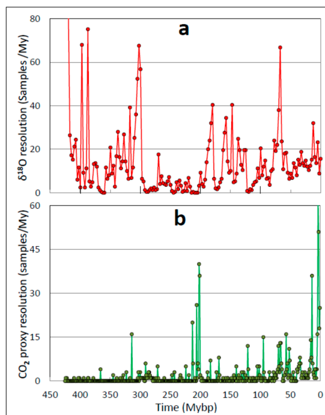
Figure 2. Sample resolution of climate proxies over the Phanerozoic Eon. Shown are sample datapoints per My for \delta^{18}\text{O} (a) and atmospheric \text{CO}_2 concentration (b). Zero values correspond to time periods in which no measurements are available.
