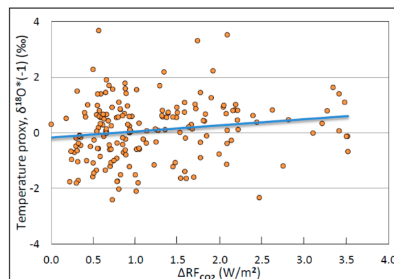
Figure 9. Scatter plot of detrended temperature-proxy data averaged in one-My bins from 425 to 0 My ago versus marginal RF by atmospheric CO 2 . The positive correlation coefficient ( R = 0.16 , n = 199 ) is discernibly different from zero ( p = 0.02 ) at this large sample size, but weak, i.e., as \Delta RF_{CO_2} increased, the temperature proxy \delta^{18}O^*(-1) increased only slightly. The trendline was fitted by the method of least squares.
