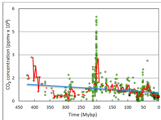
Figure 4. Atmospheric carbon dioxide ( \text{CO}_2 ) concentration proxies over the Phanerozoic Eon. Original raw data (green datapoints, n = 831 ) are from the database compiled by Royer [40]. The fitted red curve was computed as a 3–6 My moving average.
