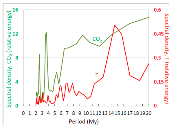
Figure 7. Spectral power periodograms of atmospheric \text{CO}_2 and temperature over the Phanerozoic Eon. The green and red curves show \text{CO}_2 and temperature spectral density profiles, respectively. The temperature periodogram was constructed using detrended temperature proxy data. Time periods covered and (in parentheses) Fisher's Kappa and the corresponding probability that the atmospheric \text{CO}_2 concentration and T periodograms result from white (Gaussian) noise are 85 to 0 My (12.57, 1.96 \times 10^{-5} ) and 522 to 0 My (28.98, 2.0 \times 10^{-13} ), respectively.
