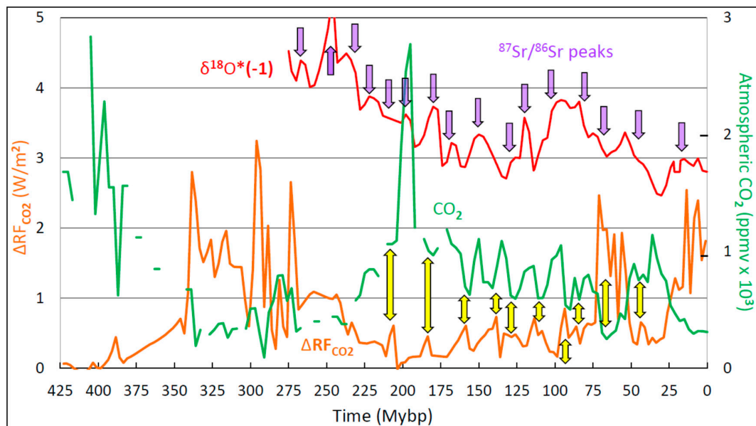
Figure 11. Time series of temperature proxies, atmospheric CO 2 concentration and \Delta RF_{CO_2} over the Phanerozoic Eon. Purple arrows correspond to peaks in the strontium ratio determined independently from visual inspection of time series in [28]. Temperature proxies (red curve) are from Prokoph et al. [28]. CO 2 proxies (green curve) are from Royer [40], represented here using a 3–6 My moving average. Yellow double-headed arrows highlight the expected antiphasic relationship between atmospheric CO 2 concentration and marginal forcing computed for tropical latitudes under clear-sky conditions. The scale for the temperature proxy is modified here by a constant offset for graphical presentation on the same scales as the other proxies. The correct temperature-proxy scale is shown in Figure 5. In this and following graphs, climate variables are color-coded: red represents the temperature proxy, \delta^{18}O^*(-1) ; green represents atmospheric CO 2 concentration proxies converted to ppmv; and orange represents the marginal forcing calculated for each atmospheric CO 2 concentration datapoint using the best-fit power function equation corresponding to the empirical curve for tropical latitudes under clear-sky conditions (Figure 8b).
