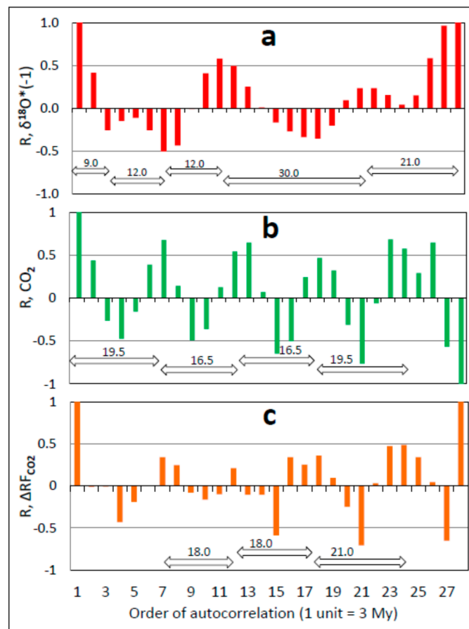
Figure 13. As in Figure 12, but over the shorter time period from 174 to 87 Mybp. Average cycle durations: (a) 16.8 My (b) 18.0 My (c) 19.0 My. Otherwise as in the legend of Figure 12.
