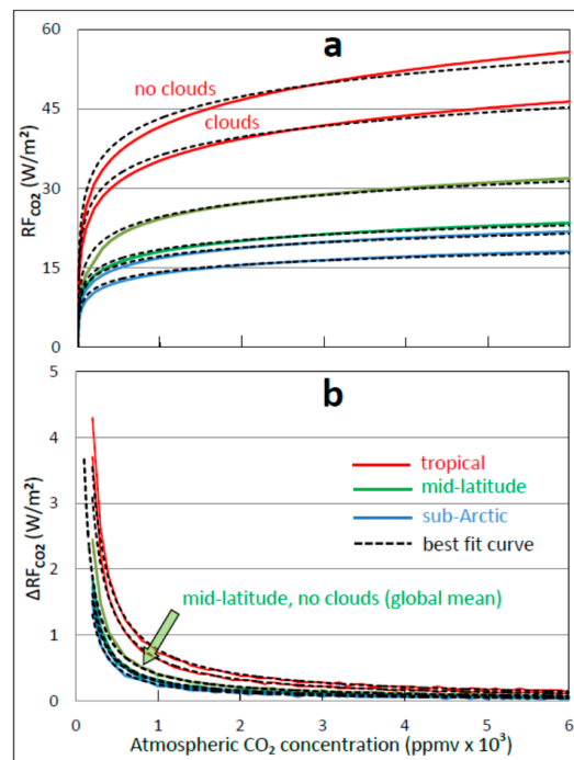
Figure 8. Relationship among atmospheric CO 2 concentration, radiative forcing (RF) and marginal radiative forcing ( \Delta RF_{CO_2} ) computed using MODTRAN. Each graph shows a family of curves for three latitudes (key in (b)) and two cloud conditions (labeled only for the top pair of red curves in (a)). For each latitude the upper curve pertains to a cloudless sky and the lower curve to a cloudy sky containing cumulus clouds starting a base at 0.66 km and a top of 2.7 km. Remaining model parameters used to generate curves are described in the text. (a) Atmospheric CO 2 concentration versus RF at the tropopause. (b) Difference analysis of the curves in (a) to show marginal radiative forcing ( \Delta RF_{CO_2} ), i.e., the change in forcing associated with a unit increment in atmospheric CO 2 . Colored curves are in all cases computed from MODTRAN while the dashed black curves are best-fit logarithmic (a) or power function trendlines (b). Abbreviations: ppmv, parts per million by volume; W/m 2 , Watts per square meter. The arrow identifies the reference curve used for computing \Delta RF_{CO_2} decay constants because it most closely approximates values for the International Standard Atmosphere (see text).
