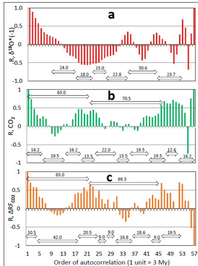
Figure 12. Lagged (serial) autocorrelation coefficient, R , of time series of Phanerozoic climate variables over the time period from 174 to 0 Mybp. The periodicity in the autocorrelation profiles demonstrates non-random periodicity in the corresponding climate variables. (a) \delta^{18}O^*(-1) . Average cycle duration, 22.4 My. (b) Atmospheric CO 2 concentration. Average short cycle, 16.9 My. Average long cycle, 66.8 My. (c) \Delta RF_{CO_2} . Average short cycle, 17.2 My. Average long cycle, 66.2 My. Double-headed arrows demarcate the approximate times of cycles and sub-cycles identified visually.
