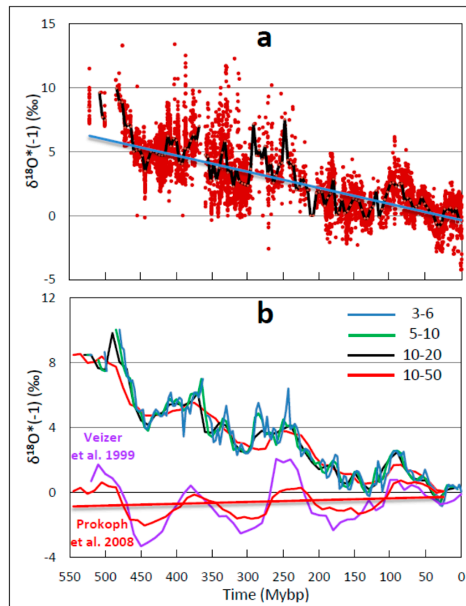
Figure 3. Temperature proxies over the Phanerozoic Eon. (a) Raw temperature data (red datapoints) and fitted black curve (3–6 My moving average). Original data are from Prokoph et al. [28]. (b) averaged non-detrended (upper curves) and linearly-detrended (lower curves) temperature proxy data. The curves of moving averages are color coded following the key in My. In (b), detrended older data from Veizer et al. [38] and inclusive newer and more comprehensive data from Prokoph et al. [28] are compared (lower curves).
