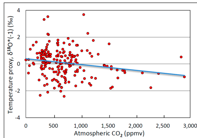
Figure 6. Scatter plot of linearly-detrended temperature-proxy data averaged in one-My bins from 425 to 0 Mybp versus atmospheric carbon dioxide concentration. The negative correlation coefficient ( R = -0.19 , n = 206 ) is discernibly different from zero ( p = 0.006 ) but weak ( R^2 = 0.036 ). The trendline was fitted by the method of least squares.
