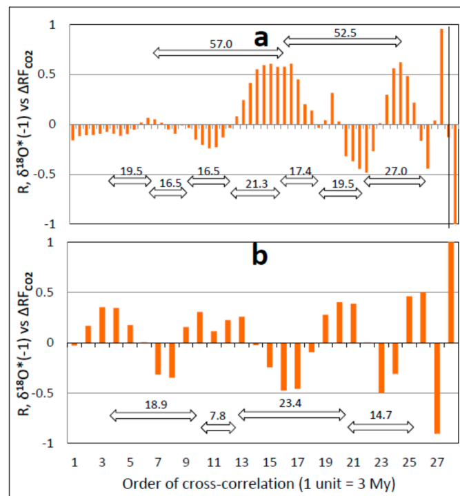
Figure 15. As in Figure 14, but for \delta^{18}\text{O}^*(-1) and \Delta\text{RF}_{\text{CO}_2} . (a) Time period from 174 to 0 Mybp. Average short and long cycle durations, 19.7 and 54.8 My respectively. (b) Time period from 174 to 87 Mybp. Average short cycle duration, 16.2 My. Otherwise as in the legend of Figure 12.
