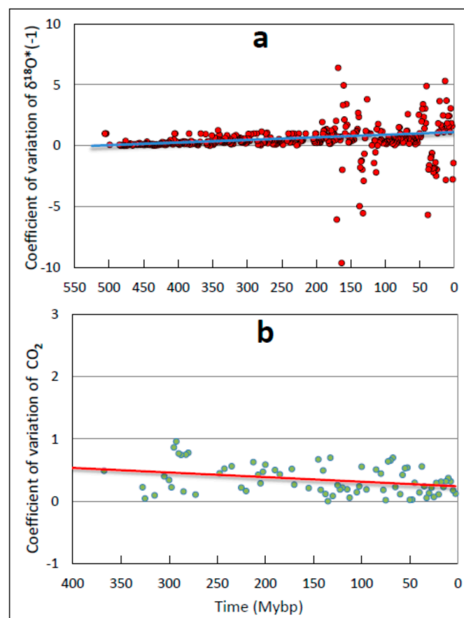
Figure 1. Variance in repeat proxy measurements over the Phanerozoic Eon. The coefficient of variation (the standard deviation divided by the mean) is plotted against sample age using data grouped in bins of 2.5 My for the temperature (a) and atmospheric \text{CO}_2 concentration (b) proxies used in this study. These graphs suggest that older samples are affected minimally by degeneration of data quality (e.g., diagenesis).
