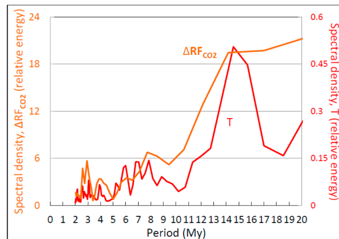
Figure 10. Spectral power periodograms of \Delta RF_{CO_2} and T in the Phanerozoic climate. The orange and red curves show \Delta RF_{CO_2} and T spectral density profiles, respectively. The temperature periodogram was constructed using linearly-detrended proxy data. Time periods covered and (in parentheses) Fisher's Kappa and the corresponding probability that the atmospheric CO_2 concentration and T periodograms result from white (Gaussian) noise are 85 to 0 My (8.26, 0.005) and 522 to 0 My (28.98, 2 \times 10^{-13} ), respectively.
