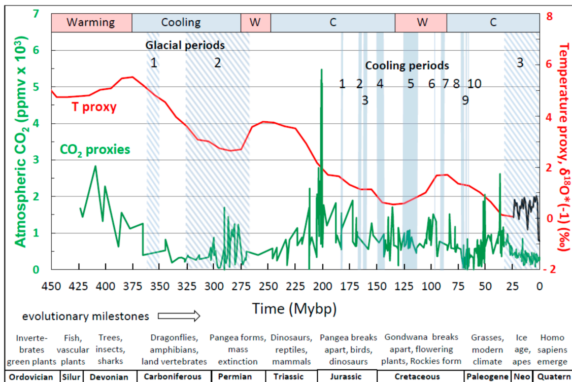
Figure 5. Temperature (T) and atmospheric carbon dioxide (CO 2 ) concentration proxies during the Phanerozoic Eon. Time series of the global temperature proxy ( \delta^{18}\text{O}^*(-1) , red curve, n = 6680 ) are from Prokoph et al. [28] while concurrent atmospheric CO 2 concentration proxies (green curve, n = 831 ) are from Royer [40]. The red curve plots moving averages of the non-detrended T proxy averaged in 50 My windows incremented in ten-My steps (the 10–50 My moving average in Figure 3b). The green curve shows mean CO 2 concentration values in one-My bins averaged over high-resolution portions of the CO 2 record (the most recent Phanerozoic) and linearly interpolated over low-resolution portions (the older Phanerozoic). Glaciations based on independent sedimentary evidence are designated by vertical blue cross-hatched areas, while putative cool periods are designated by vertical solid blue bars. Major cooling and warming cycles are shown by the colored bars across the top while geological periods and evolutionary milestones are shown across the bottom. Abbreviations: CO 2 , atmospheric concentration of carbon dioxide based on various proxies (Methods); ppmv, parts per million by volume; Silu, Silurian; Neo, Neogene; Quatern, Quaternary. The three major glacial periods and ten cooling periods identified by blue cross-hatches and solid lines, respectively, are (after [21]): Glacial periods . 1. late Devonian/early Carboniferous; 2. Permo-Carboniferous; 3. late Cenozoic. Cooling periods . 1. late Pliensbachian; 2. Bathonian; 3. late Callovian to mid-Oxfordian; 4. Tithonian to early Berriasian; 5. Aptian; 6. mid-Cenomanian; 7. mid-Turonian; 8. Campanian-Maastrichtian boundary; 9. mid-Maastrichtian; 10. late-Maastrichtian.
