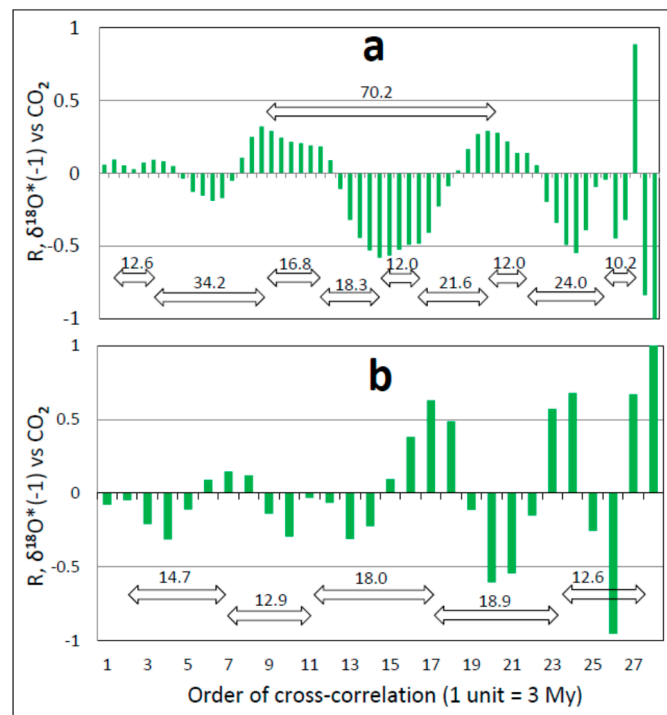
Figure 14. Lagged (serial) cross-correlation coefficient, R , of temperature and atmospheric \text{CO}_2 concentration proxies. (a) Time period from 174 to 0 Mybp. Average short cycle duration, 17.9 My. Average long cycle duration, 70.2 My. (b) Time period from 174 to 87 Mybp. Average short cycle duration, 15.4 My. Otherwise as in the legend of Figure 12.
