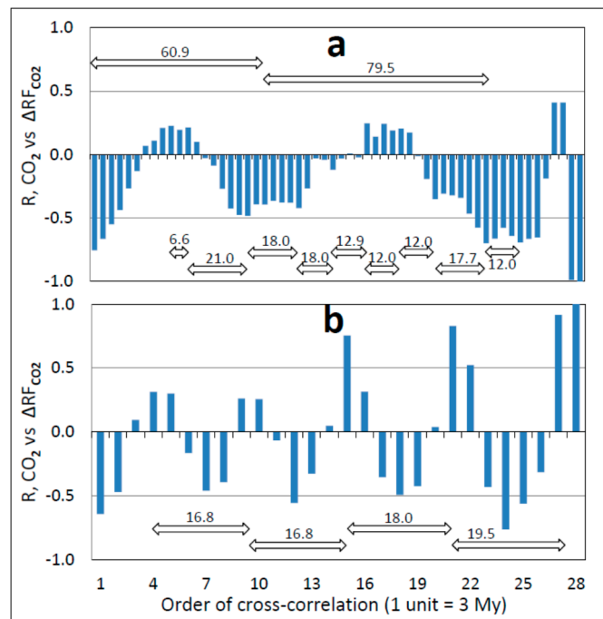
Figure 16. As in Figure 14, but for atmospheric \text{CO}_2 concentration and \Delta \text{RF}_{\text{CO}_2} . (a) Time period from 174 to 0 Mybp. Average short and long cycle durations, 14.5 and 70.2 My respectively. (b) Time period from 174 to 87 Mybp. Average short cycle duration, 17.8 My. The strong negative correlation coefficients at low shift orders demonstrate the antiphase (inverse) relation between atmospheric \text{CO}_2 concentration and \Delta \text{RF}_{\text{CO}_2} . Otherwise as in the legend of Figure 12.
