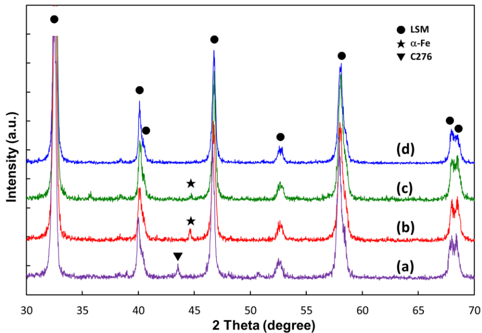
Figure S2. X-ray diffraction pattern of the plasma sprayed LSM-coated (a) C276, (b) Crofer22 APU, (c) SUS430, (d) SUS304 alloys after oxidation for 300 h in air at 800 °C.
