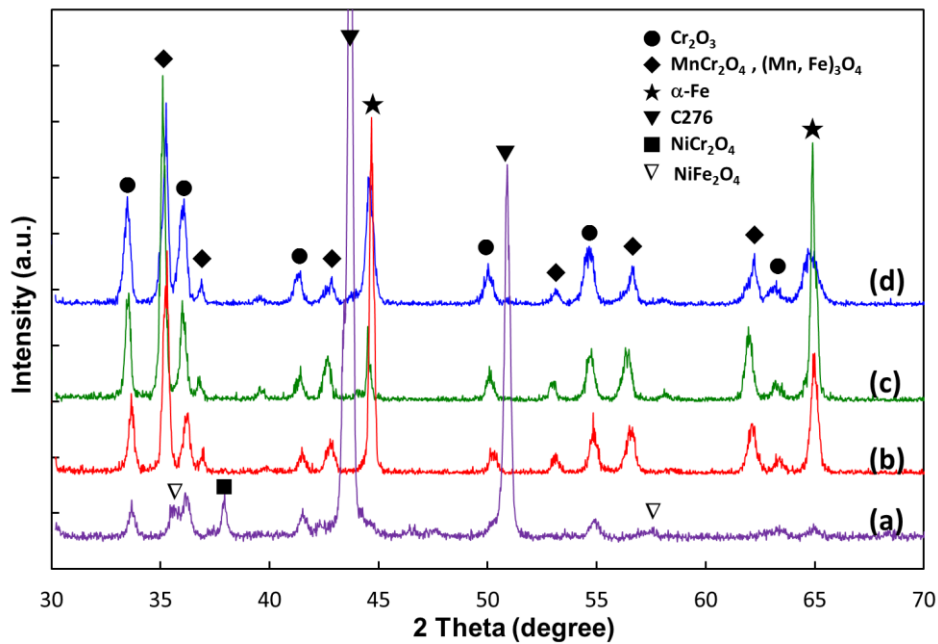
Figure S1. X-ray diffraction pattern of (a) C276, (b) Crofer22 APU, (c) SUS430, (d) SUS304 alloy after oxidation at 800 °C for 300 h.
