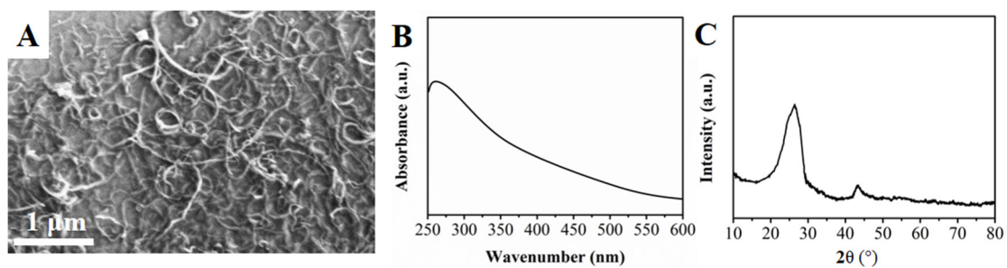
Figure S1. (A) SEM image, (B) UV-Vis spectrum and (C) XRD pattern of MWCNTs.
