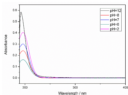
Figure 9. The UV-Vis spectra of FCMSs in acidic, alkaline and neutral suspensions.
