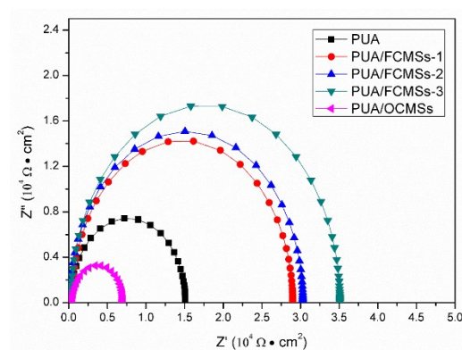
Figure 14. Nyquist plots of UV-curable polyurethane composite coatings.
