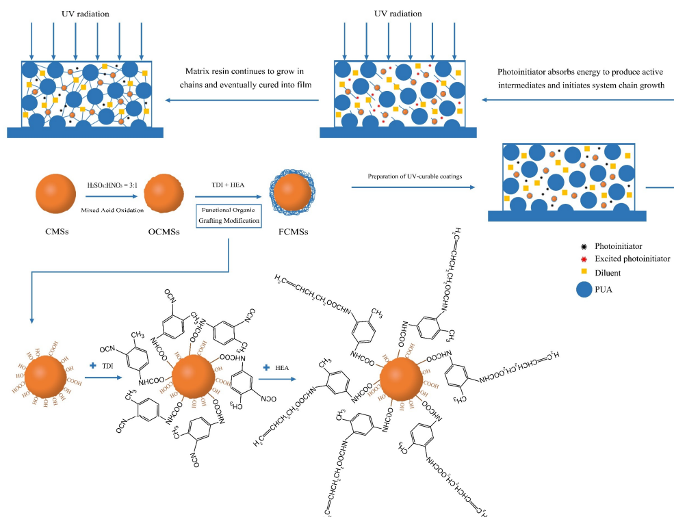
Figure 1. Schematic illustration of the synthesis procedures of functional coated microspheres (FCMs) and UV curing procedure of hydrophobic coatings of functionalized carbon microspheres.
