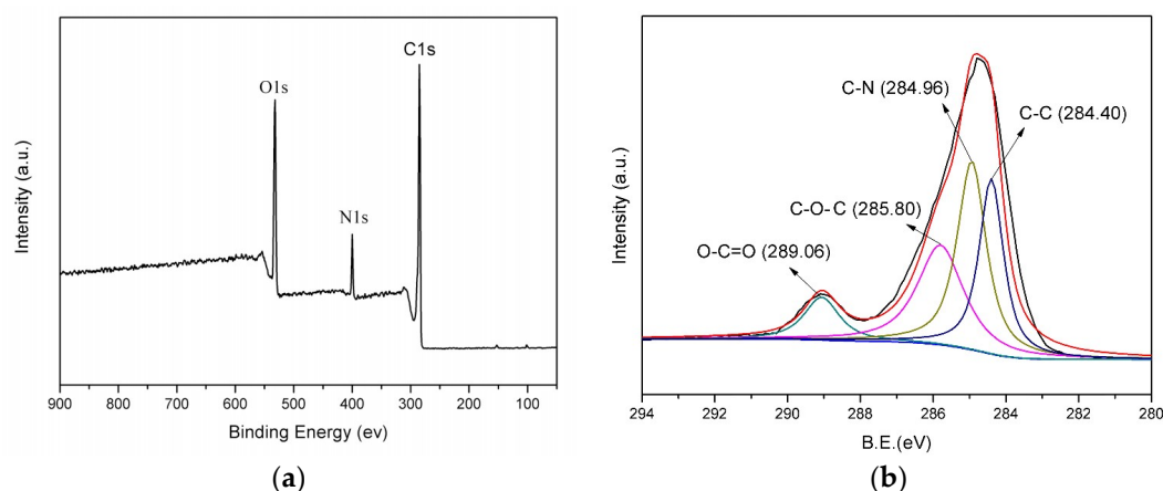
Figure 4. (a) The X-ray photoelectron spectroscopy (XPS) spectra of FCMSs; (b) The C1s spectra of FCMSs.
