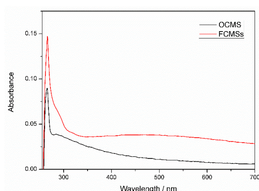
Figure 7. The UV-Vis spectra of FCMSs and OCMSs.
