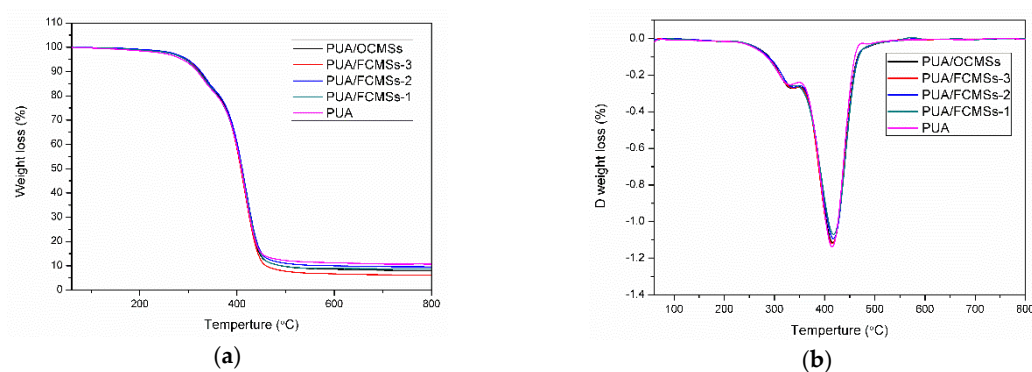
Figure 10. (a) The thermogravimetric analysis (TGA) spectra of UV cured films; (b) The Differential thermal gravity (DTG) spectra of UV-cured films.
