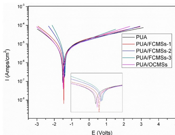
Figure 16. The polarization curve of UV-curable polyurethane composite coatings.
