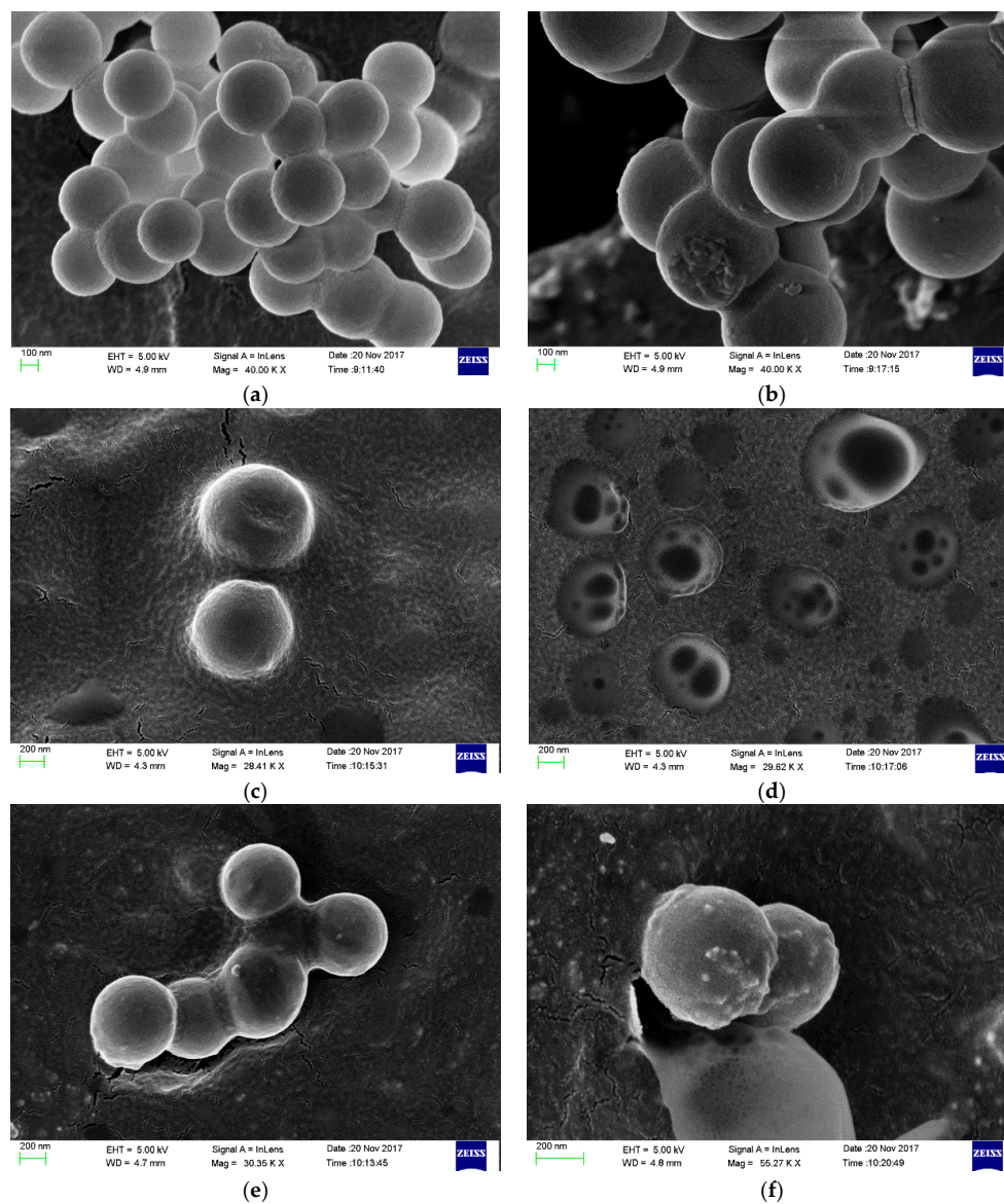
Figure 13. The SEM image of section of samples. (a) CMSs; (b) OCMSs; (c) PUA/FCMSs-3; (d) PUA/FCMSs-3; (e) PUA/OCMSs; (f) PUA/OCMSs.
