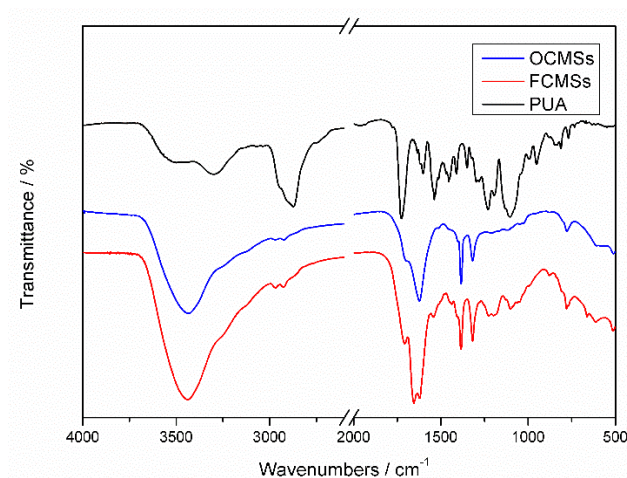
Figure 2. The FTIR spectra of polyurethane acrylates (PUA), organic carbon microspheres (OCMSs) and FCMSs.
