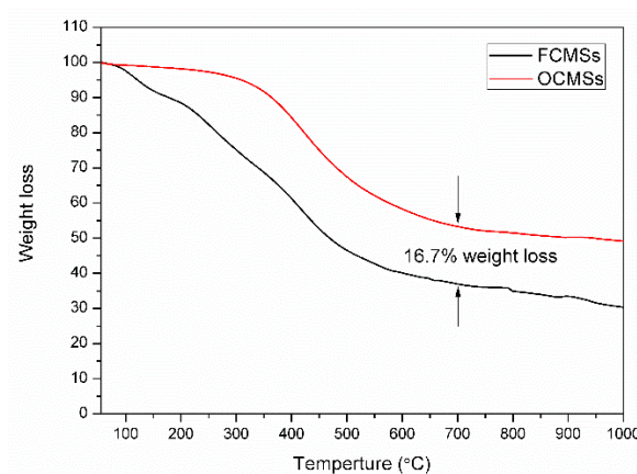
Figure 5. The TG spectra of FCMSs and OCMSs.
