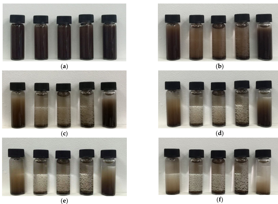
Figure 8. The dispersity of FCMSs in the solutions with different pH. (a) Initial state; (b) 2 h; (c) 5 h; (d) 8 h; (e) 11 h; (f) 24 h. Images in each picture from left to right were the solution with the pH of 2, 6, 7, 8 and 12.
