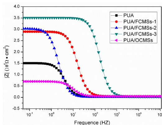
Figure 15. Bode spectrum of UV-curable polyurethane composite coatings.
