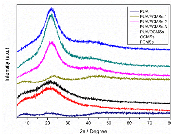
Figure 12. X-ray diffraction images of OCMSs and FCMSs.
