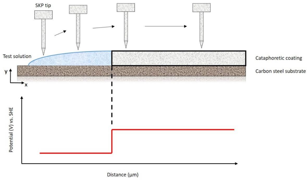
Figure S2. Working principle of the SKP equipment.
