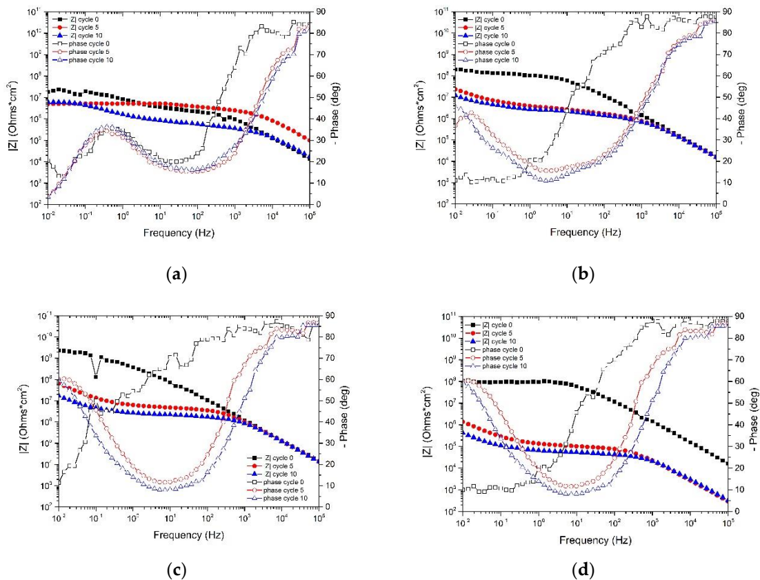
Figure S1. EIS Bode modulus and phase diagrams of (a) sample g-0; (b) sample g-0.1; (c) sample g-0.2 and (d) sample g-0.5, during the AC-DC-AC measurements.
