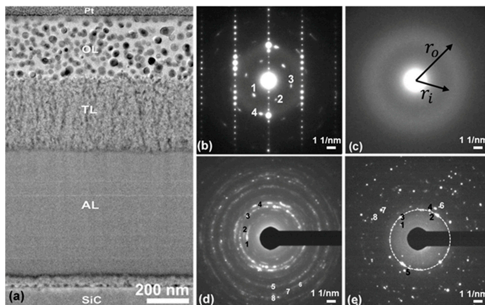
Figure 2. (a) Cross-section TEM image of the annealed Hf 6 B 10 Si 31 C 2 N 50 film. SAED pattern taken from (b) substrate, (c) amorphous layer, (d) transition layer and (e) top oxide layer shown in (a).
