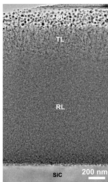
Figure 8. Cross-section TEM image of the \text{Hf}_7\text{B}_{10}\text{Si}_{32}\text{C}_2\text{N}_{44} film annealed up to 1500 °C in air.
