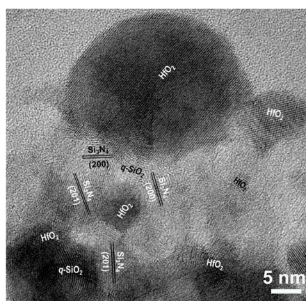
Figure 12. HRXTEM image of the oxide/transition layer interface in the annealed \text{Hf}_7\text{B}_{10}\text{Si}_{32}\text{C}_2\text{N}_{44} film.
