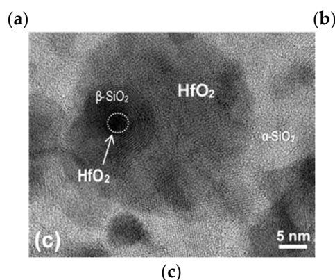
Figure 7. Plan-view HRTEM images taken from the oxide/transition layer interface in the annealed \text{Hf}_6\text{B}_{10}\text{Si}_{31}\text{C}_2\text{N}_{50} film (a–c).
