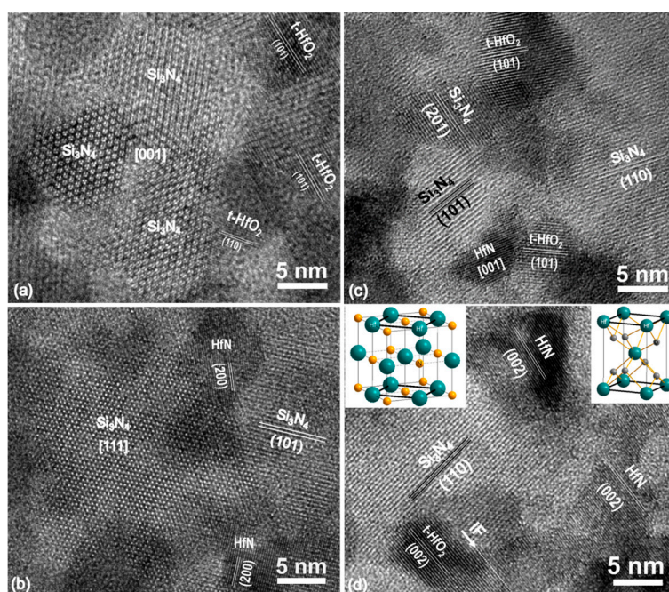
Figure 11. HRXTEM images taken from (a) the transition layer and (b) bottom, (c) top, and (d) middle section of the recrystallized layer in the annealed Hf 7 B 10 Si 32 C 2 N 44 film.
