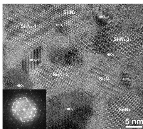
Figure 6. Plan-view HRTEM image (with inset FFT) of local structure between \text{Si}_3\text{N}_4 and \text{HfO}_2 nano grains in the transition layer in the \text{Hf}_{60}\text{B}_{10}\text{Si}_{31}\text{C}_2\text{N}_{50} film.
