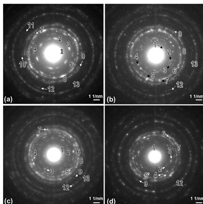
Figure 10. SAED pattern taken from the (a) bottom, (b) middle, and (c) top section of the recrystallized layer and (d) transition layer in the annealed \text{Hf}_{7.1}\text{B}_{10}\text{Si}_{32}\text{C}_2\text{N}_{44} film.
