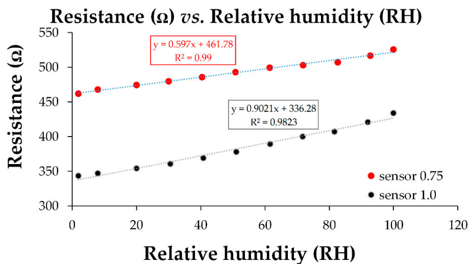
Figure 9. The transfer function of the quaternary nanohybrid-based resistive sensors in humid nitrogen (RH = 0–100%).
