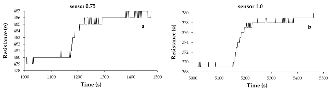
Figure 11. Response time of the RH resistive at room temperature for 40% RH–50% RH step: (a) sensor 0.75 and (b) sensor 1.0.
