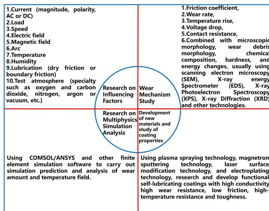
Figure 17. A summary of the research direction and content of the current-carrying friction and wear.
