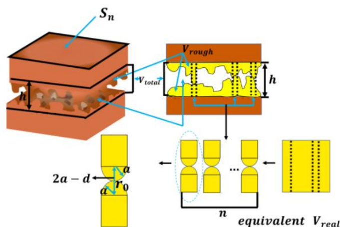
Figure 3. Schematic diagram of the contact volume and equivalent actual contact volume between rough surfaces [17].
