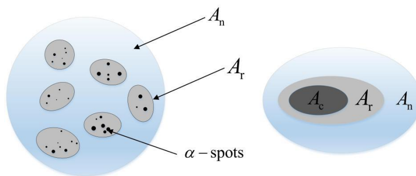
Figure 15. The three contact areas and contact area sets on the surface of the friction pair.
