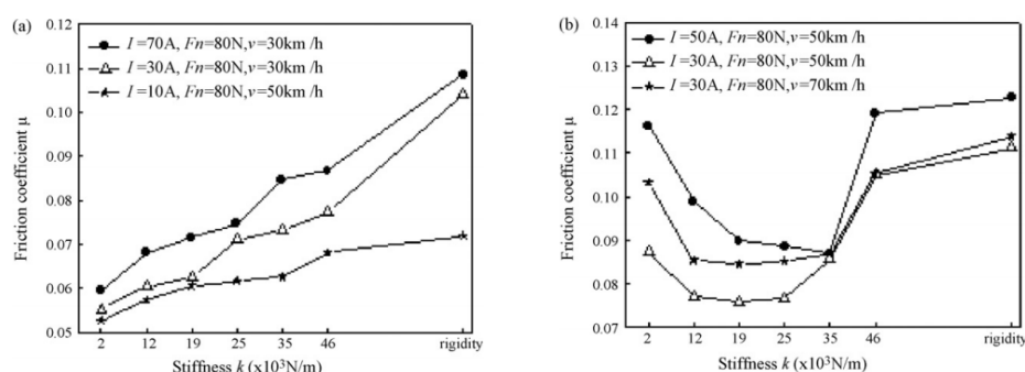
Figure 9. Variation in the friction coefficient with spring stiffness: (a) at low speed or low current, (b) at high speed or high current [62].
