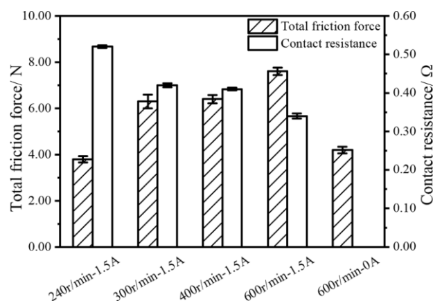
Figure 8. The total friction force and contact resistance at steady-state with different rotation speeds [54].
