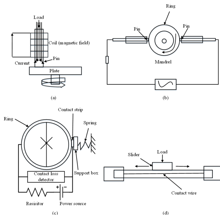
Figure 2. Four typical current-carrying friction and wear test devices [13–16]: (a) pin-disc type; (b) pin-ring type; (c) ring-block type; (d) line slider type.
