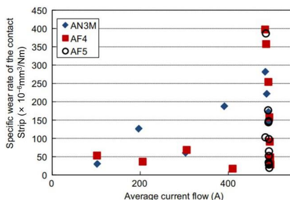
Figure 5. The relationship between the electrical current and wear of the C/C composite contact strips [24].
