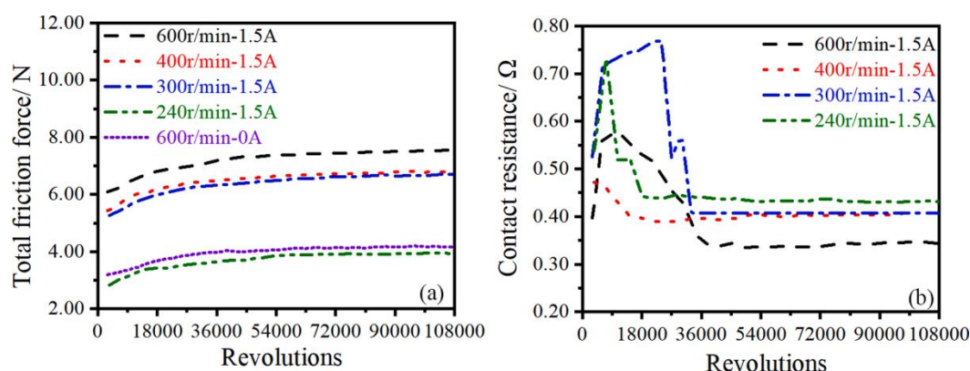
Figure 7. The effect of the rotation speed on the real-time (a) total friction force and (b) contact resistance [54].
