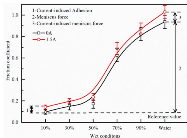
Figure 13. A comparison of the final friction coefficient with and without a current under different wet conditions [92].
