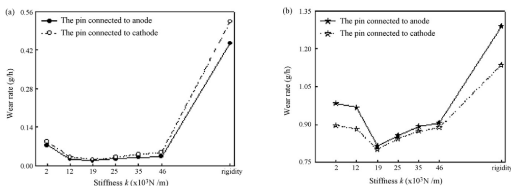
Figure 10. The wear rate as a function of spring rate: (a) I = 30 A, F_n = 80 N, v = 30 km/h, (b) I = 30 A, F_n = 80 N, v = 70 km/h [62].
