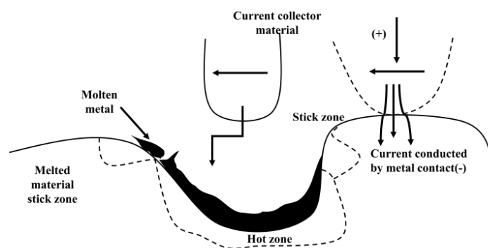
Figure 14. A schematic diagram of the current-carrying friction and wear model.
