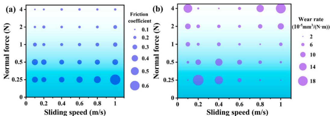
Figure 11. The friction coefficient (a) and wear rate (b) of the Ag/MoS 2 /WS 2 nanocomposites under different normal forces and sliding speeds [87].
