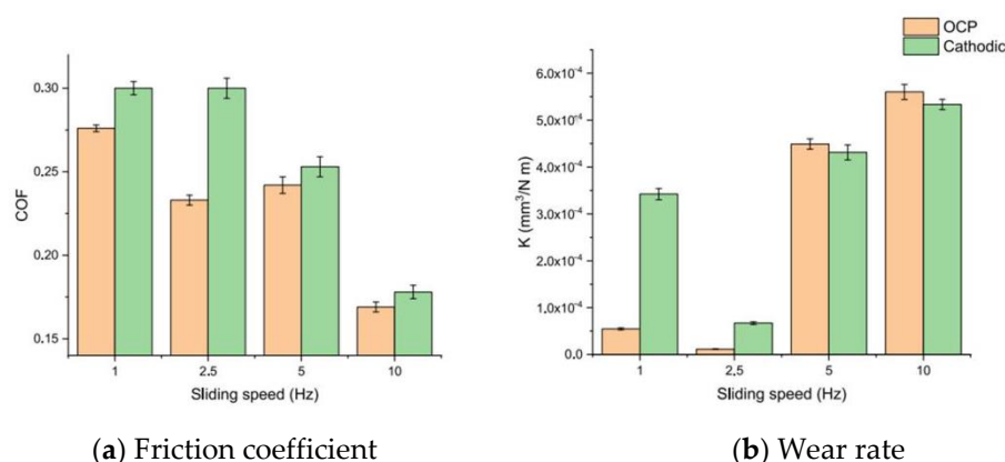
Figure 6. The coefficient of friction (COF) (a) and the specific wear rate K (b) as a function of the sliding speed under cathodic potential and OCP [27].
