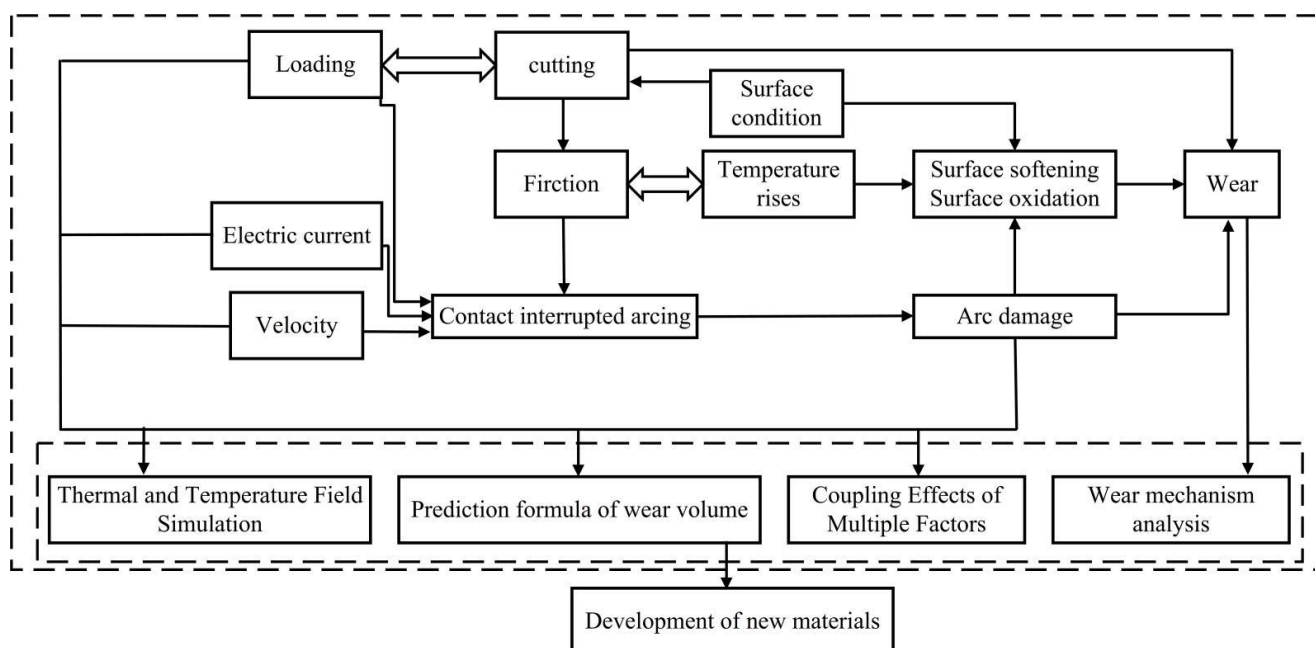
Figure 4. The current-carrying friction and wear research field.
