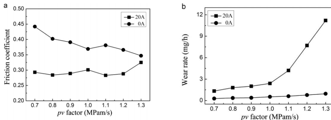
Figure 12. Variations in the (a) friction coefficient and (b) wear rate with the PV factor [88].
