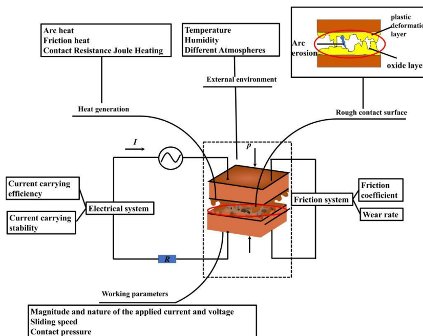
Figure 16. The current-carrying friction and wear contact system model.
