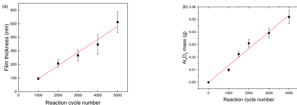
Figure 1. Al_2O_3 film growth analysis, including (a) the film thickness as a function of the number of reaction cycles on a Si(100) substrate, and (b) the mass of the Al_xO_y film post-ALD process as a function of the reaction cycles on a CFF substrate.
