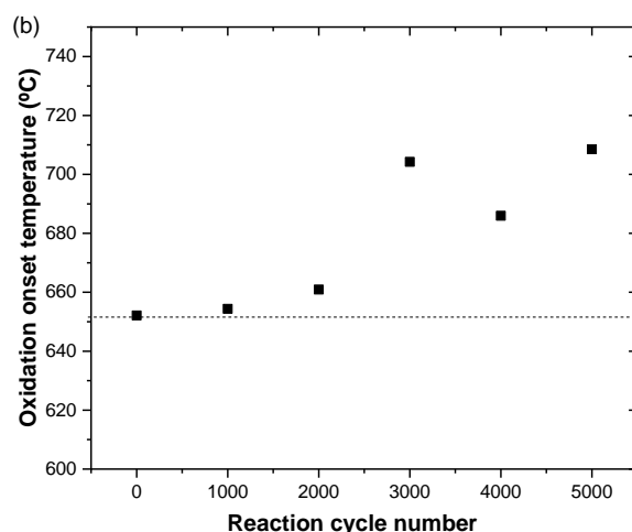
Figure 8. (a) TGA curves of CFF without and with varying ALD-coated \text{Al}_x\text{O}_y film thicknesses as indicated by deposition cycles. (b) Variation in oxidation onset temperature with respect to ALD cycle number.
