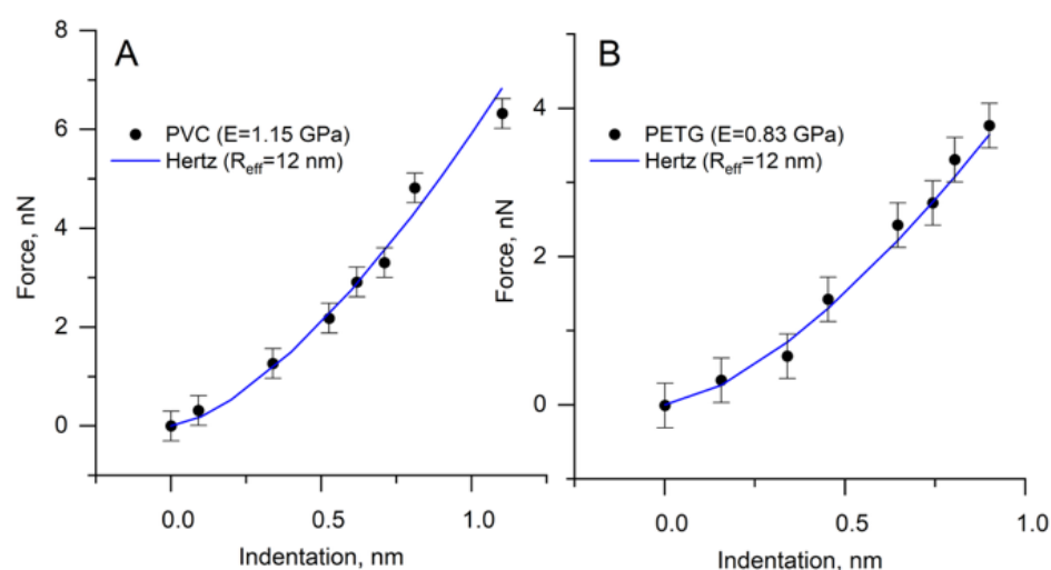
Figure 7. Force–indentation dependencies and fitted Hertz model with TRIANG2 probe. (A). PVC. (B). PETG.
