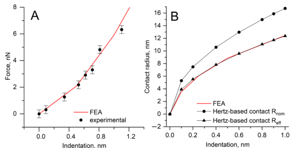
Figure 4. (A). Force-indentation FEA model comparison with experimental data, with R_{SEM} = 17.3 nm. (B). Contact radius-indentation nonlinear dependencies obtained from FEA, compared with the ones obtained using nominal geometry R_{nom} and contact parameter R_{eff} .
