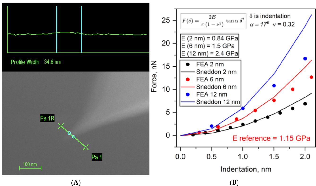
Figure 1. (A). Scanning electron microscopy view of TRIANG2 cantilever tip. (B). Force–indentation curves simulated with FEA and compared with Sneddon model. Profile width is measured between points Pa 1 and Pa 1R.
