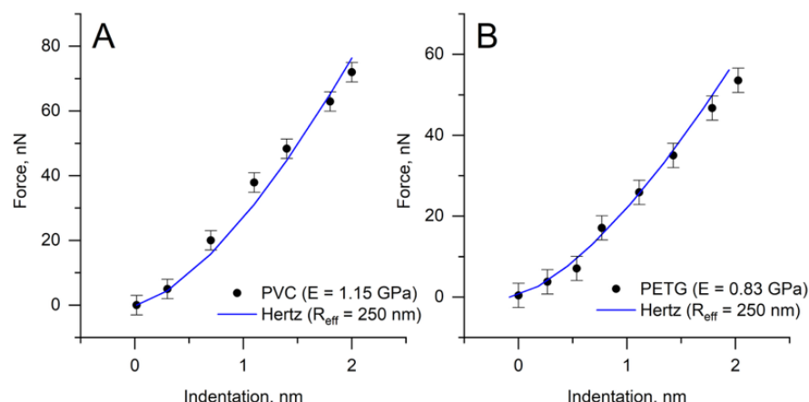
Figure 11. Force–indentation dependencies and fitted Hertz model with FLAT4000 probe. (A). PVC. (B). PETG.
