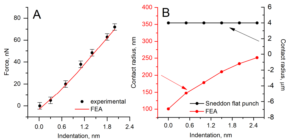
Figure 8. (A). Force–indentation curve fitted with FEA model. (B). Contact radius dependence on indentation.
