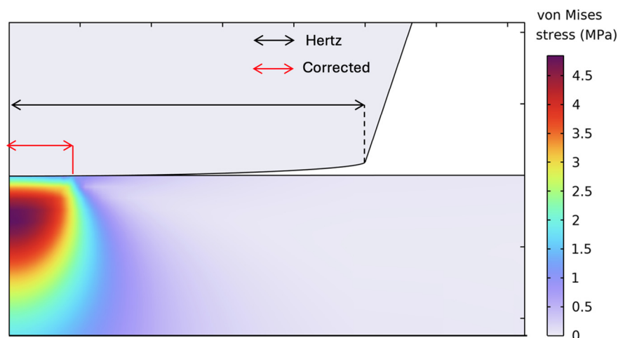
Figure 9. Visualization of contact radius: Hertz assumption vs. FEA.
