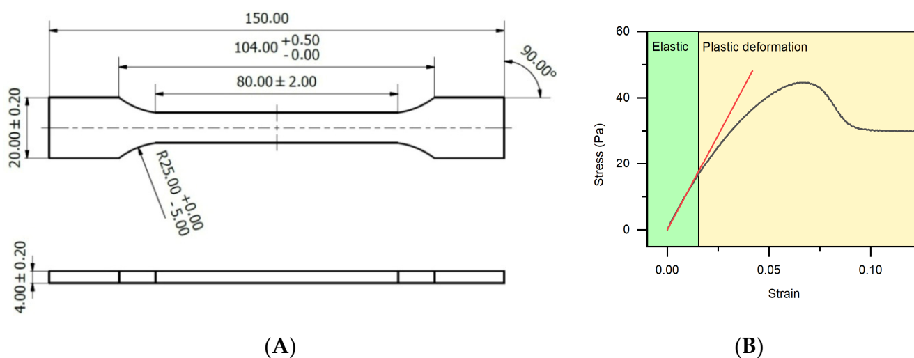
Figure 2. Specimen geometry and stress–strain response used for the determination of the elastic modulus E_{ref} . (A) Geometry and dimensions of the tensile test specimen. (B) Stress–strain curve with indication of the elastic region used to determine the elastic modulus E .
