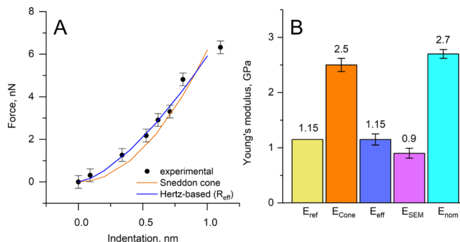
Figure 6. Experimental force vs. indentation curves and fitted models. (A). Hertz and Sneddon's cone models fitted to TRIANG2 experimental data. (B). Reference Young's modulus compared with that obtained from fitting.
