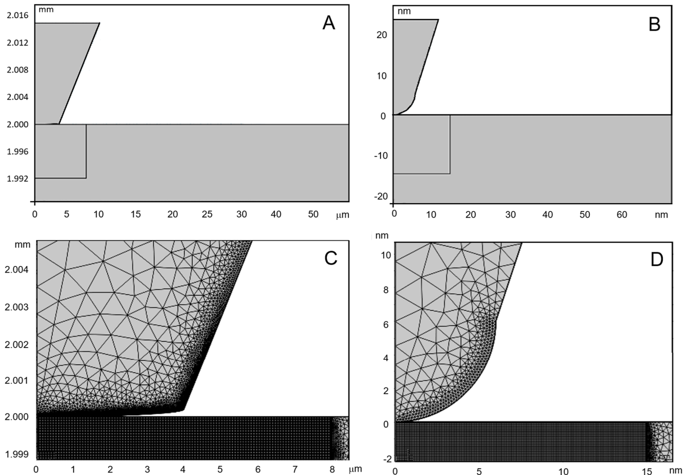
Figure 3. FEA model. Domain of the model zoomed around the indenter: (A). FLAT4000, (B). TRIANG2. Mesh distribution: (C). FLAT4000, (D). TRIANG2. Dashed line is symmetry line.
