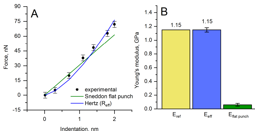
Figure 10. (A). Force dependencies on indentation with FLAT4000 probe. (B). Young's modulus determined by fitting to experimental data.
