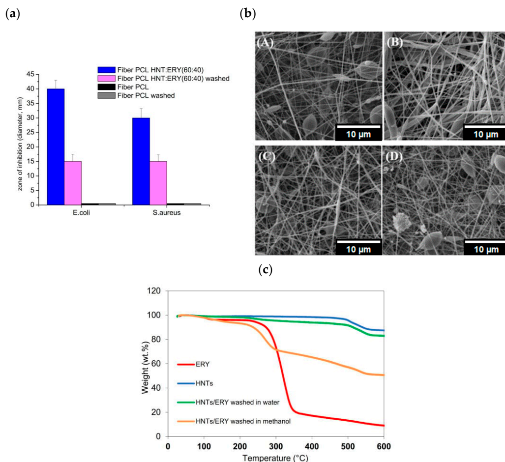
Figure 5. (a) Comparison of the antibacterial activity of washed and unwashed PCL/HNT fibers loaded with ERY, evaluated using the disk diffusion method against E. coli and S. aureus . The antibacterial effect was measured as the inhibition zone diameter and expressed as mean \pm standard error (SE). (b) High-magnification SEM images (5000 \times ) in secondary electron mode of electrospun nanofibers: (A) pure PCL, (B) PCL with 6 wt.% HNT, (C) PCL with 6 wt.% HNT/ERY (80:20), and (D) PCL with 6 wt.% HNT/ERY (60:40). (c) TG curves of ERY, HNTs, HNT/ERY washed with water, and HNT/ERY washed with methanol [89].
