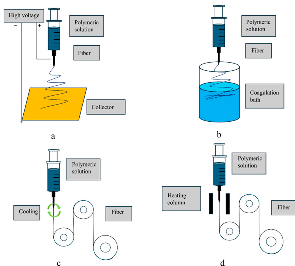
Figure 1. Schematic representation of different techniques for manufacturing fibers: (a) electrospinning, (b) wet spinning, (c) melt spinning, (d) dry spinning.
