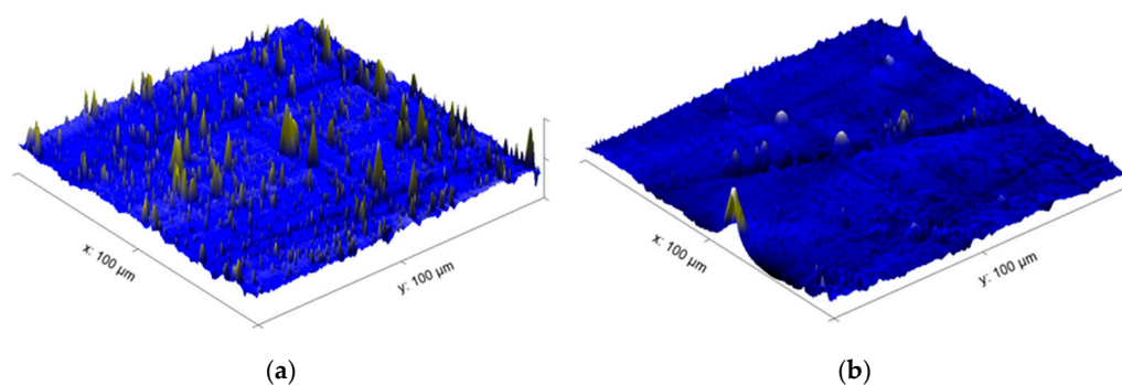
Figure 6. Representative AFM images of super-finished coated substrates used for local morphology comparison: (a) DLC-coated specimen (Ra = 41.903 nm, Rq = 68.999 nm); (b) SiO 2 -coated specimen (Ra = 31.336 nm, Rq = 49.33 nm). Color contrast represents relative surface-height variation in the AFM topography, where blue regions indicate lower surface areas and bright regions indicate higher asperities.
