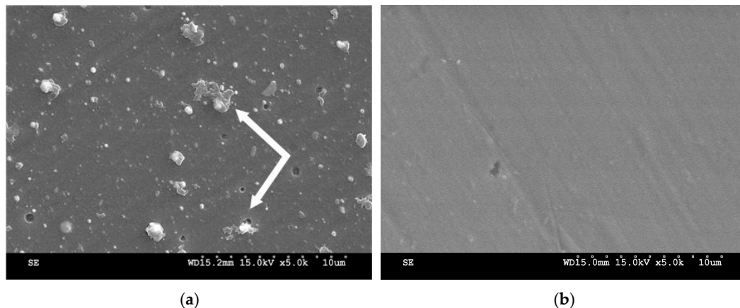
Figure 7. Representative SEM images of super-finished coated substrates used for local morphology comparison: (a) DLC-coated specimen showing localized bright protrusions; (b) SiO 2 -coated specimen showing a comparatively uniform surface morphology. Arrows indicate representative droplet-like surface protrusions observed on the DLC coating.
