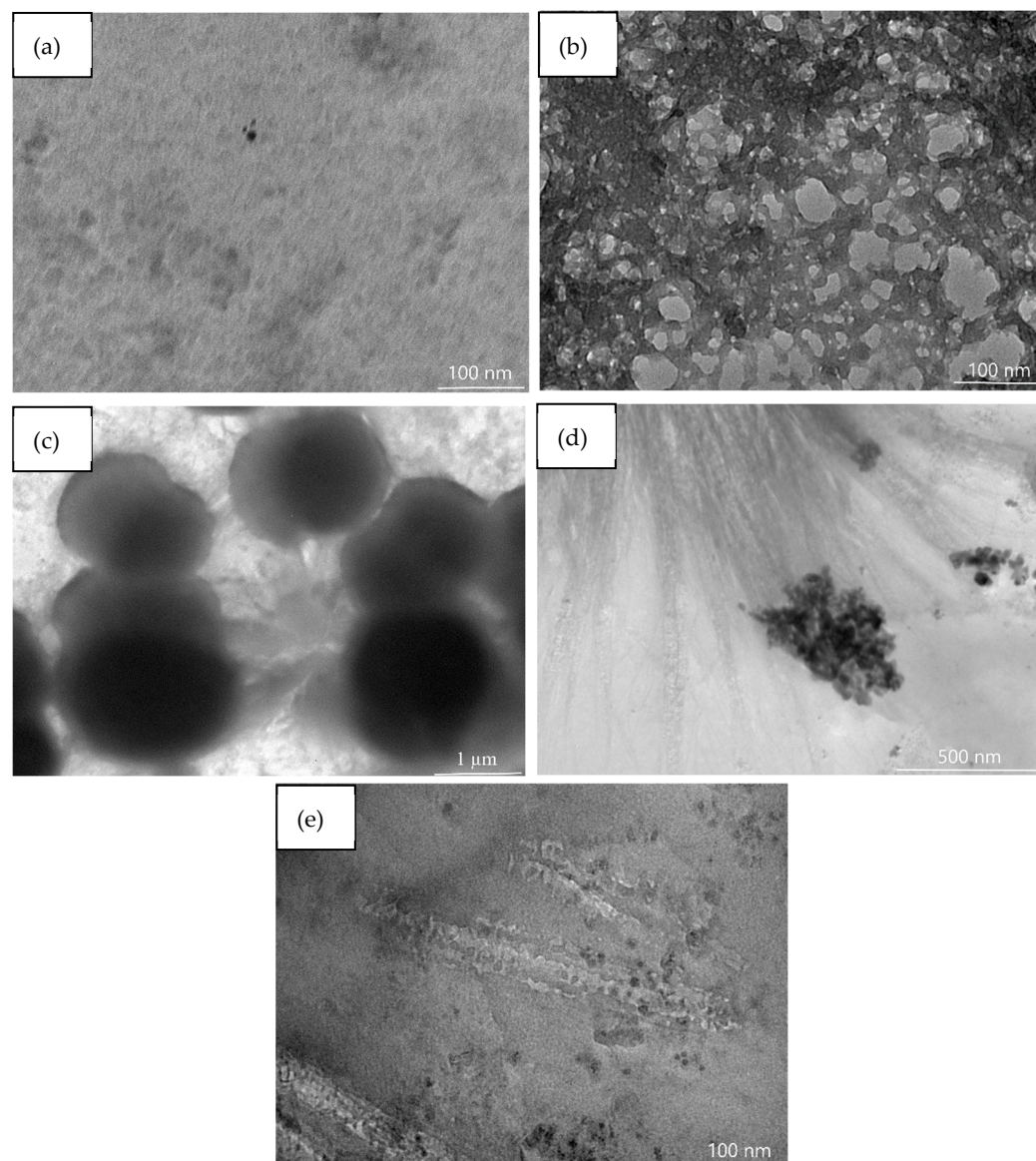
Figure 2. TEM micrographs of XG/CE-ZnO NPs with varying CE amounts: (a) 0.01 g, (b) 0.02 g, (c) 0.05 g, (d) 0.03 g (x20,000) and (e) 0.03 g (x60,000).
