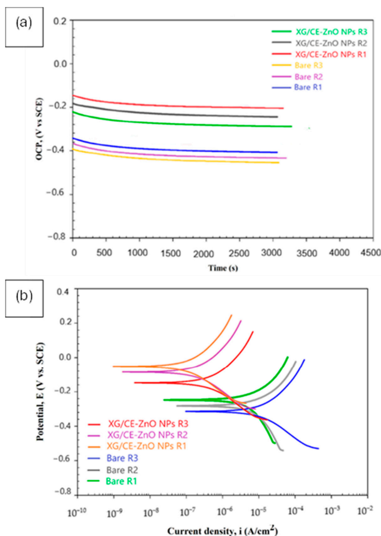
Figure 8. Electrochemical corrosion test results of the uncoated and coated substrates with different roughness: (a) OCP and (b) Tafel graph.
