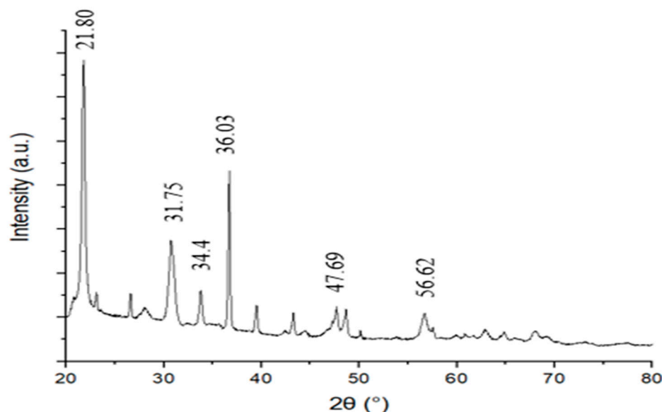
Figure 3. XRD spectrum of the synthesized XG/CE-ZnO NPs.
