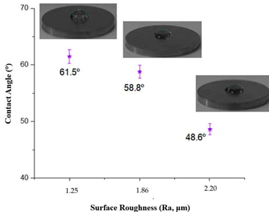
Figure 6. The change in CA with NPs at different Ra.
