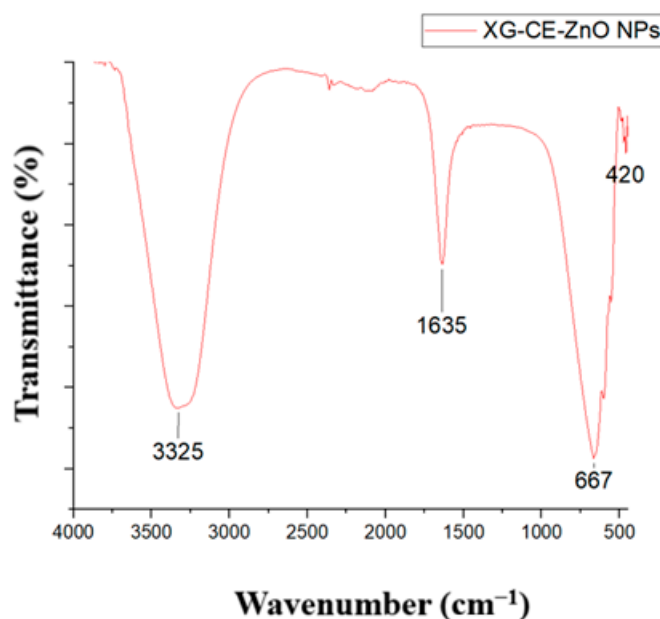
Figure 4. FTIR spectra of the synthesized XG/CE-ZnO NPs.
