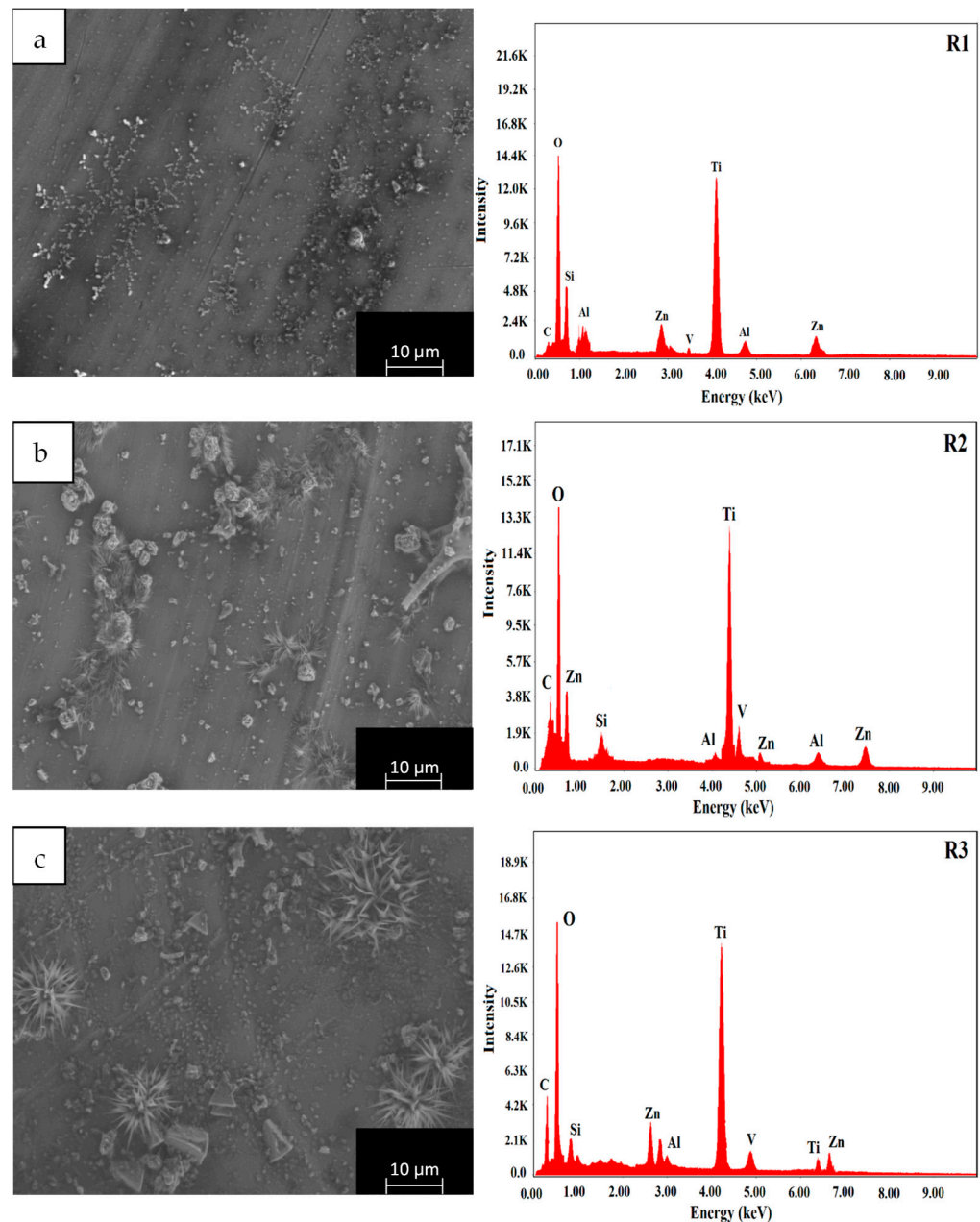
Figure 7. SEM images and EDX results of the coated surfaces at different Ra values: (a) R1, (b) R2, and (c) R3.
