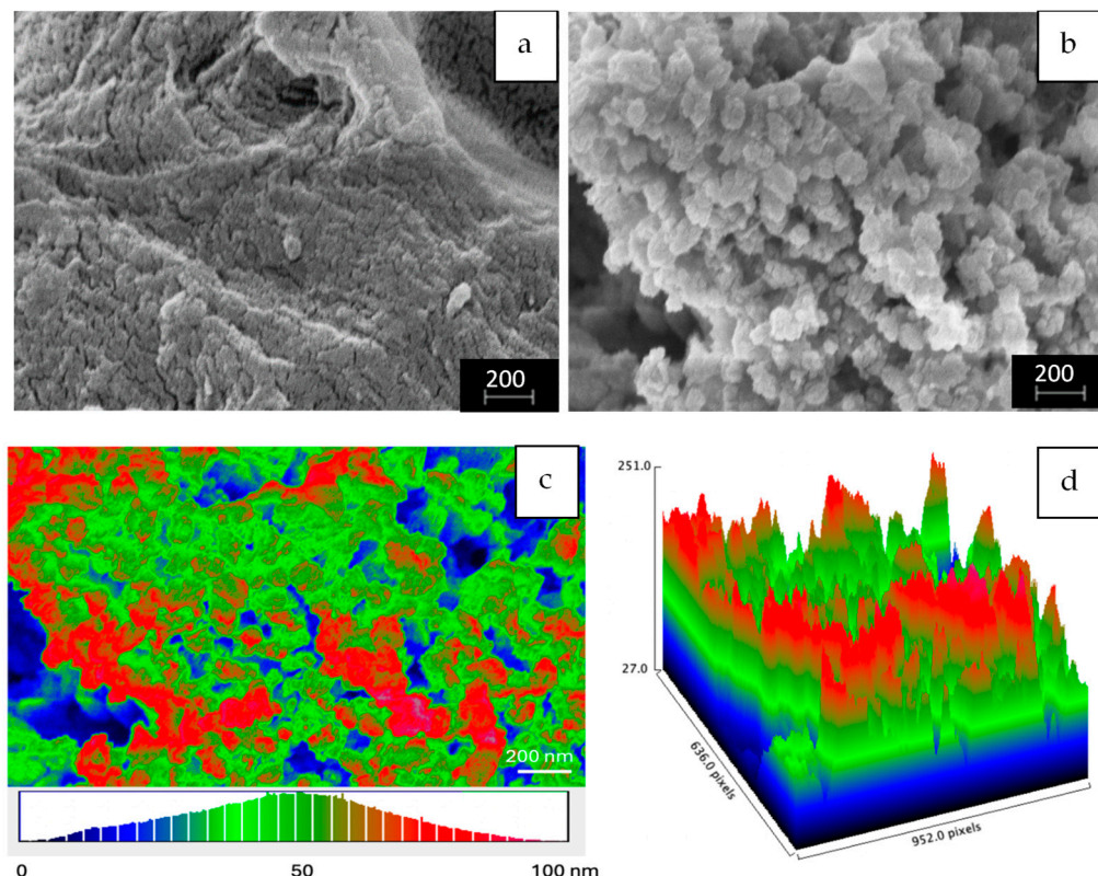
Figure 5. SEM images showcasing (a) pure XG, (b) XG/CE-ZnO NPs, (c) AI-enhanced SEM image of XG/CE-ZnO NPs (Rainbow RGB, 8-bit), and (d) 3D surface plot of XG/CE-ZnO NPs (Rainbow RGB, 8-bit).
