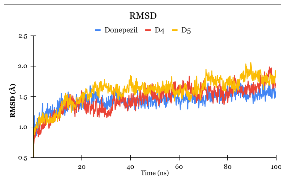
Figure 4. Backbone RMSD of the AChE–ligand complexes over 100 ns of MD simulation for Donepezil, D4 , and D5 .
