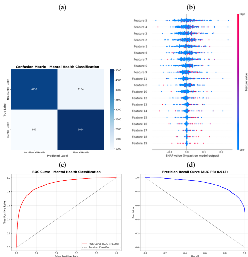
Figure 4. Evaluation and interpretability outputs: (a) confusion matrix; (b) SHAP summary plot; (c) ROC curve; (d) precision–recall curve.
