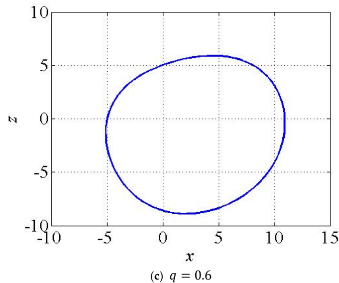
Figure 12. The phase portraits of the proposed 3-D chaotic financial firm system (10) for various values of the parameter q . (a) Periodic attractor at q = 0.1 , (b) chaotic attractor at q = 0.3 , and (c) periodic attractor at q = 0.6 .
