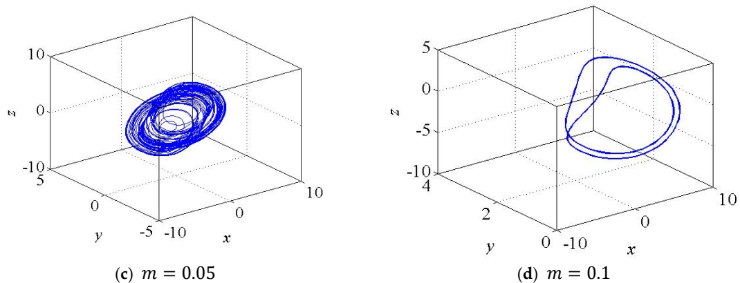
Figure 8. The dynamic analysis of the system (10) for the variation in the parameter m . (a) Bifurcation diagram; (b) LE spectrum; (c) chaotic attractor at m = 0.05 ; and (d) periodic attractor in m = 0.1 .
