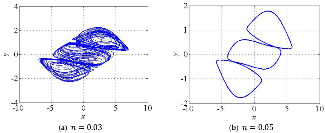
Figure 10. The phase portraits of the proposed 3-D chaotic financial firm system (10) for various values of the parameter n . (a) Chaotic attractor at n = 0.03 , and (b) periodic attractor at n = 0.05 .
