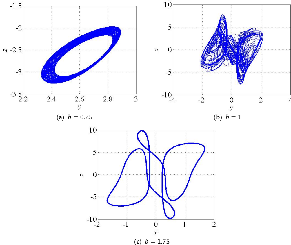
Figure 5. The phase portraits of the new financial firm system (10) for various values of the parameter b . (a) Periodic attractor at b = 0.25 , (b) chaotic attractor at b = 1 , and (c) periodic attractor at b = 1.75 .
