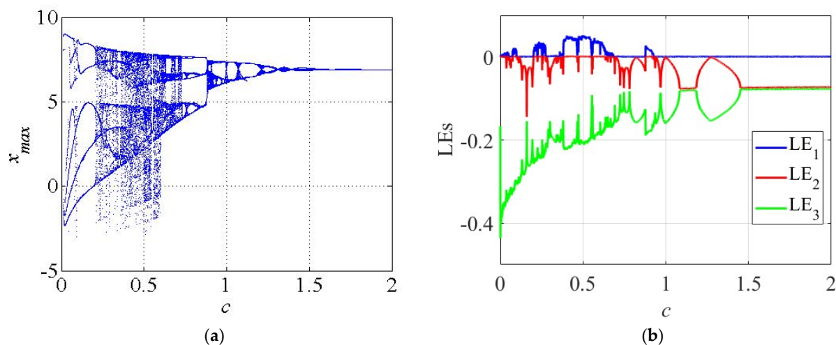
Figure 6. The dynamic analysis of the system (10) for the variation in the parameter c . (a) Bifurcation diagram; (b) LE spectrum.
