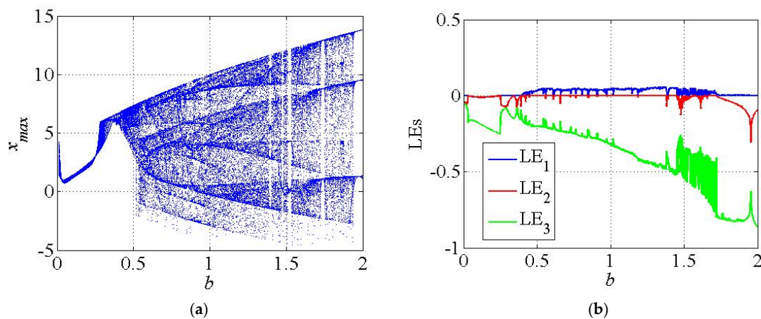
Figure 4. The dynamic analysis of the system (10) for the variation in the parameter b . (a) Bifurcation diagram; (b) LE spectrum.
