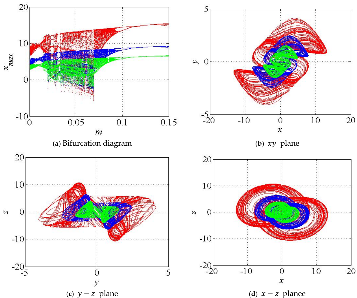
Figure 15. Total amplitude control analysis. (a) Bifurcation diagram of the system (25); (b–d) amplitude regulated attractors in xy , yz and xz plane respectively. The plots are obtained with the scaling parameter \beta = 1 (original system), shown in blue, \beta = 0.6 , shown in red, and \beta = 1.4 shown in green.
