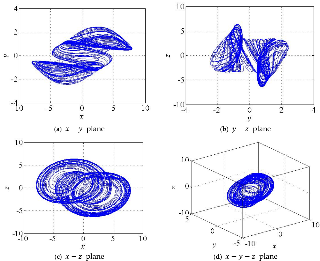
Figure 1. The phase portraits of the new multi-echelon chaotic system (10) in various planes for the initial conditions (0.03, 0.03, 0.03). We confirm that the overlapping content in Figure does not affect the scientific understanding or interpretation of results.
