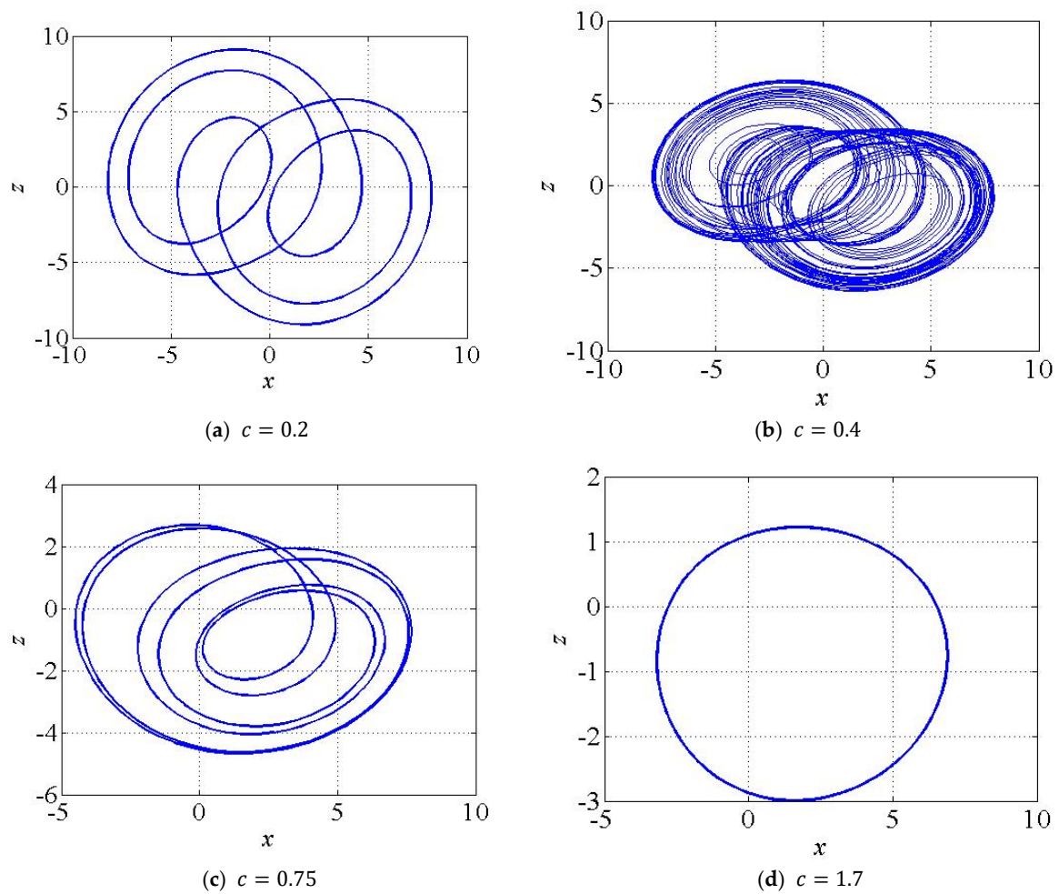
Figure 7. The phase portraits of the new financial firm system (10) for various values of the parameter c . (a) Periodic attractor at c = 0.2 , (b) chaotic attractor at c = 0.4 , (c) periodic attractor at c = 0.75 and (d) periodic attractor at c = 1.7 .
