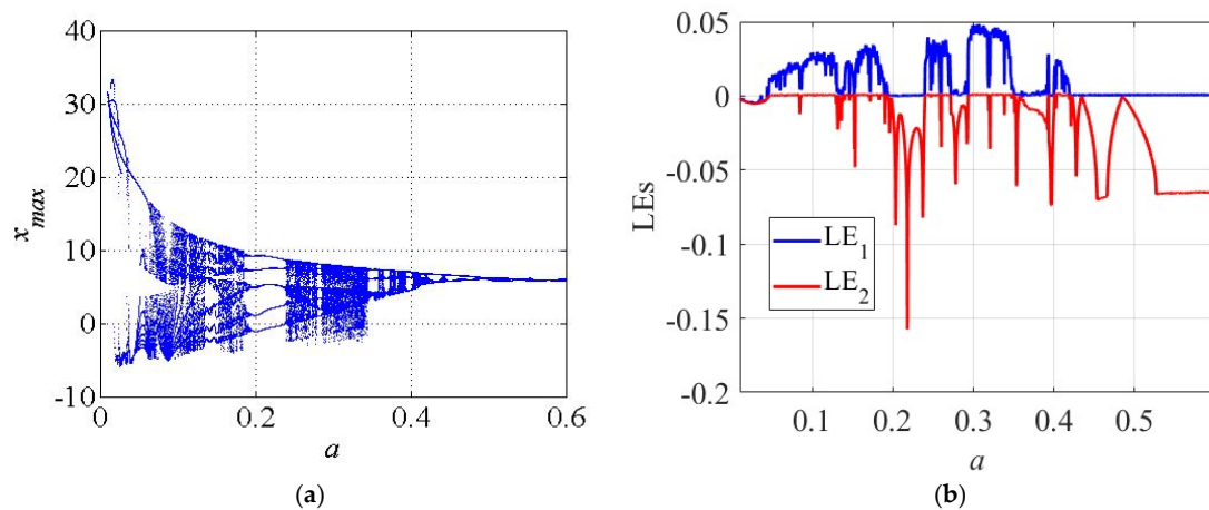
Figure 2. The dynamic analysis of the system (10) for the variation in the parameter a . (a) Bifurcation diagram; (b) LE spectrum.
