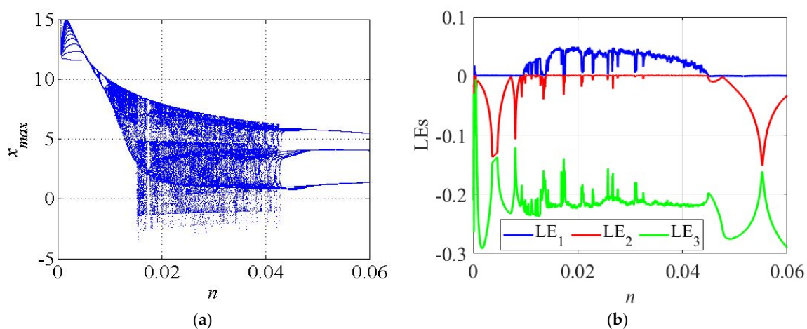
Figure 9. The dynamic analysis of the system (10) for the variation in the parameter n . (a) Bifurcation diagram; (b) LE spectrum.
