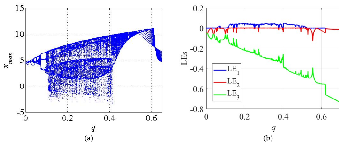
Figure 11. The dynamic analysis of the system (10) for the variation in the parameter q . (a) Bifurcation diagram; (b) LE spectrum.
