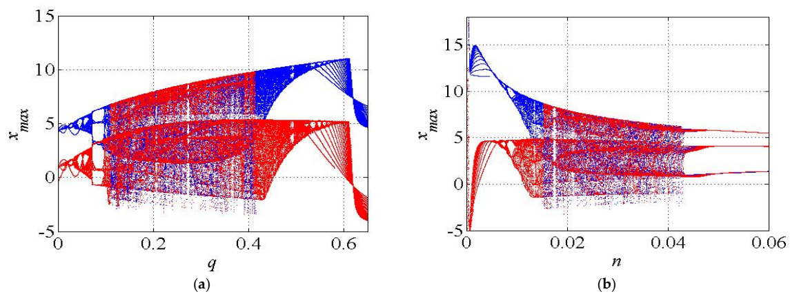
Figure 13. Multistability analysis in the proposed 3-D chaotic financial firm system (a,b) The bifurcation diagram with the distinct initial conditions (0.03, 0.03, 0.03), shown in blue branch and (−0.03, −0.03, −0.03), shown in red branch.
