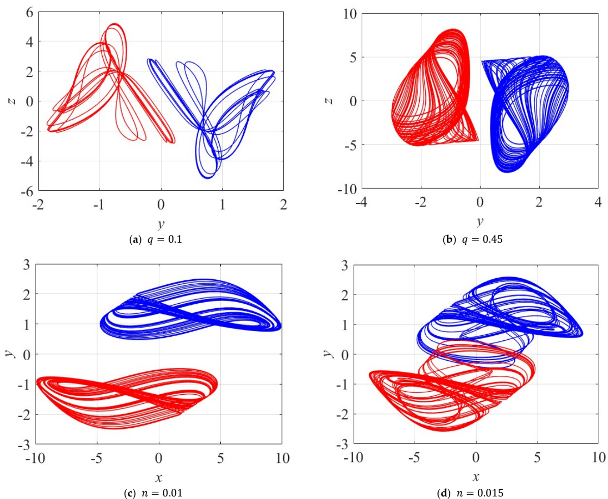
Figure 14. The coexisting attractors of the system with different initial conditions (0.03, 0.03, 0.03) (blue) and (−0.03, −0.03, −0.03) (red). (a) Periodic coexisting attractors at q = 0.1 , (b) chaotic coexisting attractors at q = 0.45 , (c) one scroll coexisting attractors at n = 0.01 , and (d) two scroll coexisting attractors at n = 0.015 .
