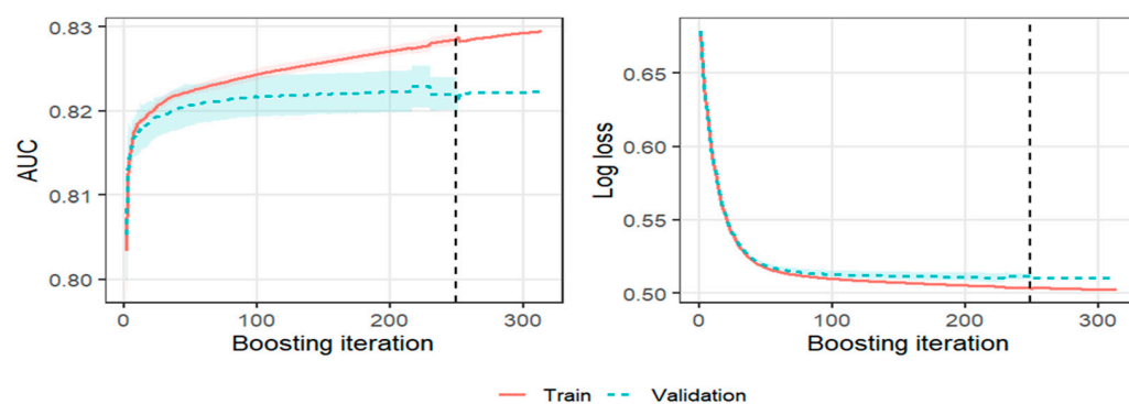
Figure A3. Training and validation learning curves for the selected CatBoost model. The vertical black dashed line indicates the number of boosting iterations selected by early stopping. The shaded area represents variability across the validation folds.
