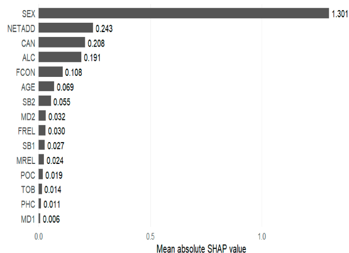
Figure 3. Global predictor importance based on mean absolute SHAP values for the CatBoost model of adolescent pornography use.
