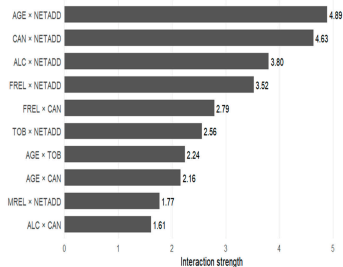
Figure 4. Ten strongest feature interactions identified by the CatBoost model.
