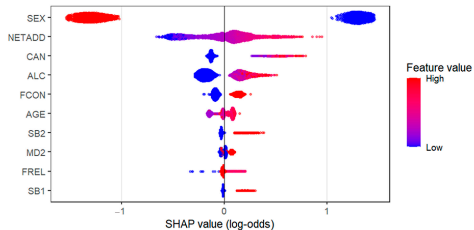
Figure 2. Beeswarm of SHAP values estimated with CatBoost.
