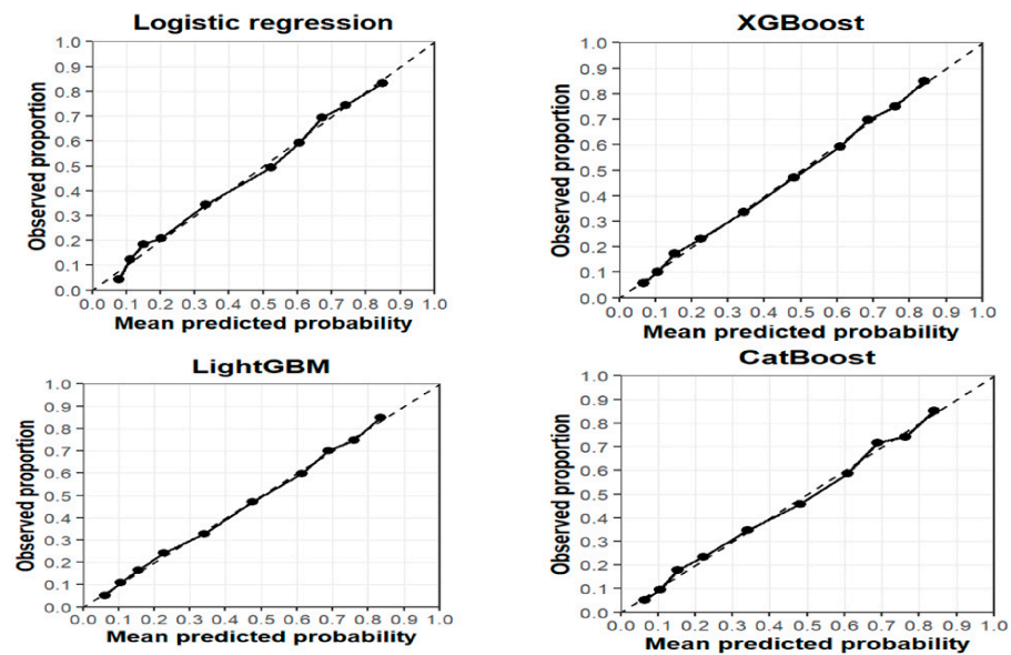
Figure A4. Calibration curves for the four predictive models in the independent test sample.
