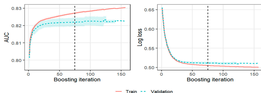
Figure A1. Training and validation learning curves for the selected XGBoost model. The vertical black dashed line indicates the number of boosting iterations selected by early stopping. The shaded area represents variability across the validation folds.
