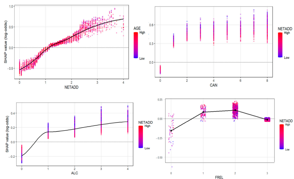
Figure 5. SHAP dependence plots for the four strongest feature interactions in the CatBoost model.
