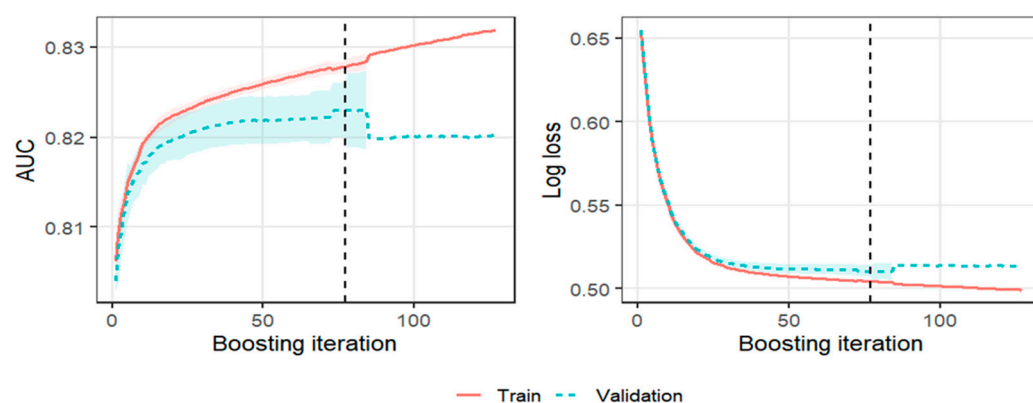
Figure A2. Training and validation learning curves for the selected LightGBM model. The vertical black dashed line indicates the number of boosting iterations selected by early stopping. The shaded area represents variability across the validation folds.
