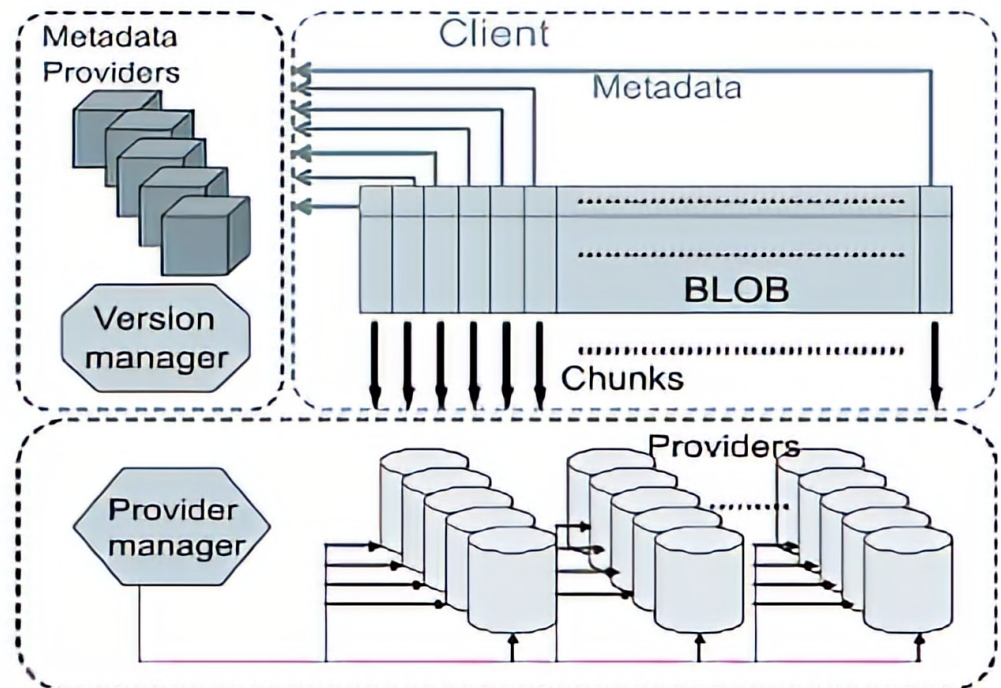
Figure 1. Framework of BlobSeer distributed file system (DFS) [26].
