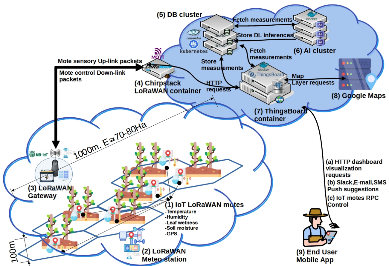
Figure 1. Proposed thingsAI high-level system architecture.
