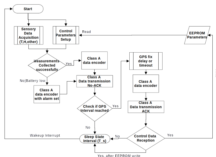
Figure 3. LoRaWAN class A data transmission process of mote devices and meteorological stations.
