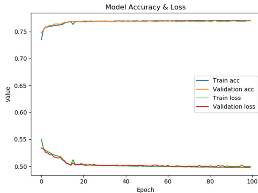
Figure 9. The performance of the model for the optimization of time slot scheduling.
