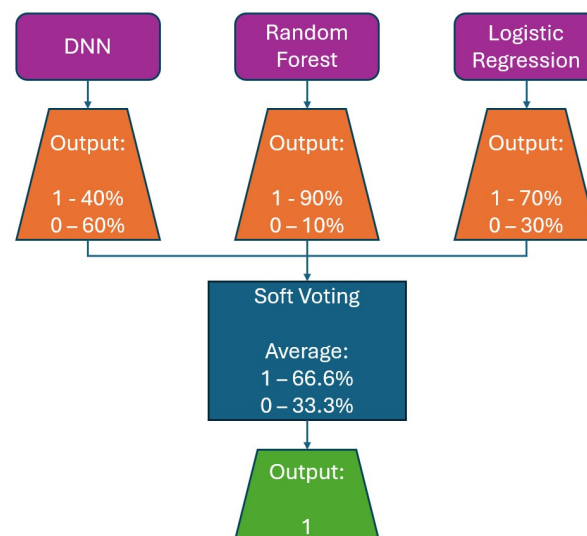
Figure 15. Example for soft voting ensemble of DNN, Random Forest, and logistic regression classifiers.
