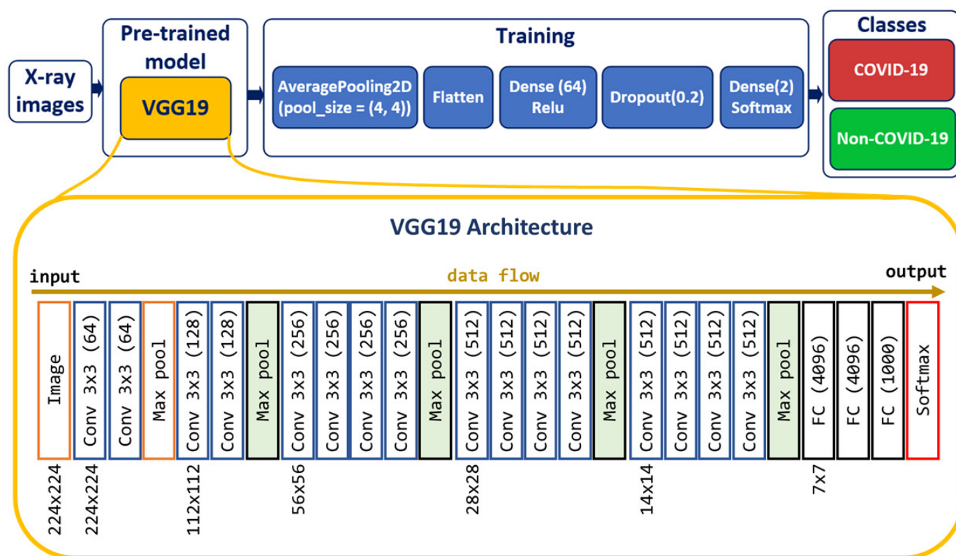
Figure 2. Model for predicting COVID-19 and non-COVID-19 cases.
