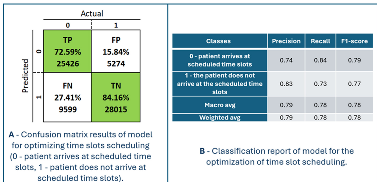
Figure 10. Confusion matrix results and classification report of the model for optimizing time slots scheduling (0—patient arrives at scheduled time slots, 1—patient does not arrive at scheduled time slots).
