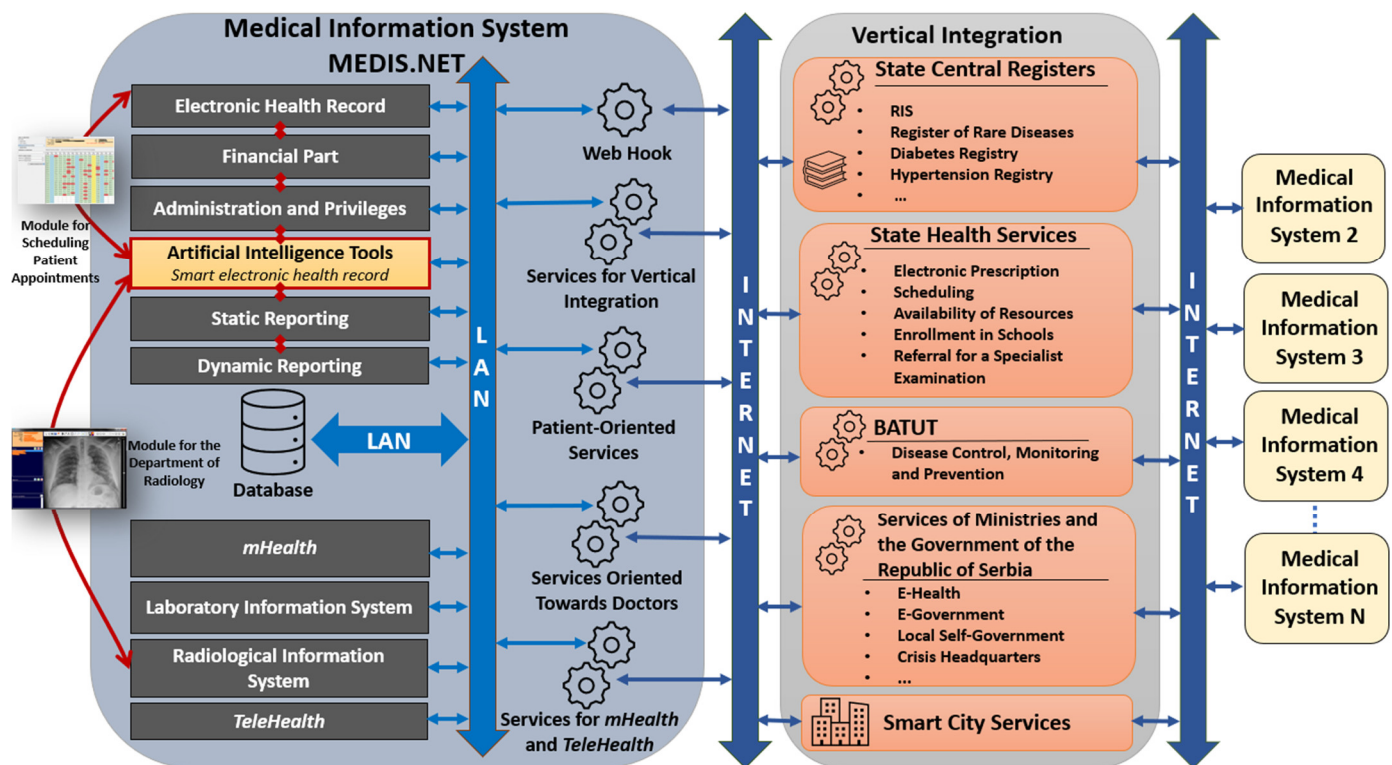
Figure 16. Architecture of MIS MEDIS.NET and position of artificial intelligence tools.
