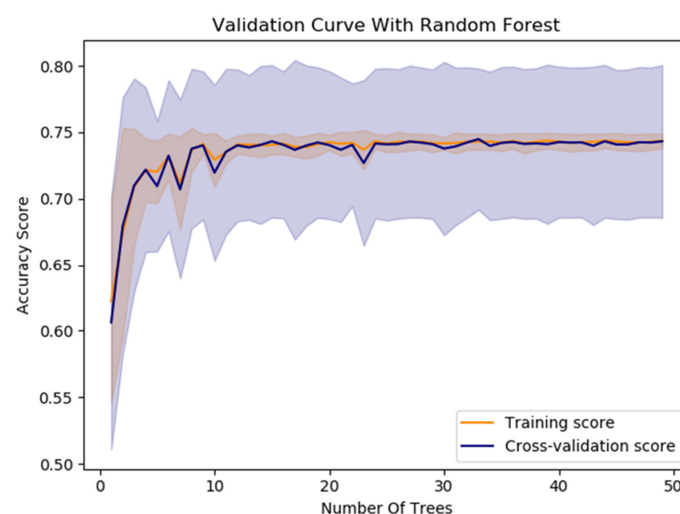
Figure 14. The Random Forest model's performance for optimizing time slot scheduling.
