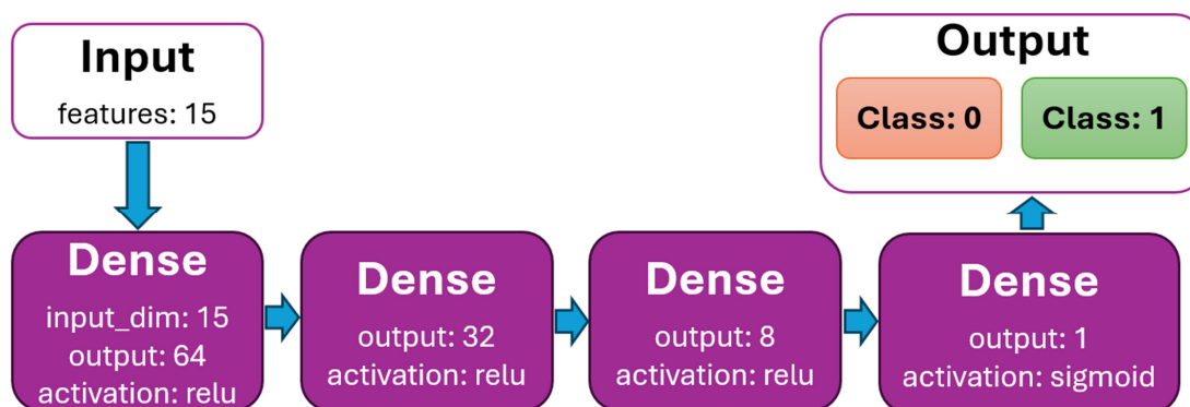
Figure 6. DNN model graph with dense layers.
