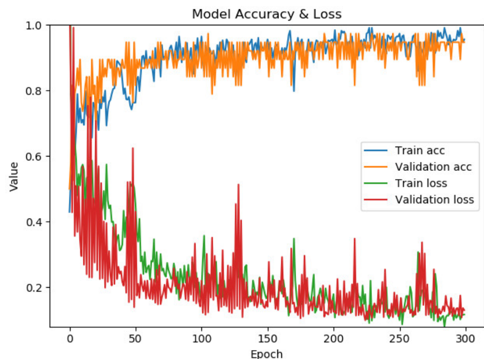
Figure 7. The performance of the model for chest X-ray image classification.
