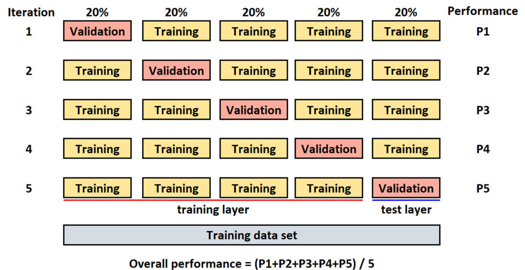
Figure 3. K-fold cross-validation for k = 5.
