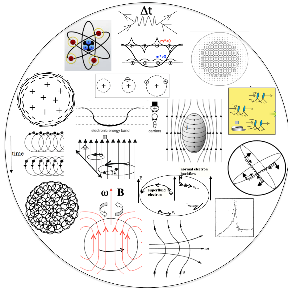
Figure 1. Schematic pictorial depiction of the principal elements of the theory of hole superconductivity.
