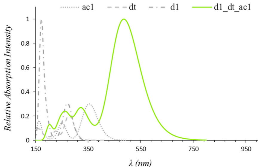
Figure 8. Comparison between the TD-CAM-B3LYP/6-311G//B3LYP/6-311G computed electron absorption spectra of d1_dt_ac1 , d1 , dt and ac1 . The spectra are reported normalized with respect to the highest absorption band of d1_dt_ac1 in order to highlight the absorption changes upon formation of the complete D- \pi -A chromophore.
