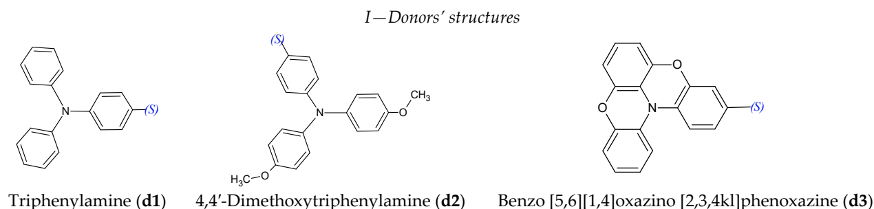
Figure 1. Sketch of the molecular structures of the donor groups with their name and acronym used for identification in parenthesis. The symbol (S) represents the binding site in the push–pull system.
