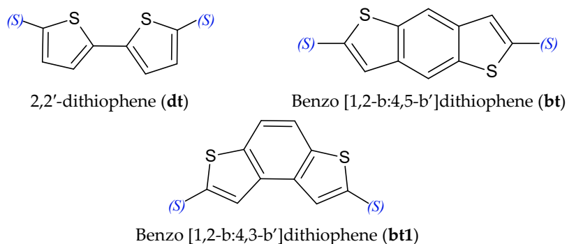
Figure 2. Sketch of the molecular structures of the \pi -bridges with their name and acronym used for identification in parenthesis. The symbol (S) represents the binding site in the push–pull system.
