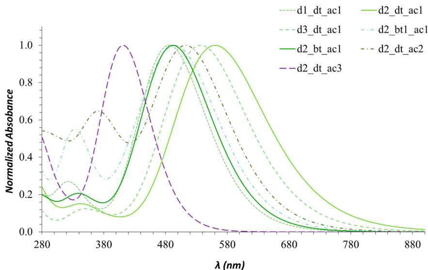
Figure 9. Comparison between the simulated absorption spectra of the D_dt_ac1 , d2_π_ac1 and d2_dt_A chromophores obtained at TD-CAM-B3LYP/6-311G level. Calculations were performed on the optimized B3LYP/6-311G geometry.
