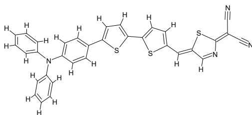
Scheme 1. Molecular structure of d1_dt_ac1 as an example of a D– \pi –A system according to the acronym notation (D = d1 , = dt and A = ac1 ).
