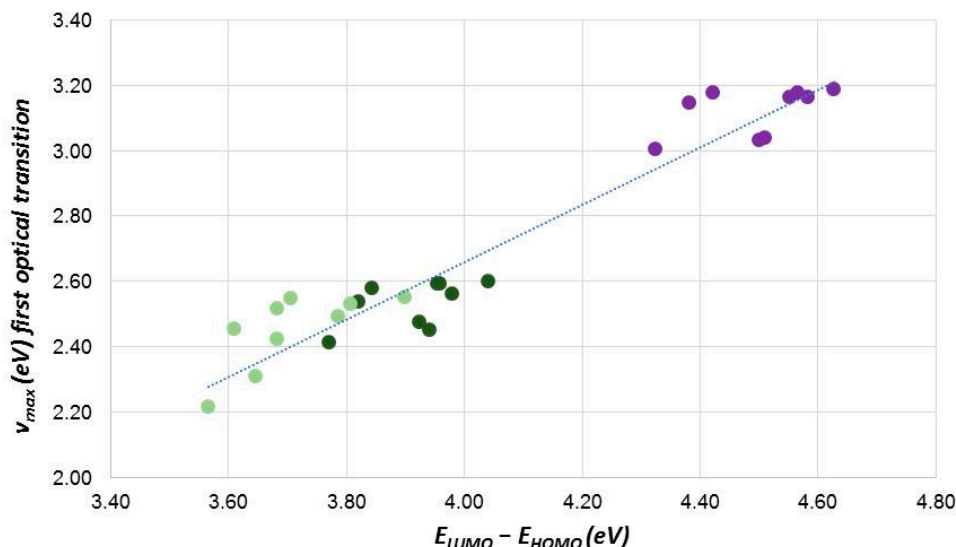
Figure 7. Plot of the first optical transitions frequencies \nu_{max} , in eV, versus the HOMO–LUMO energy gap ( E_{LUMO} - E_{HOMO} , eV) for the D– \pi –A systems. The chromophores with the ac3 , ac2 and ac1 donors are depicted as violet, dark green and green dots, respectively. Calculations were performed at the TD–CAM–B3LYP/6–311G //B3LYP/6–311G level.
