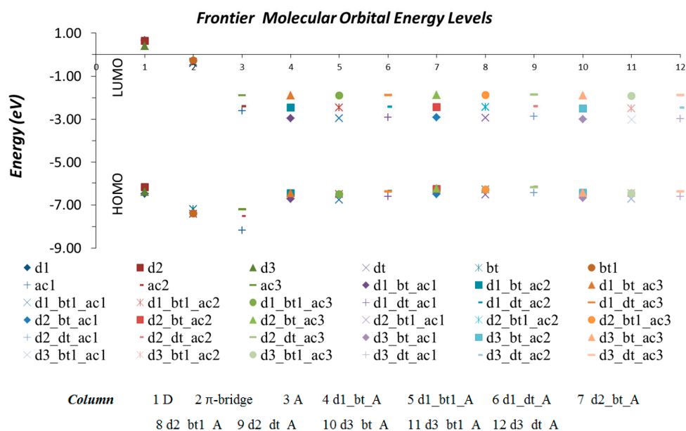
Figure 4. Comparison of the TD-CAM-B3LYP/6-311G HOMO and LUMO energies of the different molecules studied here. The first three columns refer to the single building moieties.
