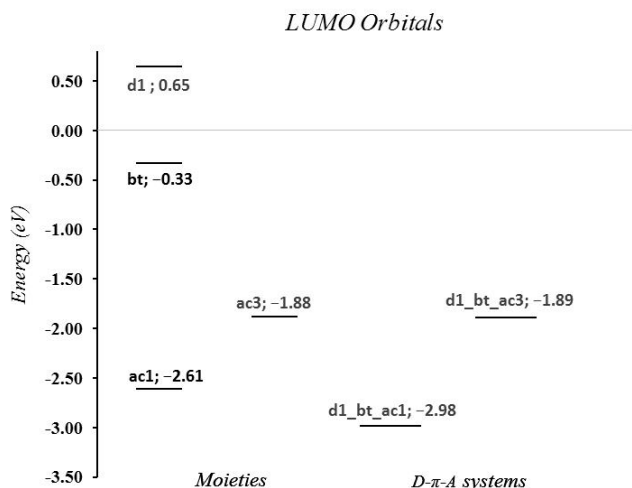
Figure 5. Fragment-orbital interaction diagram for the representative chromophores d1_bt_ac3 and d1_bt_ac1 . The HOMO (top) and LUMO (bottom) energies of the D- \pi -A chromophores are compared with those of the donor ( d1 ), \pi -bridge ( bt ), and acceptor ( ac1 or ac3 ) fragments.
