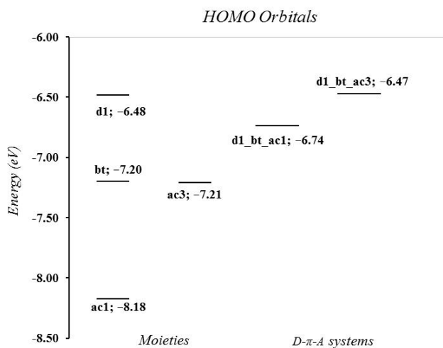
Figure 4. Comparison of the TD-CAM-B3LYP/6-311G HOMO and LUMO energies of the different molecules studied here. The first three columns refer to the single building moieties.
