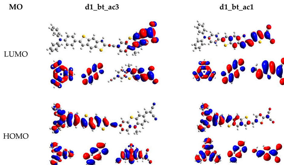
Figure 6. Sketch of the TD-CAM-B3LYP/6-311G HOMO and LUMO isodensity ( 0.02 \text{ e/a}_0^3 ) for d1_bt_ac3 (left) and d1_bt_ac1 (right). In each panel, the chromophore MOs (top) are compared with those of the corresponding moieties (bottom). For the acronyms, refer to Figures 1–3.
