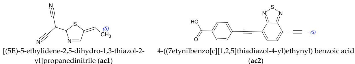
Figure 2. Sketch of the molecular structures of the \pi -bridges with their name and acronym used for identification in parenthesis. The symbol (S) represents the binding site in the push–pull system.
