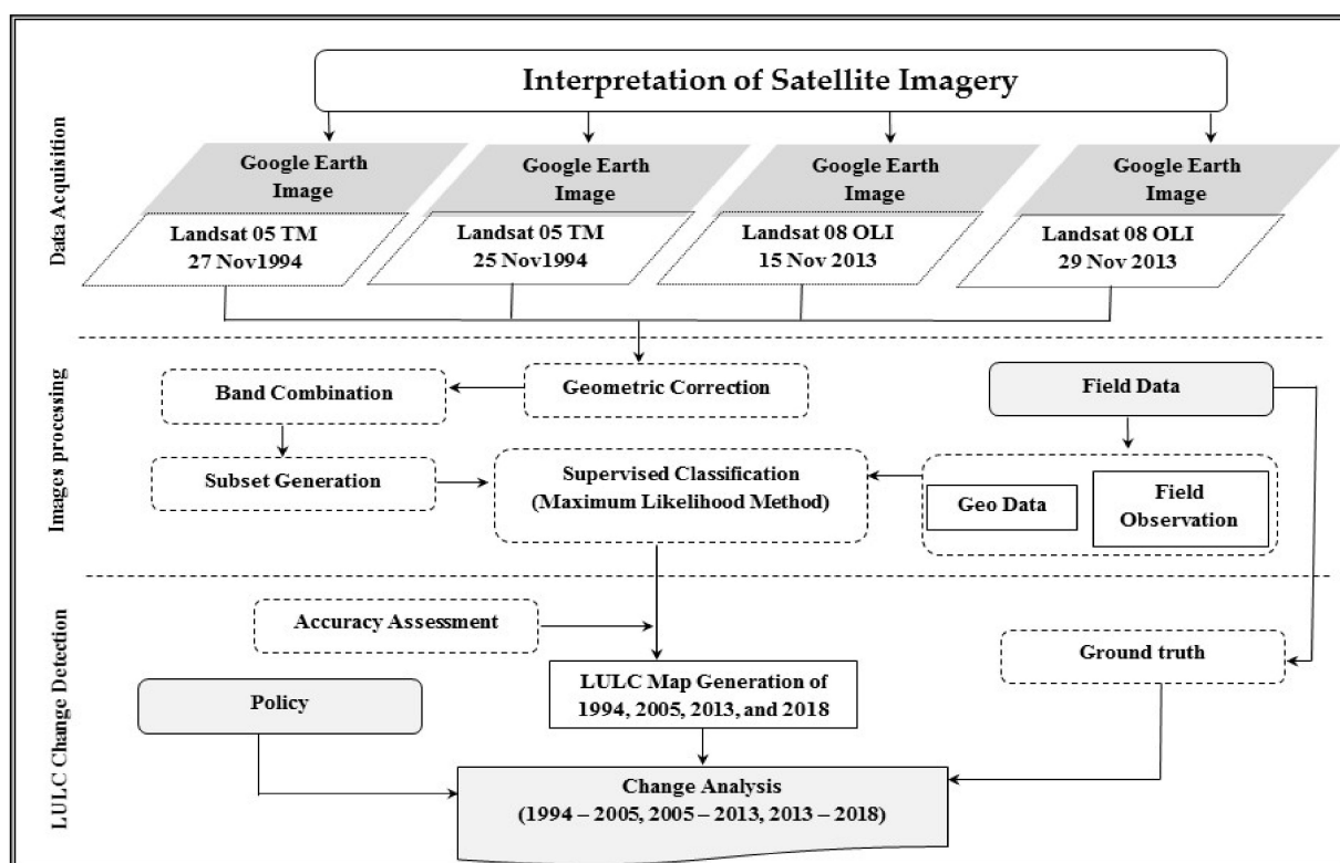
Figure 3. General methodological flowcharts: data acquisition, land use and land cover (LULC) analysis, and trends in forest land use changes in RKWS, Bangladesh.
