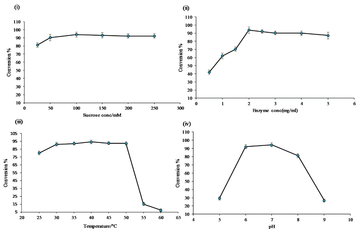
Figure 3. Conversion percentage of resveratrol to resveratrol glucosides in the optimization cascade reaction; (i) variation of sucrose concentration; (ii) different enzymes concentration of DgAS; (iii) variation of reaction temperature; and (iv) variation of buffer and pH.
