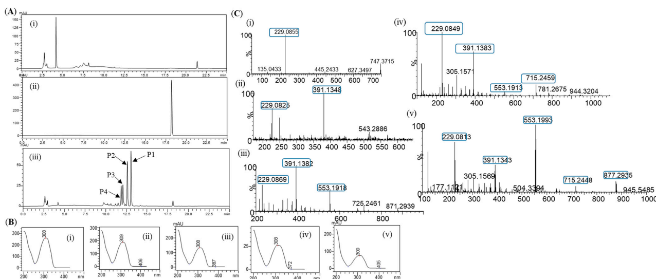
Figure 2. (A) HPLC analysis of resveratrol reaction mixture: (i) control reaction for regular glycosylation reaction of DgAS; (ii) standard resveratrol; and (iii) regular glycosylation reaction carried out using DgAS. (B) UV-VIS analysis of each major peak from HPLC: (i) standard resveratrol; (ii) P1; (iii) P2; (iv) P3; and (v) P4. (C) HRQTOF-ESI/MS analysis of (i) resveratrol standard; (ii) product P1; (iii) product P2; (iv) product P3; and (v) product P4.
