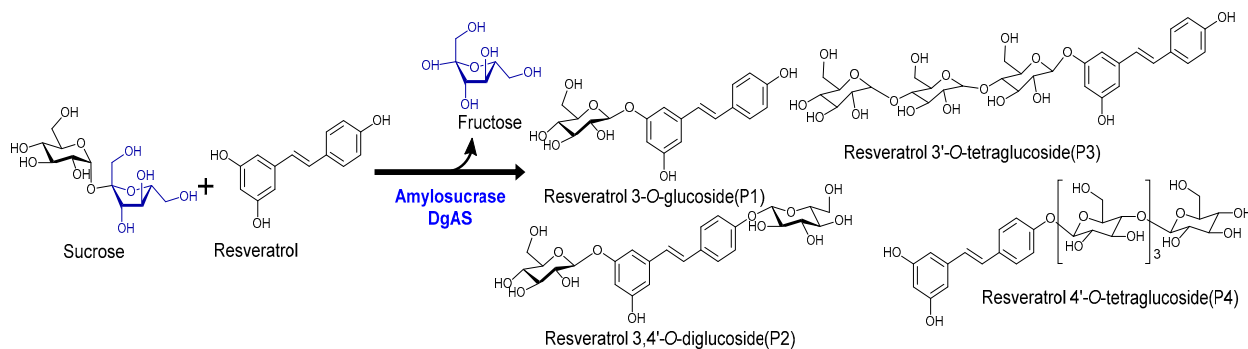
Figure 1. Representative reaction scheme of resveratrol glucoside formation by the enzyme DgAS, amylosucrase.
