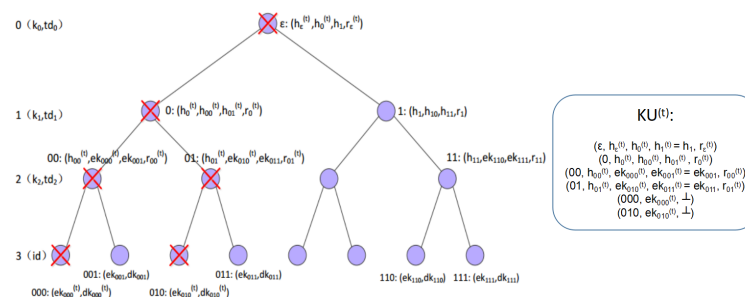
Figure 5. The illustration of KU^{(t)} when users “000” and “010” have been revoked at time slot t .
