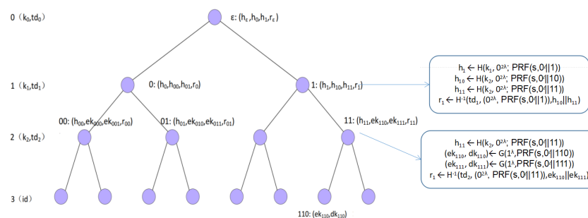
Figure 4. The illustration of Private Key Generation for user “110”. The private key sk_{110} of user “110” collects all the node values along the path from “110” to “ \epsilon ” in the tree.
