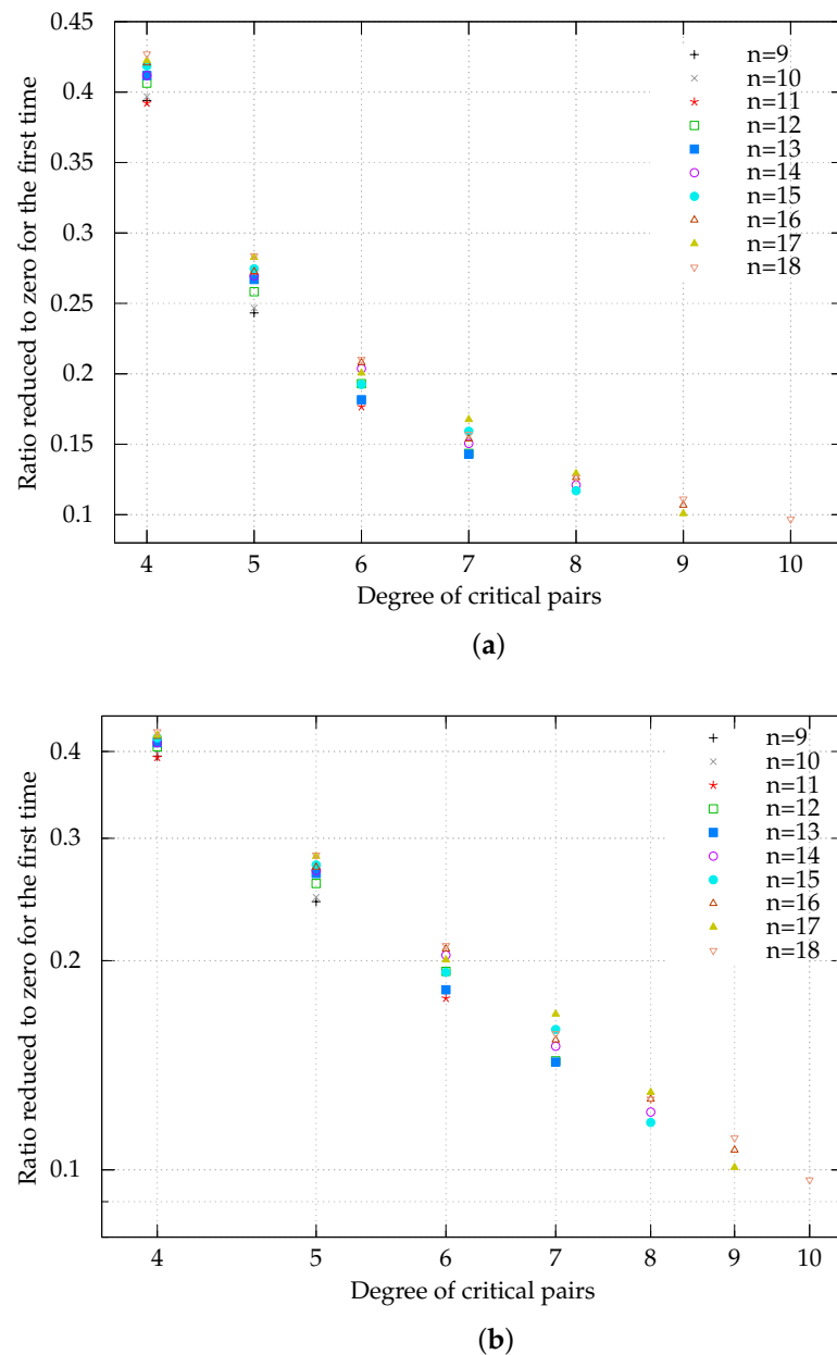
Figure 4. Benchmark results for m = n + 1 over \mathbb{F}_{256} . (a) Experimental results of the ratio of critical pairs for a reduction to zero in the first half over \mathbb{F}_{256} and \mathbb{F}_{31} for m = n + 1 . (b) \log_{10} - \log_{10} graph of the ratio of critical pairs for a reduction to zero in the first half over \mathbb{F}_{256} and \mathbb{F}_{31} for m = n + 1 .
