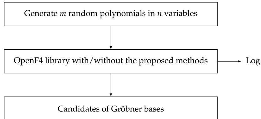
Figure 1. Software architecture of our system.
