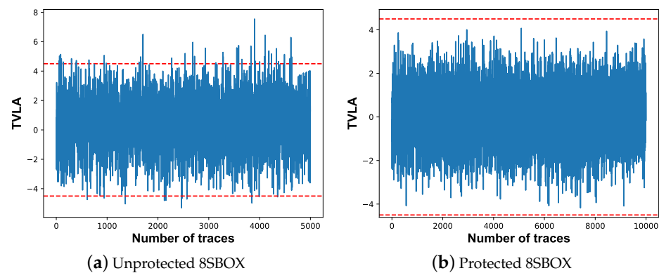
Figure 16. TVLA analysis.
