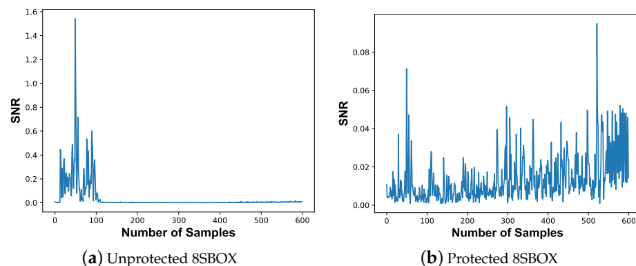
Figure 15. SNR analysis.
