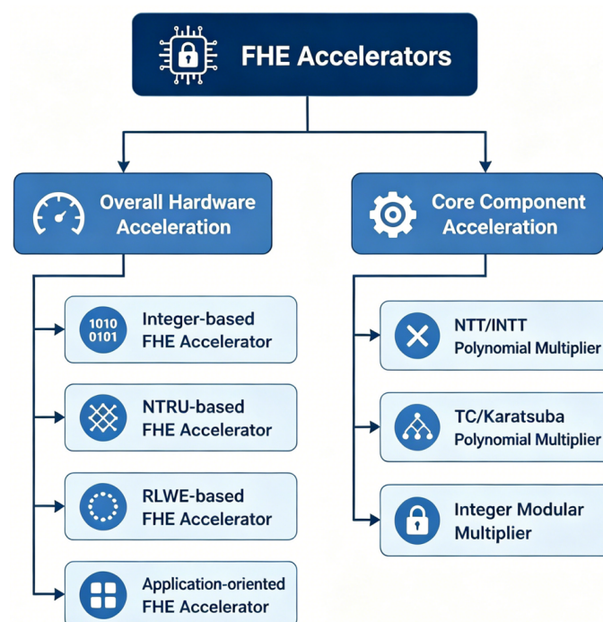
Figure 2. Classification Framework of FHE Hardware Architectures.
