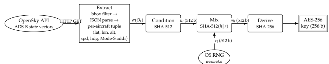
Figure 2. Pipeline A: from ADS-B aircraft state vectors to a 256-bit AES-256 key. The Extract stage reduces a regional snapshot of the OpenSky live feed to a serialised byte string; the remaining three stages instantiate the framework with SHA-512 conditioning, a SHA-512-based combiner mixing in OS-RNG bytes, and a SHA-256 derive step. Source: authors' own work.
