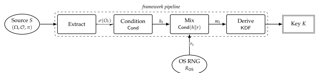
Figure 1. The framework: a four-stage construction that combines an environmental source S with the operating-system generator R_{OS} to produce a cryptographic key K . The dashed rectangle encloses the four framework stages; S supplies the extracted observation stream and R_{OS} supplies the independent randomness mixed in at the third stage. Source: authors' own work.
