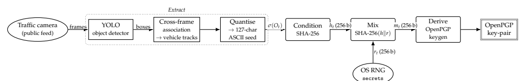
Figure 4. Pipeline C: from a public traffic-camera feed to an OpenPGP key-pair. The Extract stage chains a YOLO object detector, a cross-frame association step that produces persistent vehicle tracks, and a quantisation step that emits a fixed-length ASCII seed. SHA-256 is used throughout the conditioning, mixing, and derivation stages, and the derived passphrase seeds an OpenPGP key generation routine conformant with RFC 9580. Source: authors' own work.
