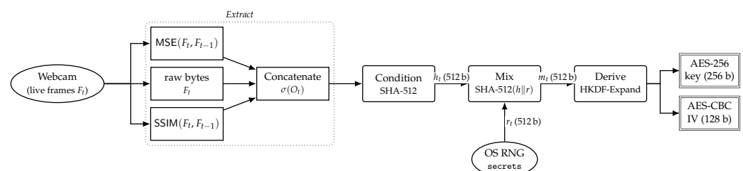
Figure 3. Pipeline B: from a webcam observing a chaotic physical process to an AES-256 key plus initialisation vector for AES-CBC encryption. The Extract stage produces three parallel descriptors of the current frame—raw bytes, mean squared error against the previous frame, and the structural similarity index—which are concatenated before SHA-512 conditioning. The Derive stage uses HKDF-Expand with two distinct info labels (‘aes-256-key’ and ‘aes-cbc-iv’) to obtain the key and the initialisation vector as domain-separated outputs of the mixed value, in place of the earlier truncate-the-same-digest derivation. Source: authors’ own work.
