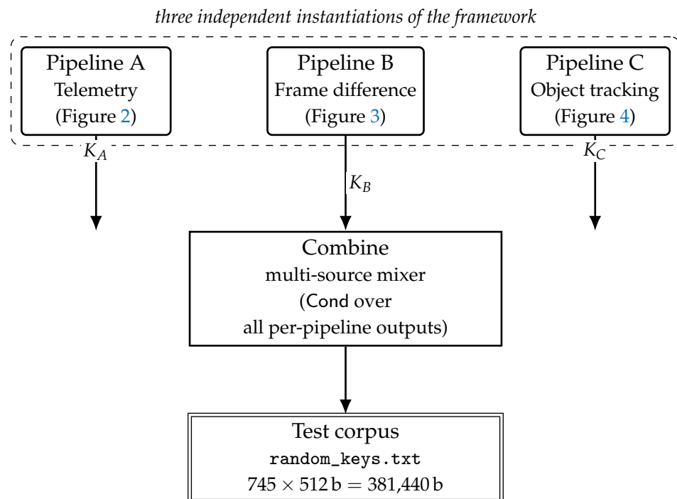
Figure 6. How the three pipelines are combined into the empirical corpus tested in this section. Each pipeline runs the framework (Figures 2–4) and emits a derived key; the three per-pipeline keys are then passed through a multi-source mixer that re-applies the framework's conditioning function Cond over the concatenation of its inputs, and the resulting output stream is partitioned into 64-byte test units. The corpus random_keys.txt contains 745 such units used in Tables 3 and 4. Source: authors' own work.
