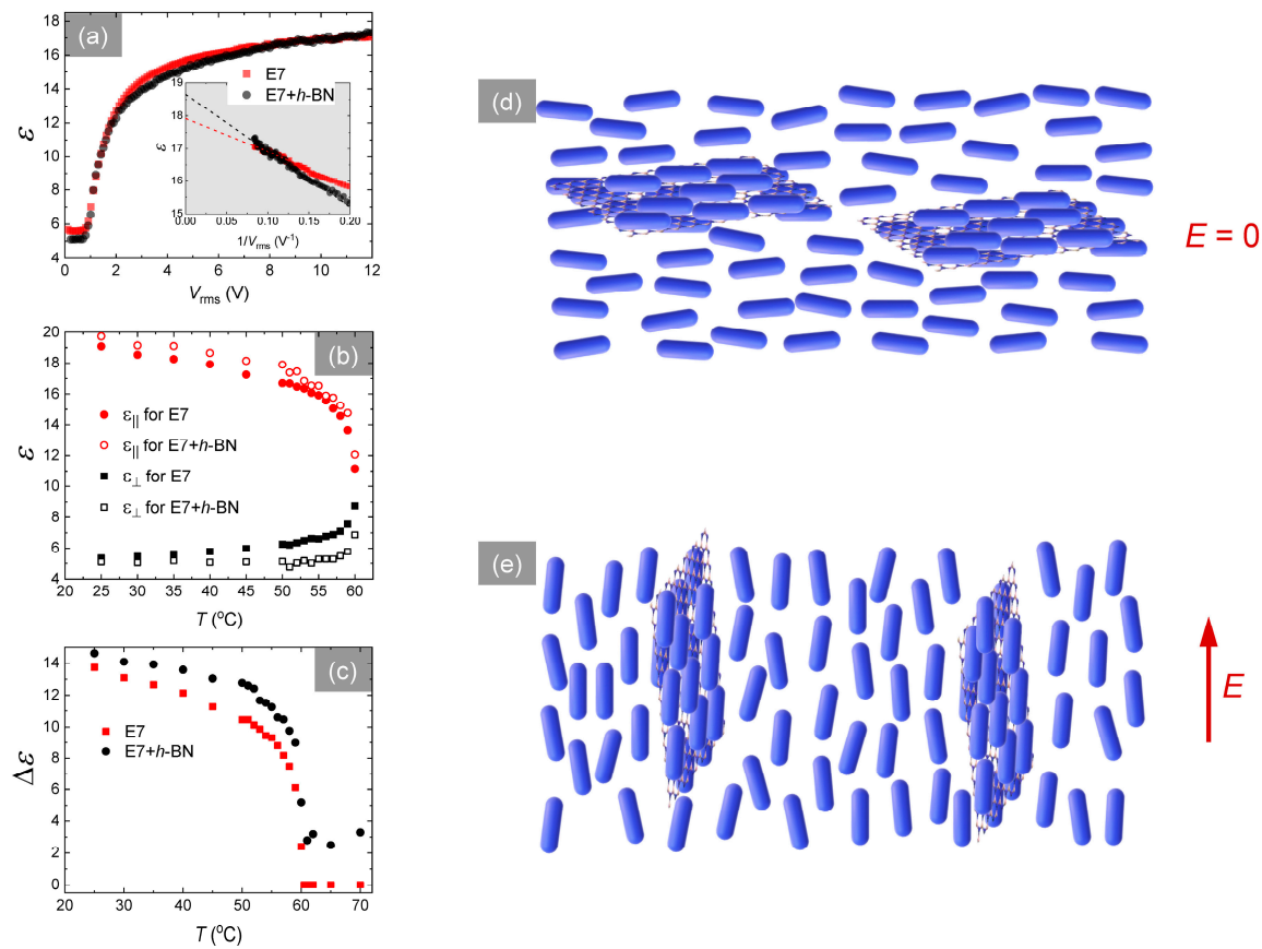
Figure 2. (a) Dielectric constant \epsilon as a function of applied RMS voltage ( f = 1000 Hz) in the nematic phase ( T = 40 °C) for the pure LC and LC+h-BN listed in the legend. (b) Dielectric components, \epsilon_{\perp} and \epsilon_{||} as a function of temperature for the pure LC and LC+h-BN listed in the legend. (c) Dielectric anisotropy \Delta\epsilon as a function of temperature for the pure LC and LC+h-BN listed in the legend. (d) A schematic illustration of the presence of PNDs in the nematic phase. (e) A schematic illustration of the reorientation of the PNDs with the nematic director in the application of an electric field \vec{E} .
