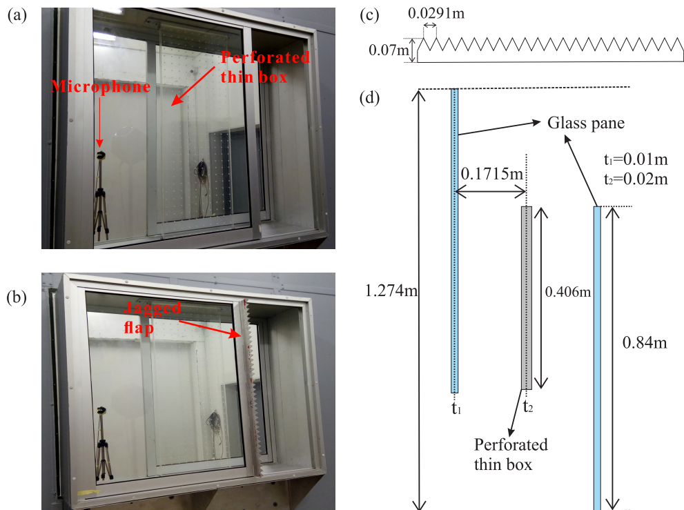
Figure 1. (a) Experimental set-up of the plenum window with perforated thin box at reverberation room. (b) Plenum window with attached 90^\circ jagged flap. (c) Geometry of the jagged flap. (d) Schematic diagram of the experiment set up (top view, t = thickness, detailed geometry of the perforated thin box is shown in Figure 2).
