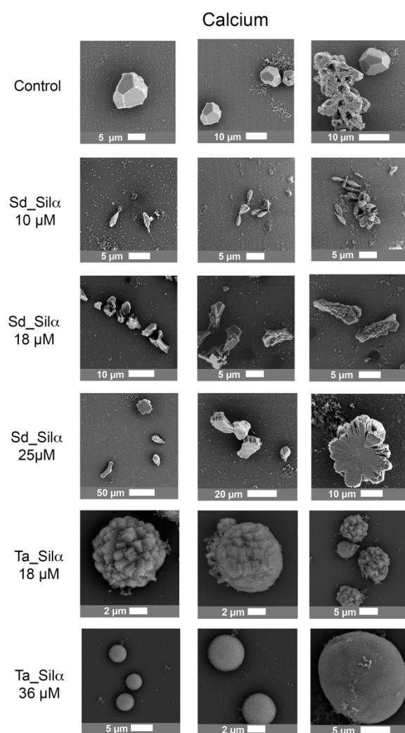
Figure 3. Selection of SEM micrographs from calcium silica carbonate biomorphs obtained at 25 °C in the presence of different concentrations of silicatein- \alpha . Sd_Sil \alpha — Suberitis domuncula silicatein- \alpha , Ta_Sil \alpha — Tethya aurantia silicatein- \alpha .
