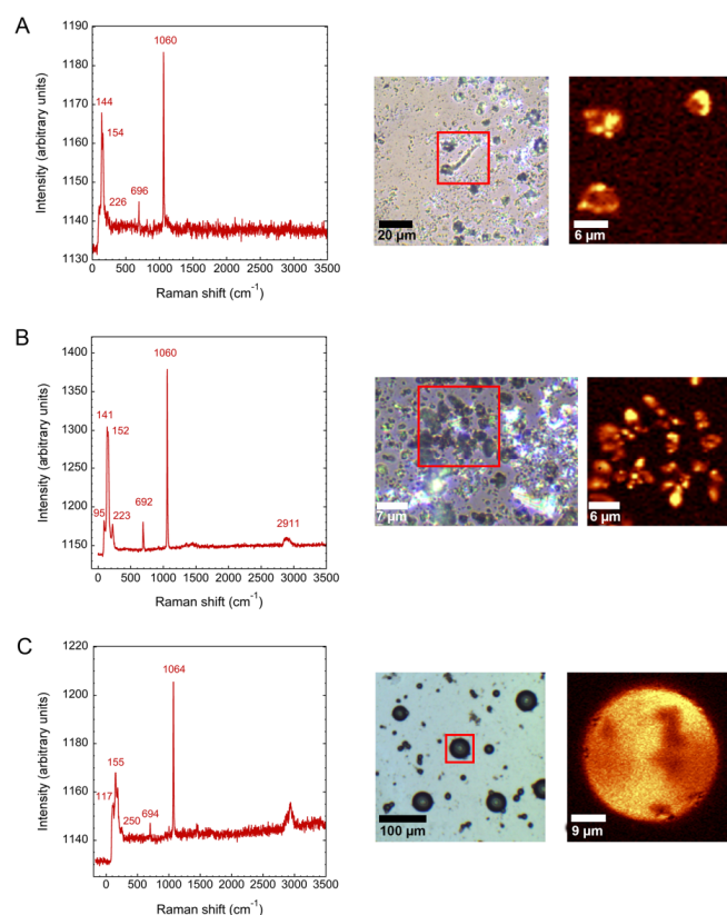
Figure 7. Raman spectroscopic analysis of witherite silica carbonate biomorphs obtained in different conditions. (A) Control in the absence of enzyme. (B) Suberitis domuncula silicatein- \alpha . (C) Tethya aurantia silicatein- \alpha . Left panels correspond to the Raman spectra. Right panels correspond to the optical image and mapping at the most intense Raman signal.
