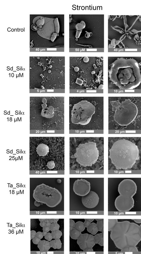
Figure 6. Selection of SEM micrographs from strontium silica carbonate biomorphs obtained at 25 °C in the presence of different concentrations of silicatein- \alpha . Sd_Sil \alpha — Suberitis domuncula silicatein- \alpha , Ta_Sil \alpha — Tethya aurantia silicatein- \alpha .
