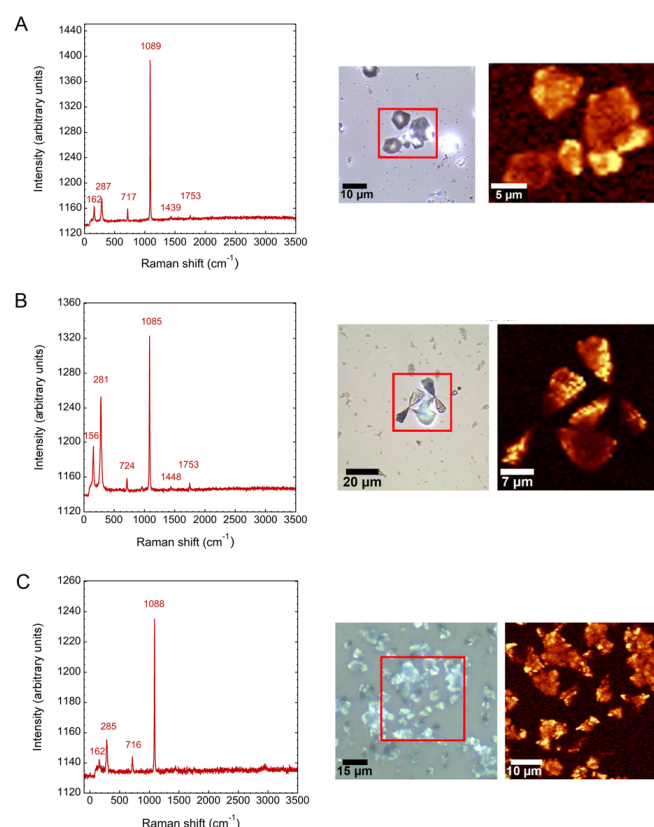
Figure 4. Raman spectroscopic analysis of calcite silica carbonate biomorphs obtained in different conditions. (A) Control in the absence of enzyme. (B) Suberitis domuncula silicatein- \alpha . (C) Tethya aurantia silicatein- \alpha . Left panels correspond to the Raman spectra. Right panels correspond to the optical image and mapping at the most intense Raman signal.
