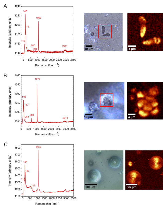
Figure 8. Raman spectroscopic analysis of strontianite silica carbonate biomorphs obtained in different conditions. (A) Control in the absence of enzyme. (B) Suberitis domuncula silicatein- \alpha . (C) Tethya aurantia silicatein- \alpha . Left panels correspond to the Raman spectra. Right panels correspond to the optical image and mapping at the most intense Raman signal.
