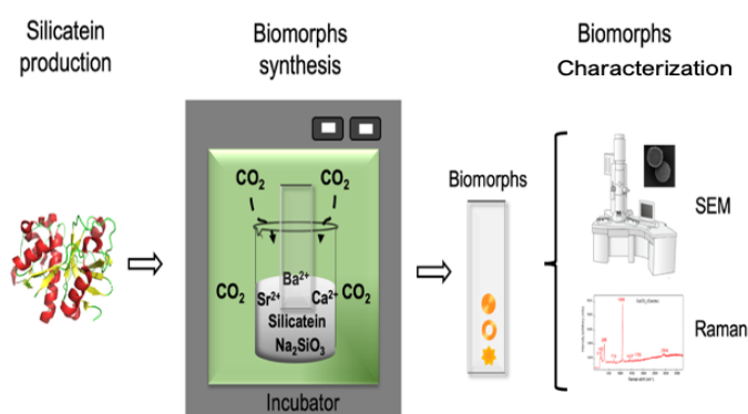
Figure 1. Schematic representation of the procedure involved in the synthesis of silica carbonate biomorphs in solution using a gas-diffusion system. The structure of the T. aurantia silicatein- \alpha corresponds to that deposited in the Protein Data Bank code 6zq3.
