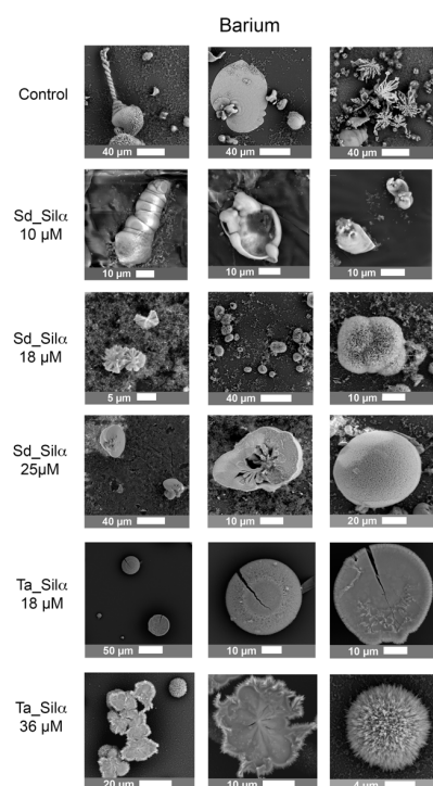
Figure 5. Selection of SEM micrographs from barium silica carbonate biomorphs obtained at 25 °C in the presence of different concentrations of silicatein- \alpha . Sd_Sil \alpha — Suberitis domuncula silicatein- \alpha , Ta_Sil \alpha — Tethya aurantia silicatein- \alpha .
