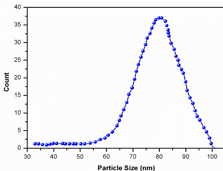
Figure 3. Histogram of ZnO particle size distribution.
