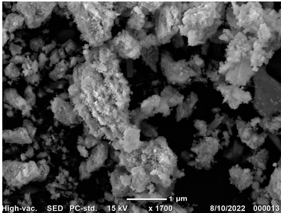
Figure 5. FESEM picture of zinc oxide NPs synthesized via the green route.
