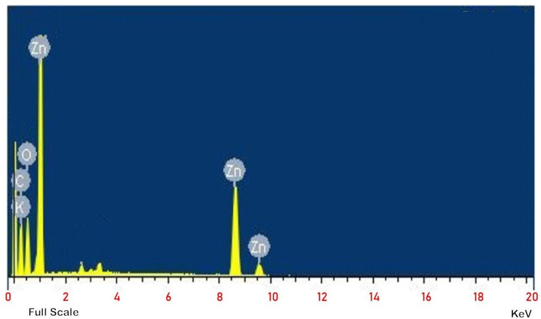
Figure 6. EDAX pattern for the green synthesized ZnO-NPs (Zn—zinc, O—oxygen, and C—carbon).
