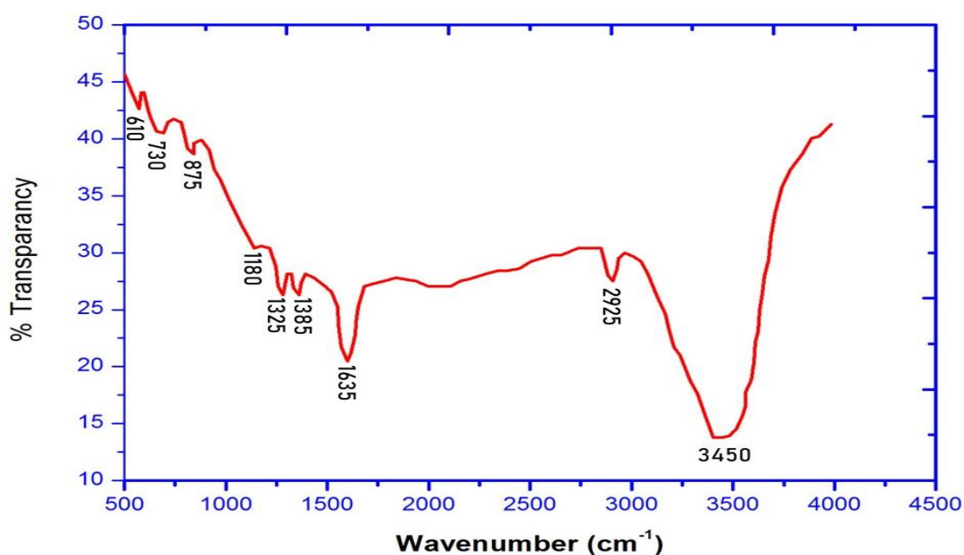
Figure 7. FTIR spectrum of ZnO-NPs.
